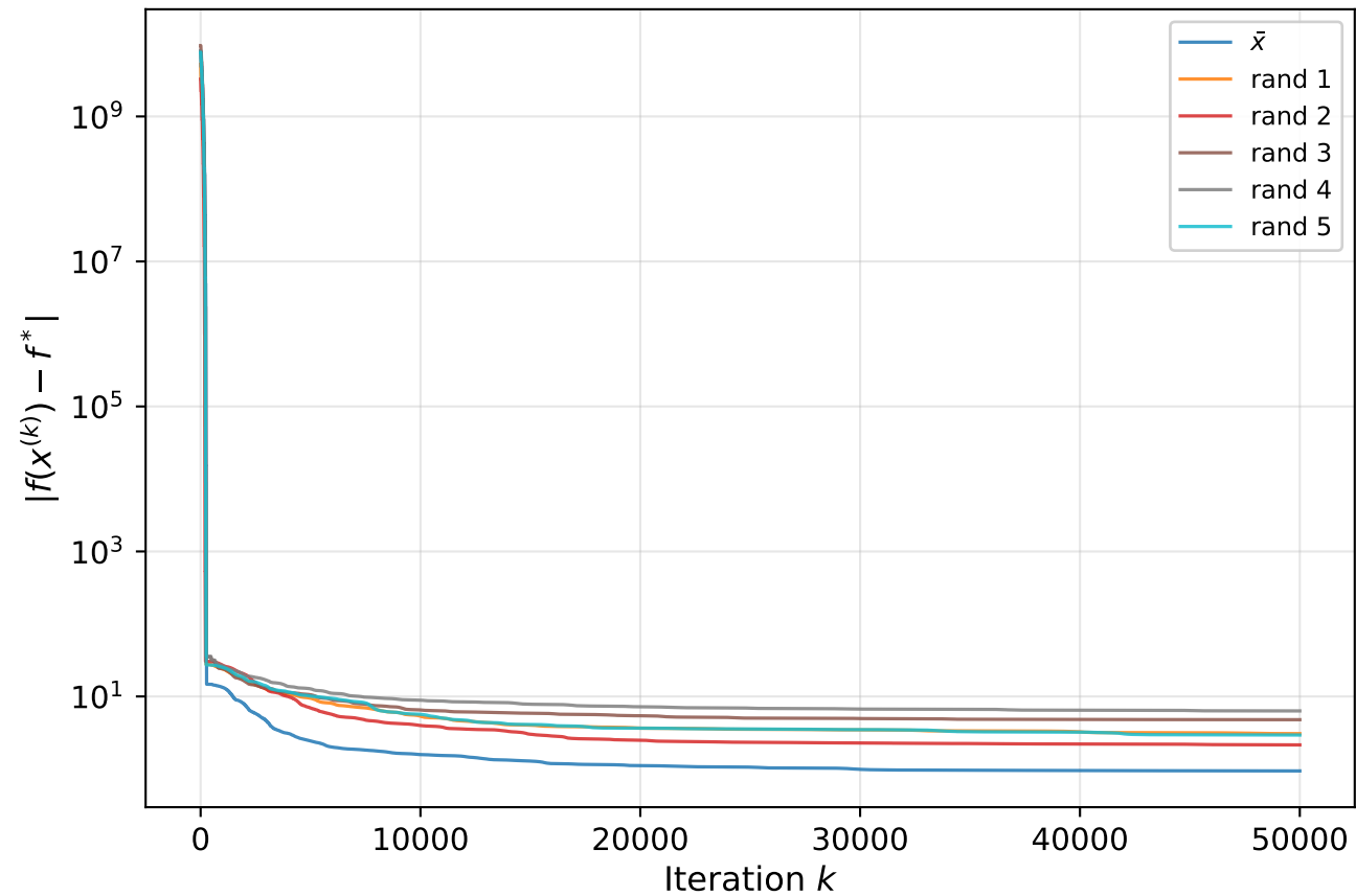
Zakharov — convergence ( n = 50 )
