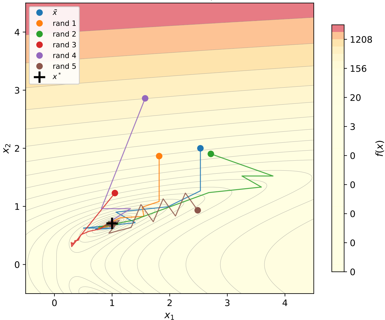
Dixon-Price — Nelder-Mead paths ( n = 2 )
