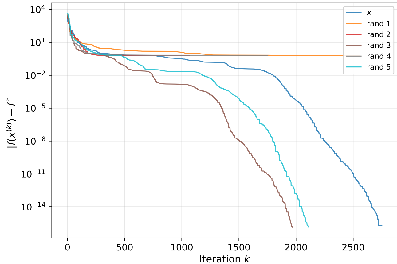
Dixon-Price — convergence ( n = 10 )
