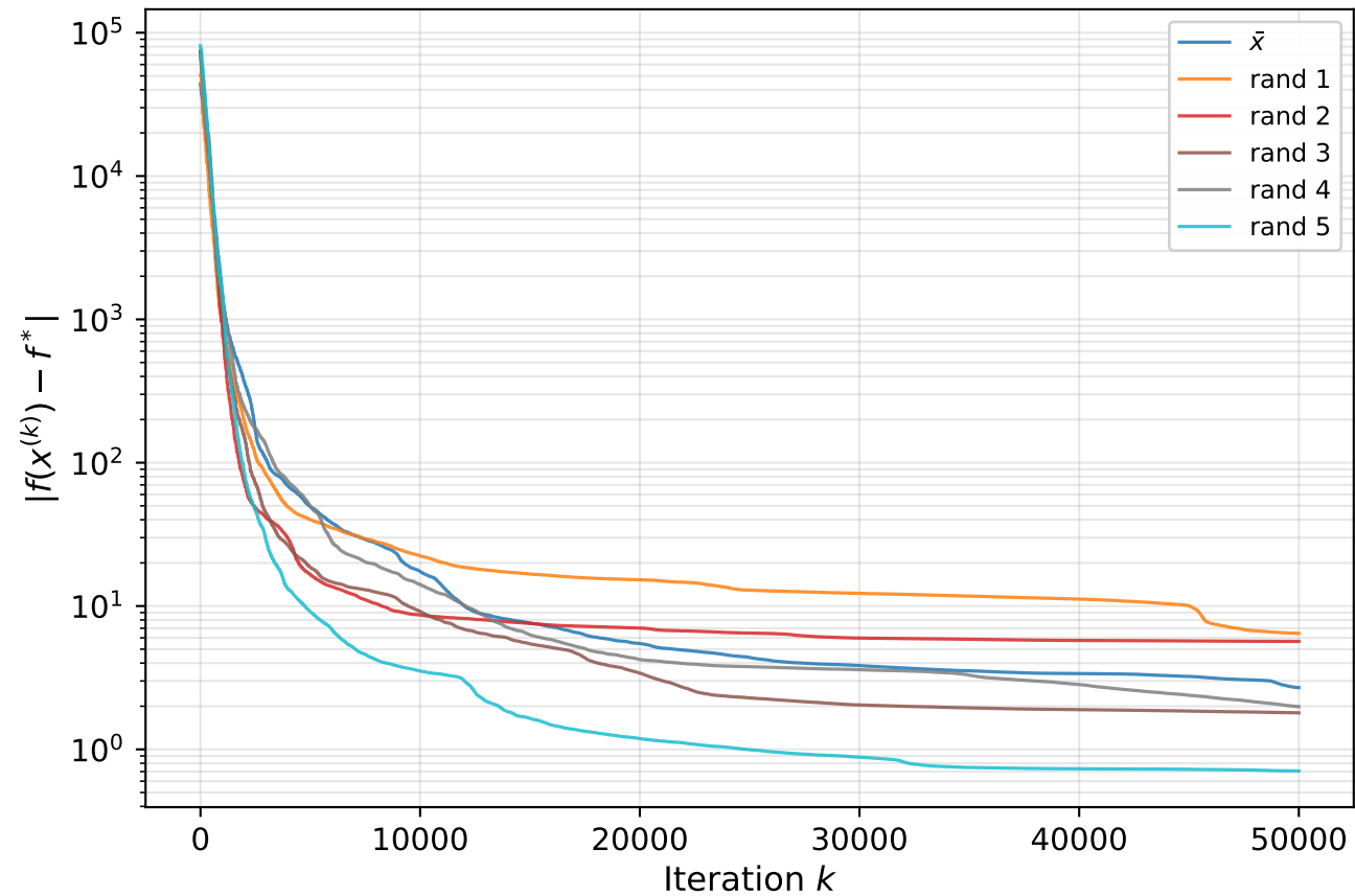
Dixon-Price — convergence ( n = 50 )
