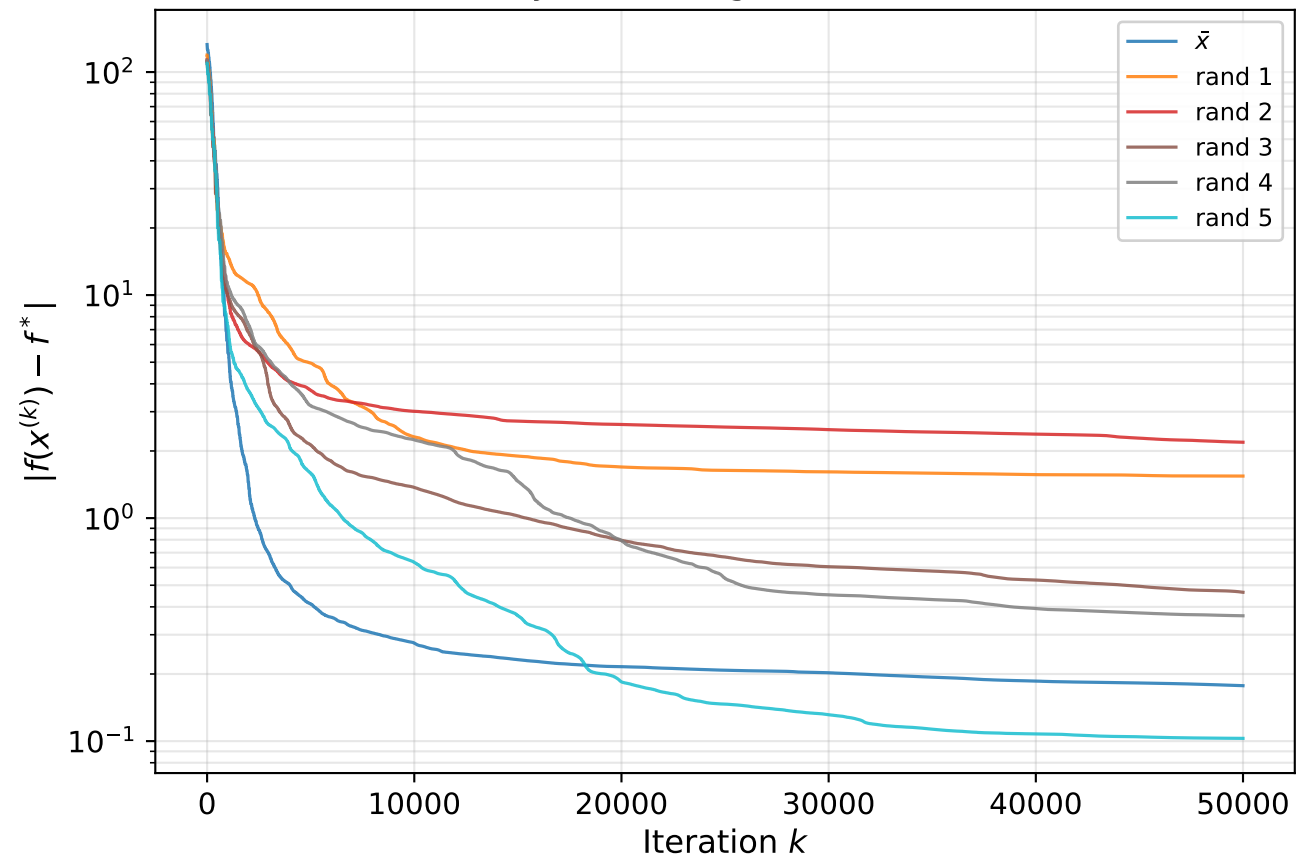
Levy — convergence ( n = 50 )
