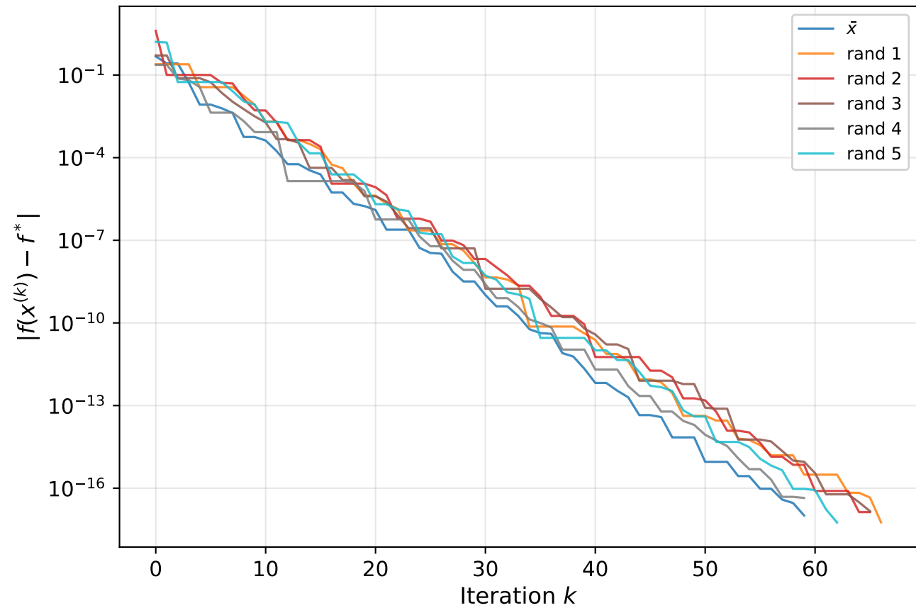
Zakharov — convergence ( n = 2 )
