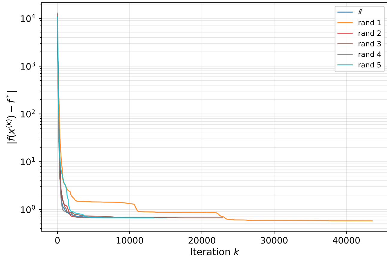
Dixon-Price — convergence ( n = 20 )
