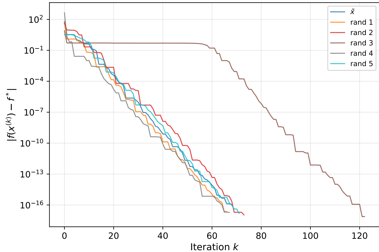
Dixon-Price — convergence ( n = 2 )
