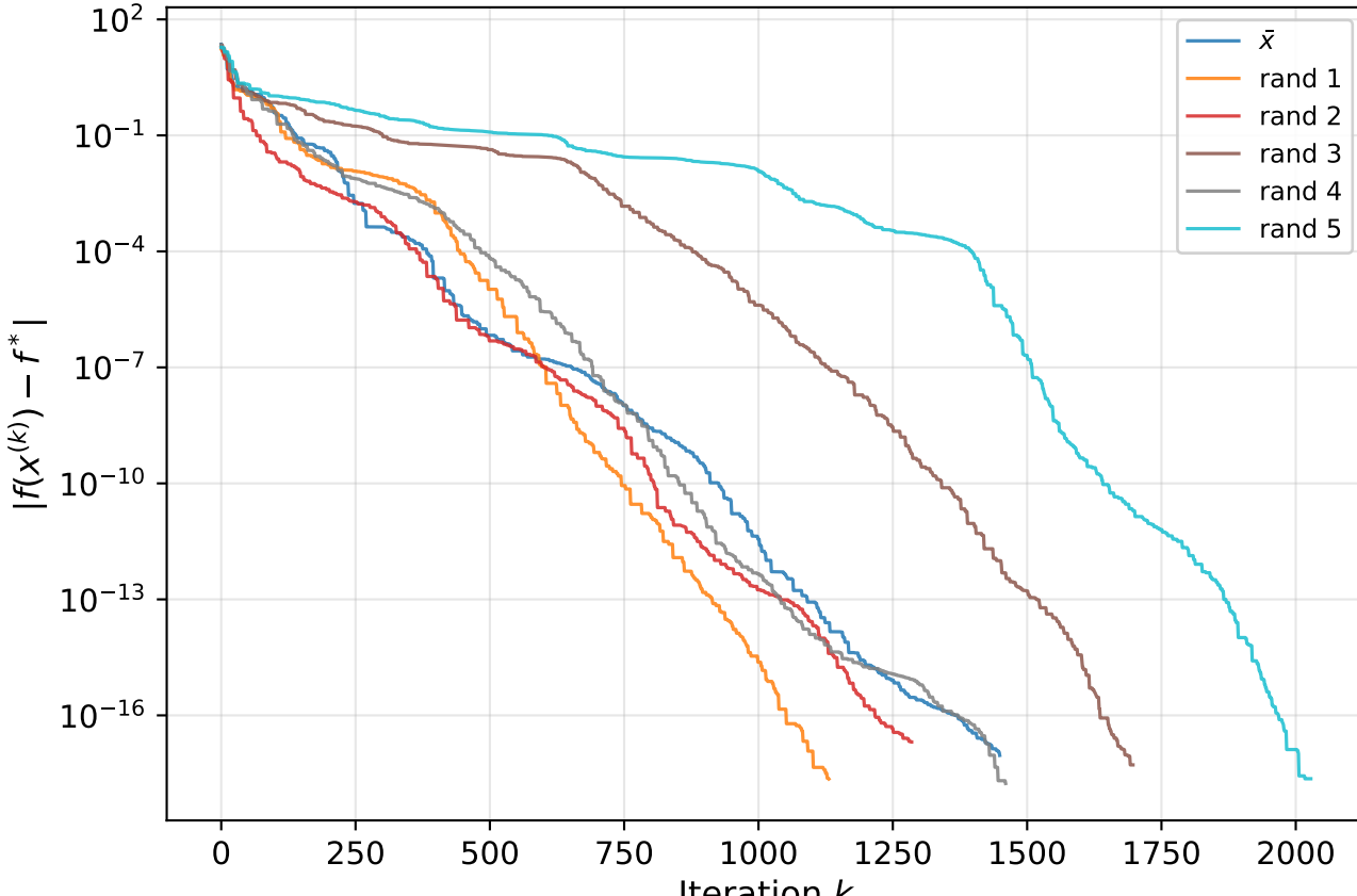
Levy — convergence ( n = 10 )
