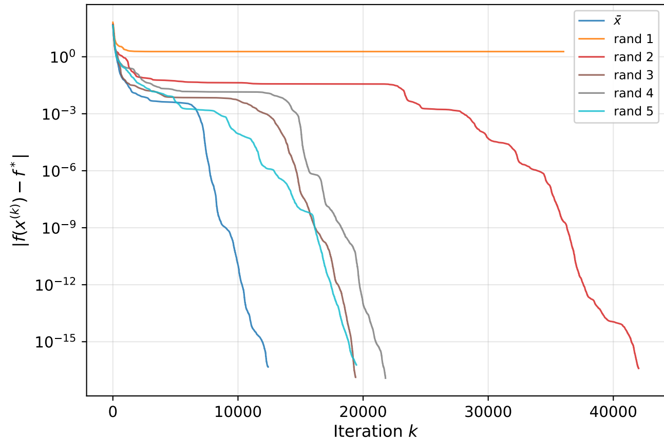
Levy — convergence ( n = 20 )
