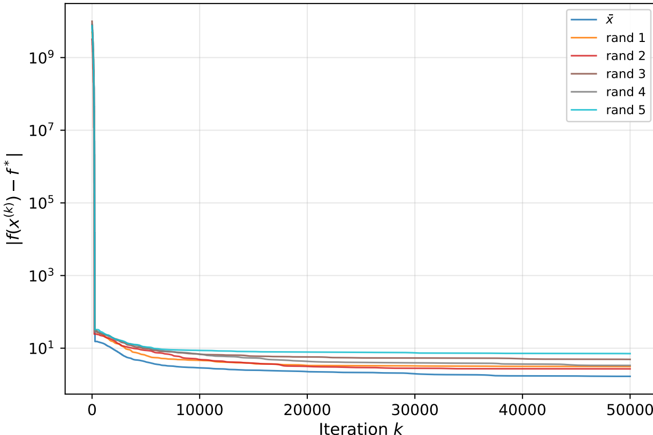
Zakharov — convergence ( n = 50 )
