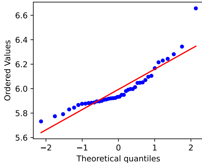
Q-Q plot: \log_{10} FIMO hits per motif Shapiro-Wilk p = 0.000142 , n = 42
