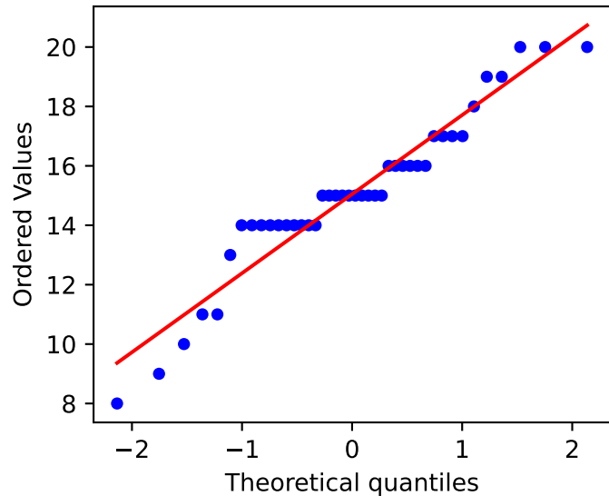
Q-Q plot: Mean motif width Shapiro-Wilk p = 0.016 , n = 42
