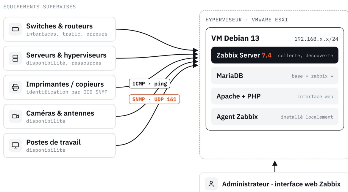
FIGURE 1 Architecture de la solution de supervision
