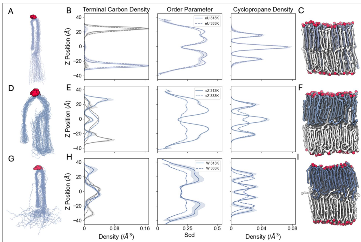
Figure 3. Folding patterns and organization of mycomembrane inner leaflet symmetric bilayers.
