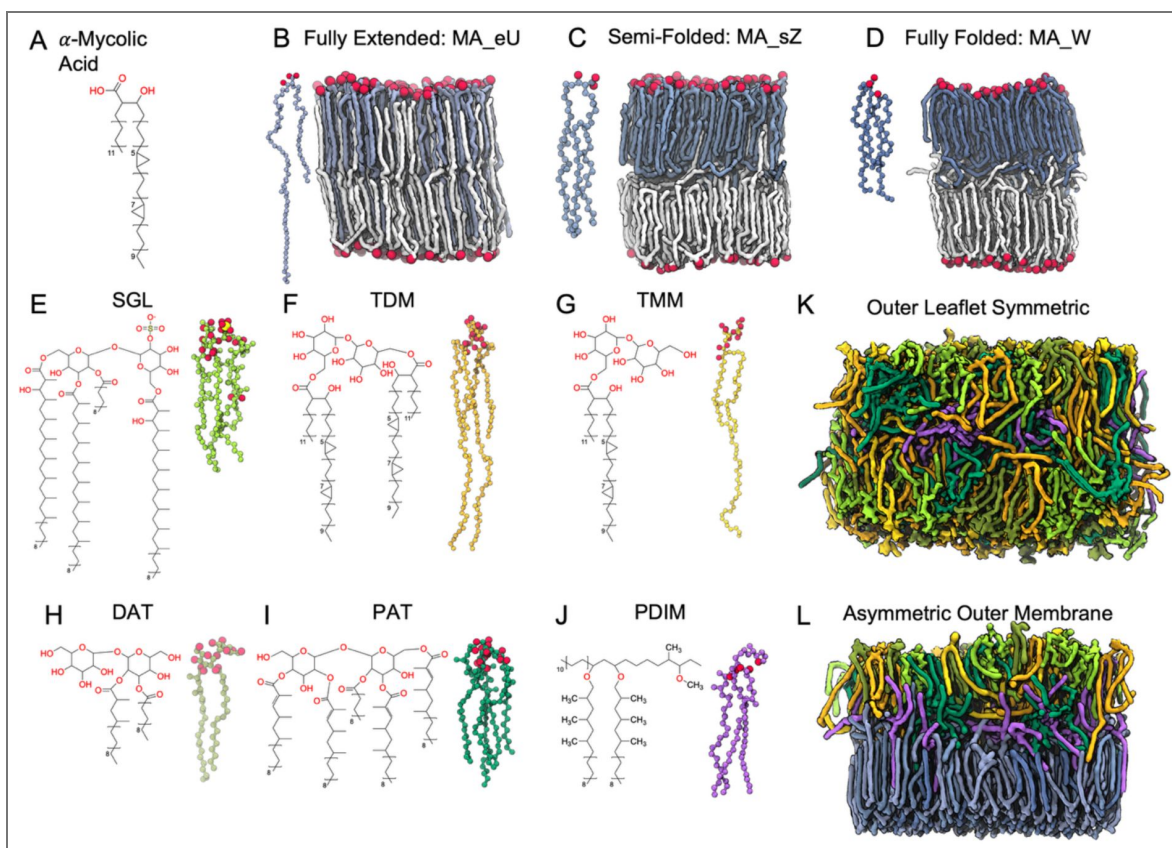
Figure 2. Chemical structures of mycobacterial lipids and membranes snapshots.
