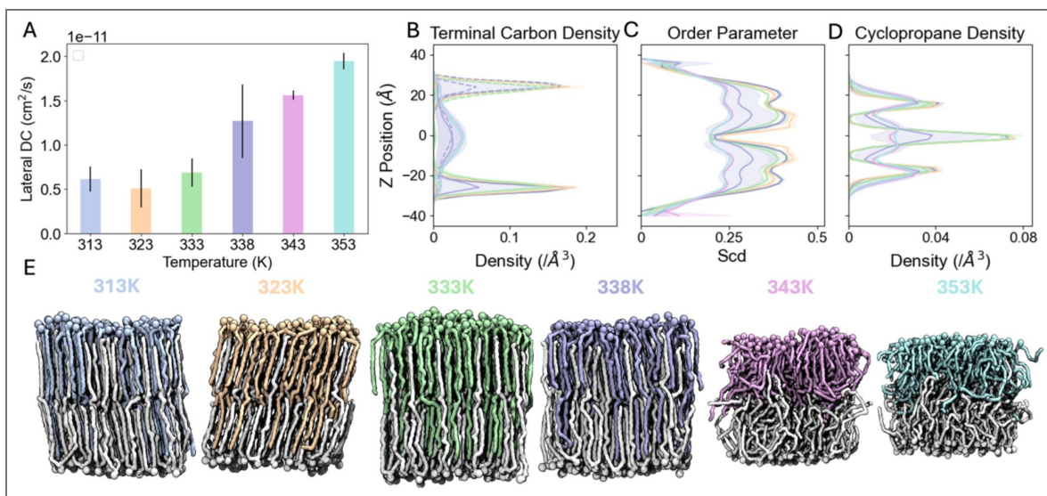
Figure 4. Phase transition of pure fully-extended \alpha -mycolic acid bilayers.
