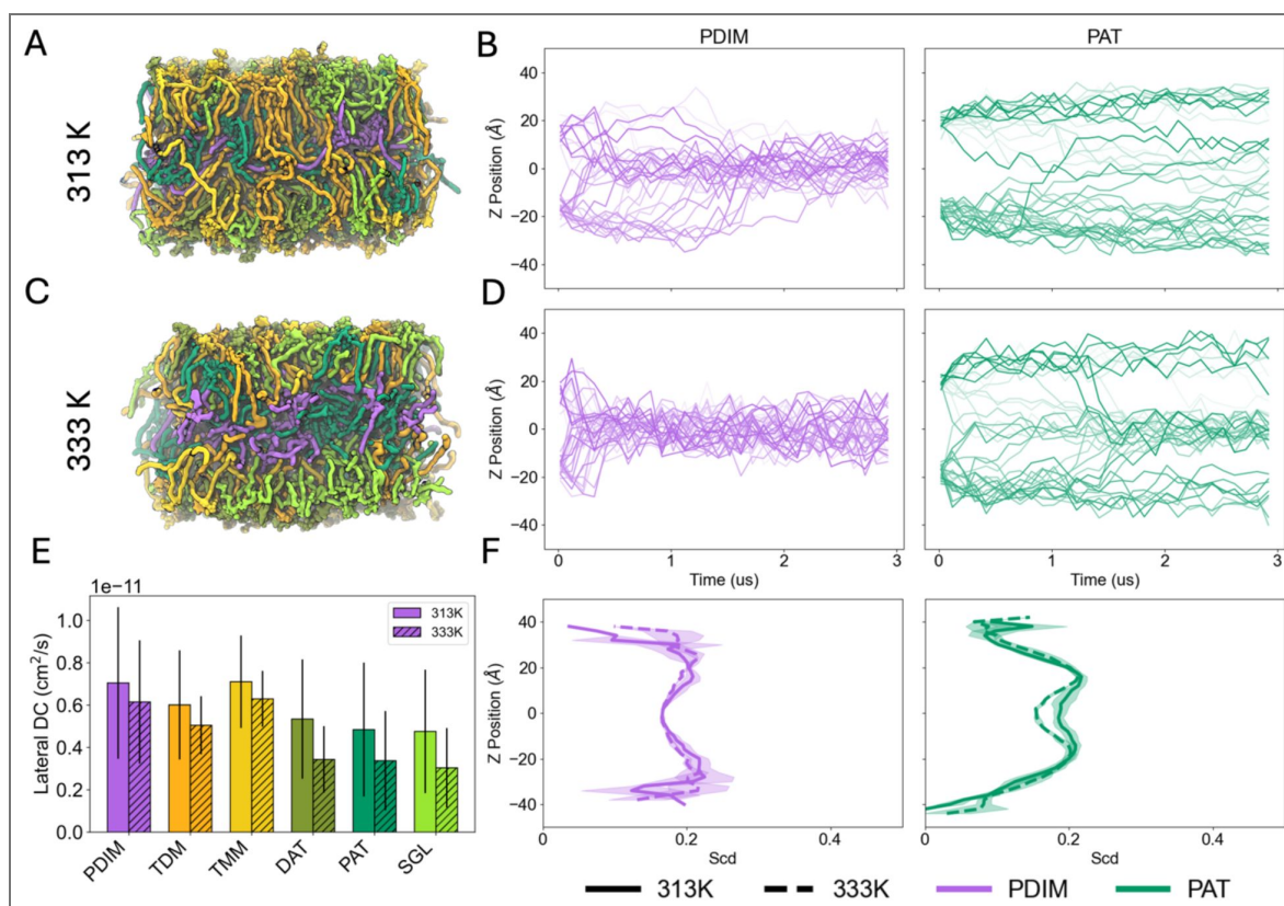
Figure 5. Lipid aggregation in mycomembrane outer leaflet symmetric bilayers.
