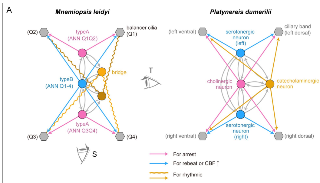
Figure 5. Comparison of neural circuits regulating ciliary movement
