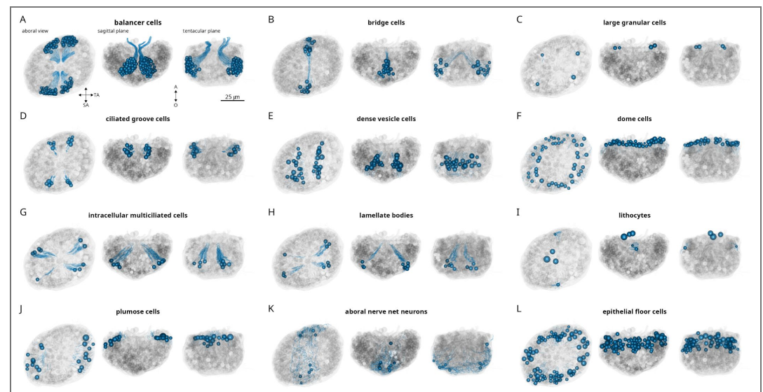
Figure 1—figure supplement 1. Cell-type composition of the ctenophore aboral organ Morphological rendering of skeletonised cell types, (A) balancer cells (B) bridge cells, (C) large granular cells, (D) ciliated groove cells, (E) dense vesicle cells, (F) dome cells, (G) intracellular multiciliated cells, (H) lamellate bodies, (I) lithocytes, (J) plumose cells, (K) aboral nerve-net neurons (L) epithelial floor cells.
