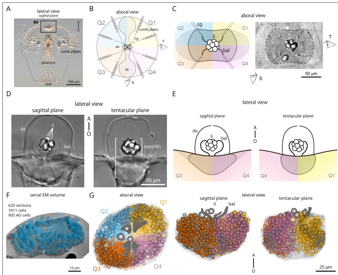
Figure 1. Morphology of the aboral organ in Mnemiopsis leidyi
