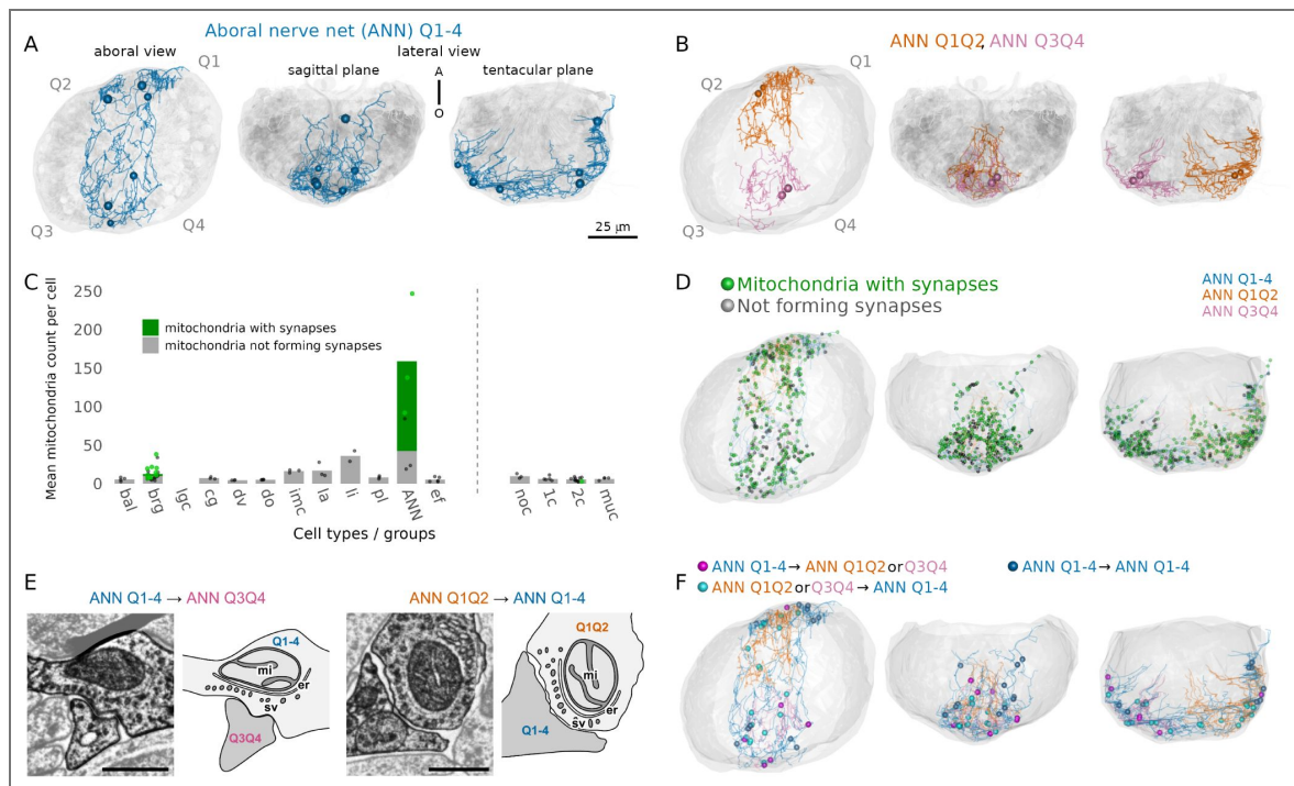
Figure 2. Organisation of the aboral synaptic nerve net
