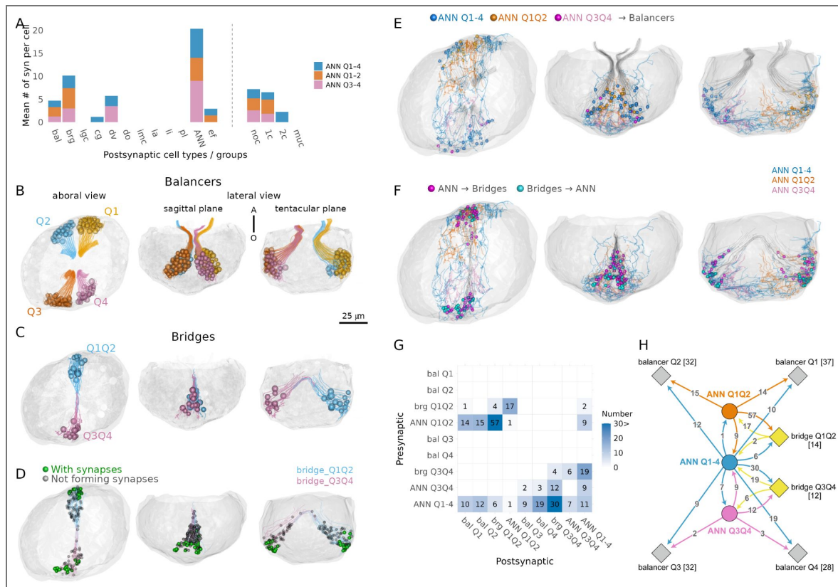
Figure 3. Synaptic connectivity of the balancer and bridge cells with the ANN.
