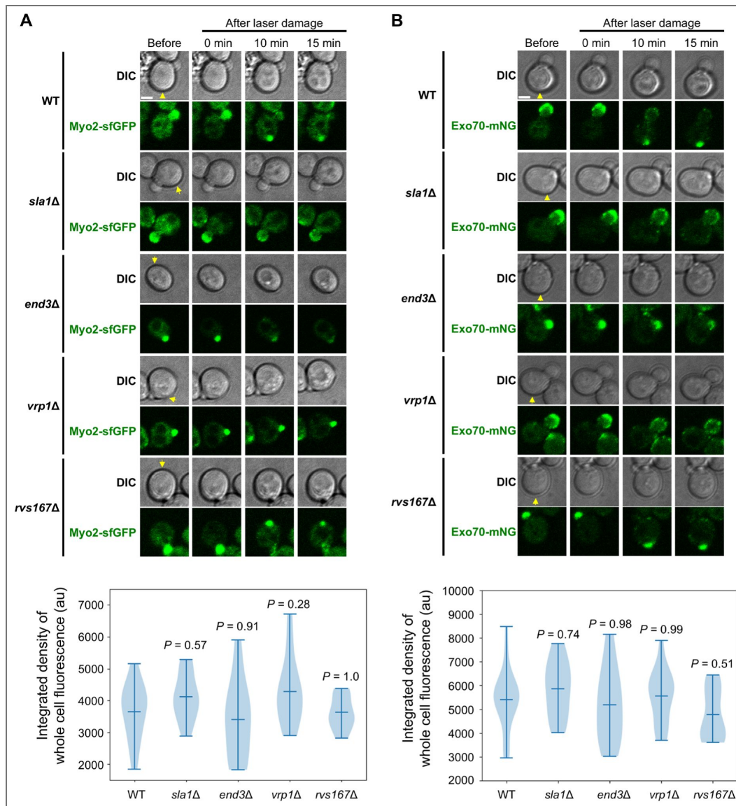
Fig. S6. Representative images of Myo2-sfGFP and Exo70-mNG in CME mutants.
