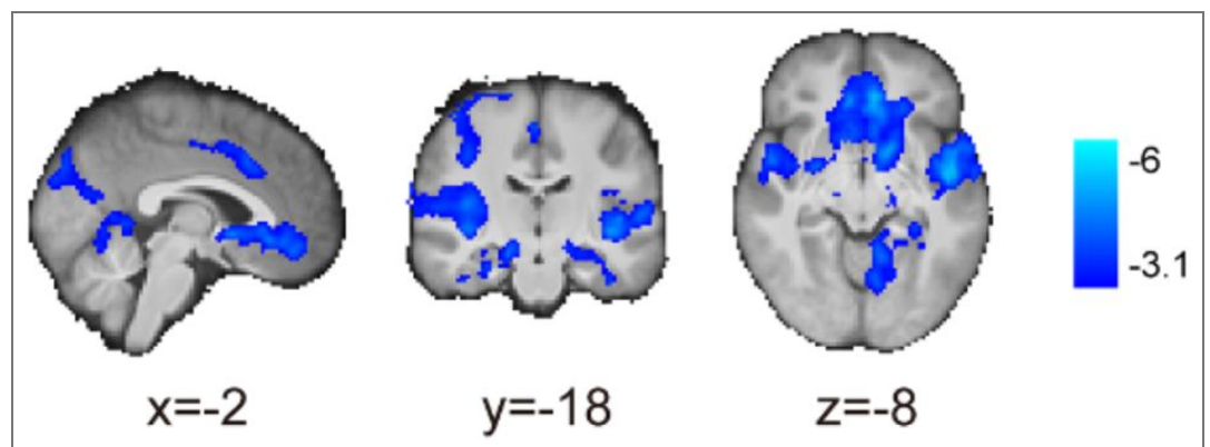
Figure S8. Whole-brain results on activity that significantly correlated with the subjects' log odds estimates of regime shift, \ln(P_t/(1 - P_t)) , where P_t represents subjects' probability estimates. In this analysis, we replaced the parametric regressor of P_t with the log odds of regime shifts in GLM-1. Color for significant activations: blue indicates negative correlation with \ln(P_t/(1 - P_t)) . Familywise error-corrected at p < .05 using Gaussian random field theory with a cluster-forming threshold z > 3.1 .
