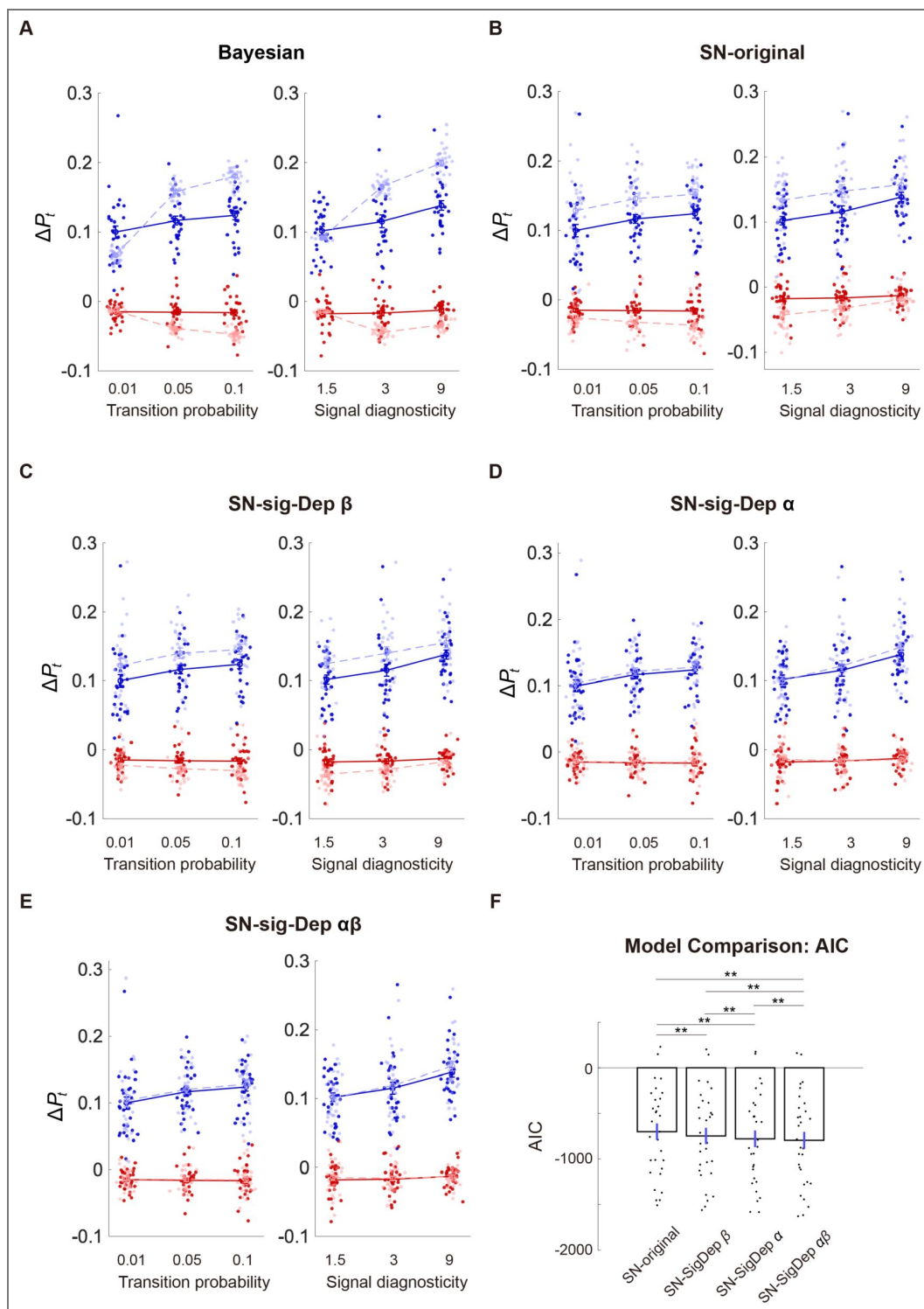
Figure 6. Model comparison.
