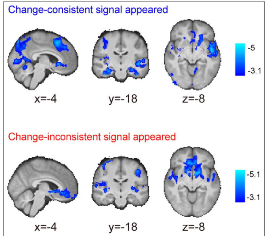
Figure S9. Probability estimates of regime shifts ( P_t ) separately analyzed for change-consistent (blue) and change-inconsistent (red) signals. Whole-brain results on activity that significantly correlated with probability estimates of regime shift for change-consistent and change-inconsistent signals. We observed that vmPFC correlated with P_t for both types of signals. Blue color showing significant activations indicates negative correlation with P_t . Familywise error-corrected at p < .05 using Gaussian random field theory with a cluster-forming threshold z > 3.1 .
