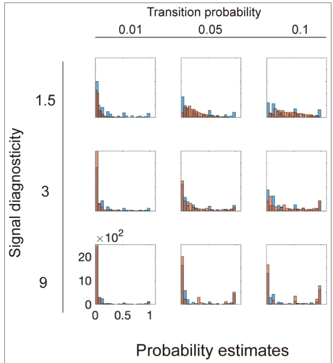
Figure S1. Probability estimates from all subjects are plotted as histograms separately for each condition—a combination of transition probability and signal diagnosticity. The blue bars represent the actual probability estimates, while the orange bars correspond to the probability estimates predicted by the Bayesian model.
