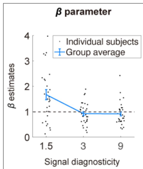
Figure S2. Experiment 2: estimates of the weighting parameter for signal diagnosticity ( \beta ) in the system-neglect model.
