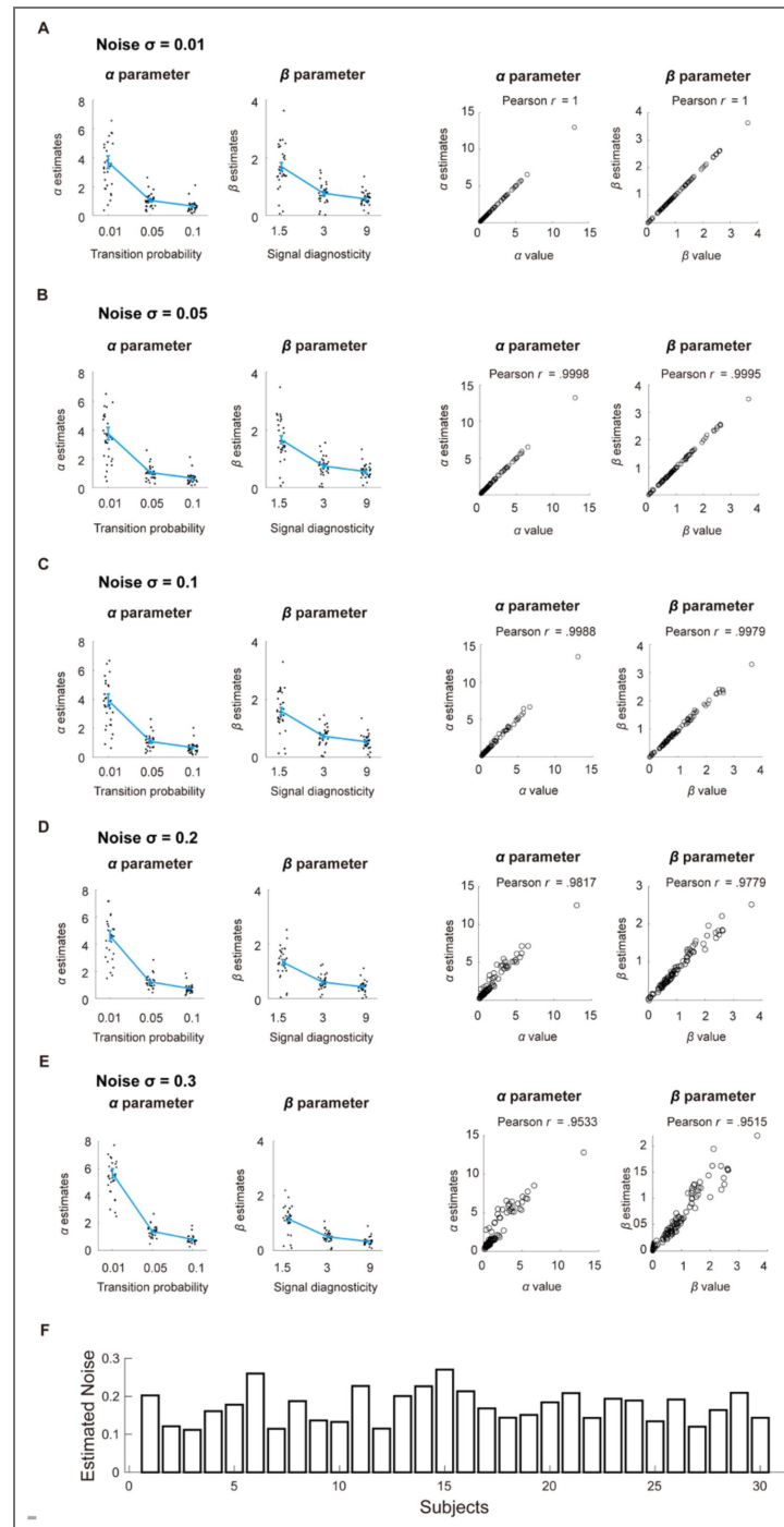
Figure S3. Parameter recovery.
