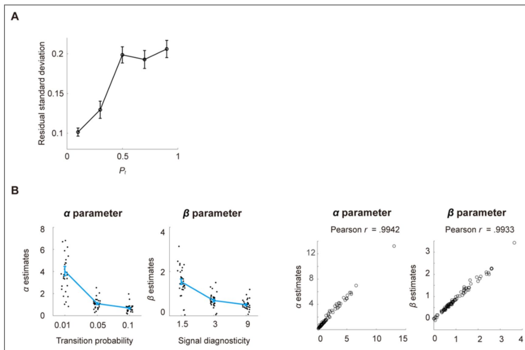
Figure S4. Impact of noise homoscedasticity on parameter estimation.
