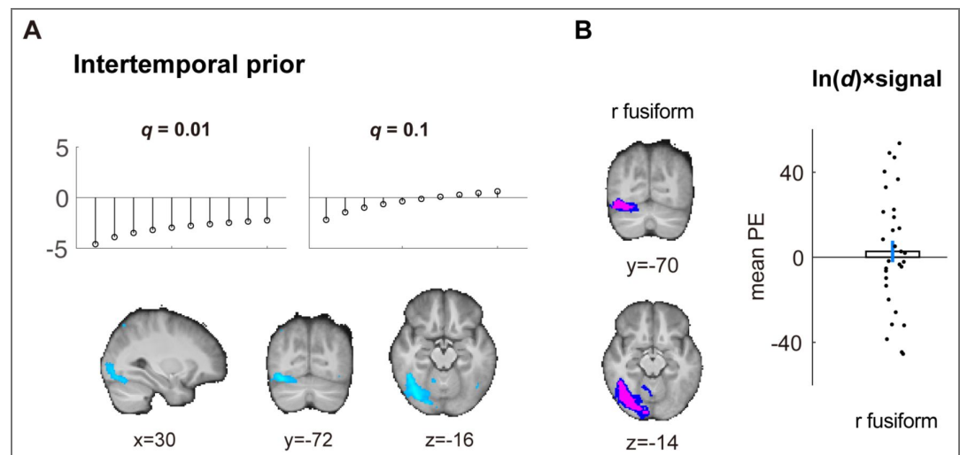
Figure S11. Key variables for regime-shift computations. A. Whole-brain results on the intertemporal prior of regime shift. B. Using the intertemporal prior ROI (left graph: magenta indicates voxels shared by the LOSO ROI of all subjects; blue indicates voxels of LOSO ROI of at least one subject) to examine the regression coefficients of the strength of evidence in favor of change, \ln(d) \times \text{signal} . The mean parameter estimates (mean PE), i.e., regression coefficient, was not significantly different from 0 (one-sample t test, t(29) = 0.54 , p = 0.59 , two-tailed).
