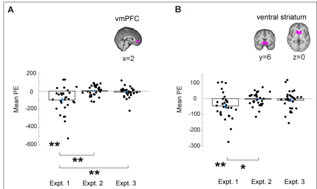
Figure S10. Independent region-of-interest (ROI) analysis in vmPFC and ventral striatum on probability estimates across the three experiments (Experiment 1 was the main experiment on regime-shift detection, Experiments 2 and 3 were control experiments). The vmPFC ROI we used was based on Bartrat et al. (2013). The ventral striatum mask was based on nucleus accumbens mask from Harvard-Oxford Cortical Structural Atlas. For each subject and each ROI, we extracted the mean parameter estimates (PE) of the probability estimates contrast in GLM-1. A. vmPFC ROI. Experiment 1: One-sample t test, t(29) = -3.82 , p < 0.01 ; Experiment 2: One-sample t test, t(29) = 0.36 , p = 0.71 ; Experiment 3: One-sample t test, t(29) = -1.11 , p = 0.28 ; Experiments 1 - Experiment 2: two-sample t test, t(58) = -3.67 , p < 0.01 ; Experiments 1 - Experiment 3: two-sample t test, t(58) = -3.12 , p < 0.01 ; B. Ventral striatum ROI. Experiment 1: t(29) = -3.06 , p < 0.01 ; Experiment 2: t(29) = 0.44 , p = 0.67 ; Experiment 3: t(29) = -0.93 , p = 0.36 ; Experiments 1 - Experiment 2: t(58) = -2.55 , p = 0.01 ; Experiments 1 - Experiment 3: t(58) = -1.95 , p = 0.06 . The * symbol indicates p < 0.05 (two-tailed), and ** symbol indicates p < 0.01 (two-tailed).
