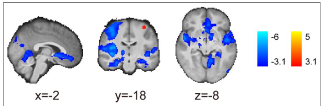
Figure S7. Whole-brain results on activity that significantly correlated with probability estimates of regime shift ( P_t ) in GLM-2. In GLM-2, we implemented variables important for estimating regime shifts as parametric regressors in addition to P_t . In particular, the intertemporal prior that captured the prior probability of change increasing as a function of time was included in the GLM-2. Still, we observed P_t correlates in the vmPFC and ventral striatum after controlling for these variables. Color for significant activations: blue indicates negative correlation with P_t ; yellow indicates positive correlation with P_t . Familywise error-corrected at p < .05 using Gaussian random field theory with a cluster-forming threshold z > 3.1 .
