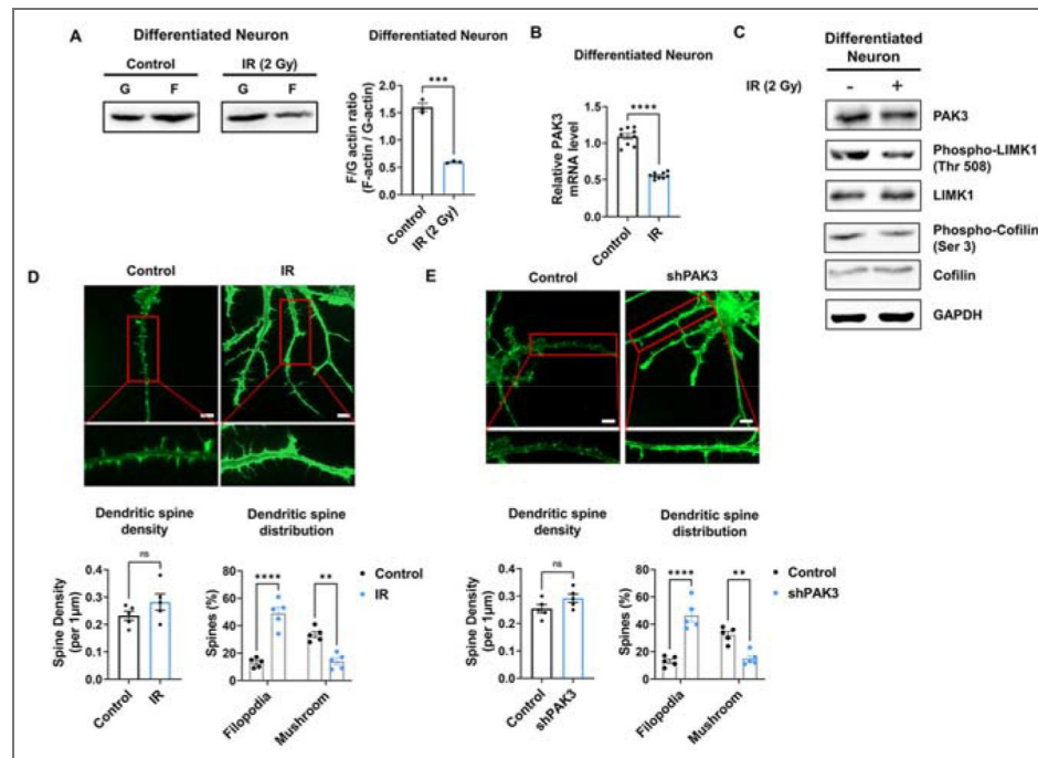
Fig 4. IR decreases PAK3-LIMK1-Cofilin signaling in differentiated human neuron
