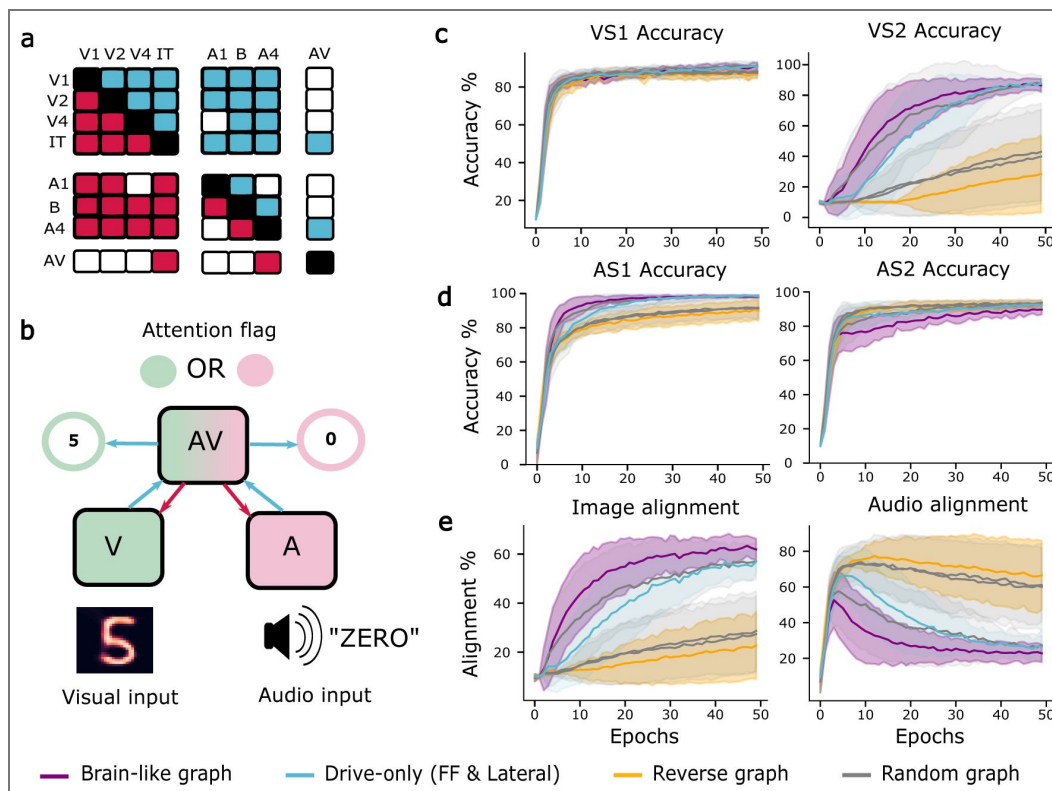
Figure S4. Models with multiplicative feedback on audiovisual switching task.
