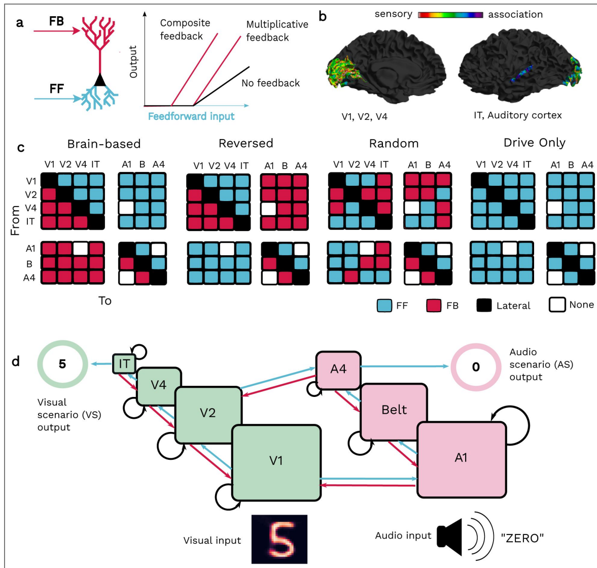
Figure 1. Description of models.
