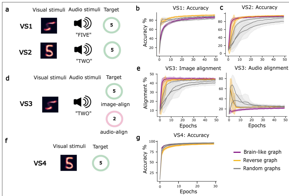
Figure 2. Multimodal visual tasks.
