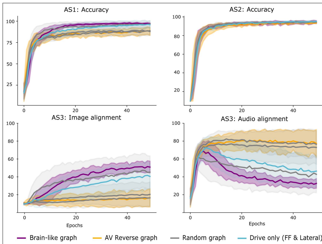
Figure S2. Performance of larger model (hidden state size 32) on AS tasks.
