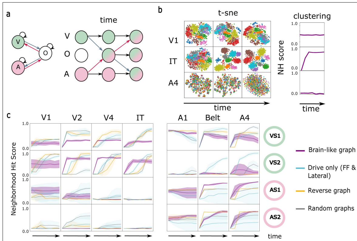
Figure 6. Model activity during multimodal tasks.
