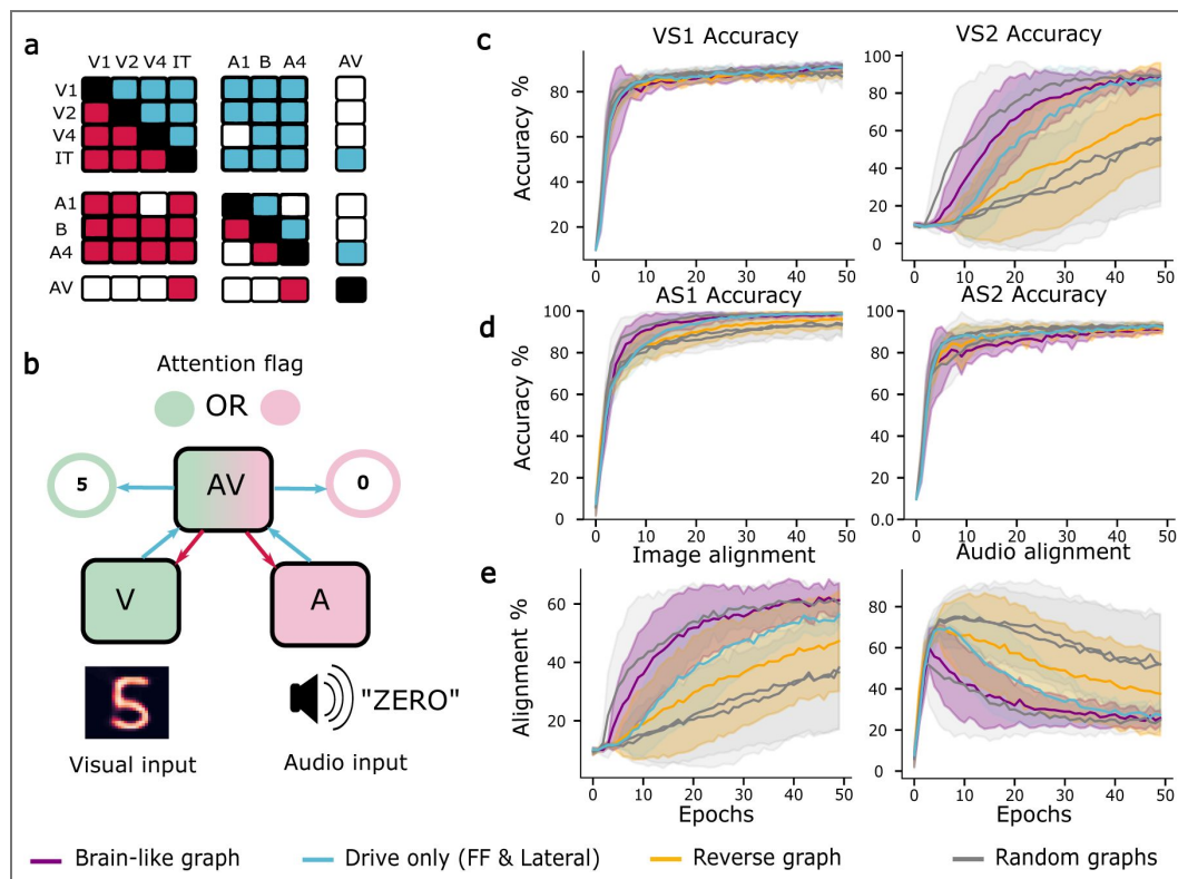
Figure 5. Audiovisual switching task.
