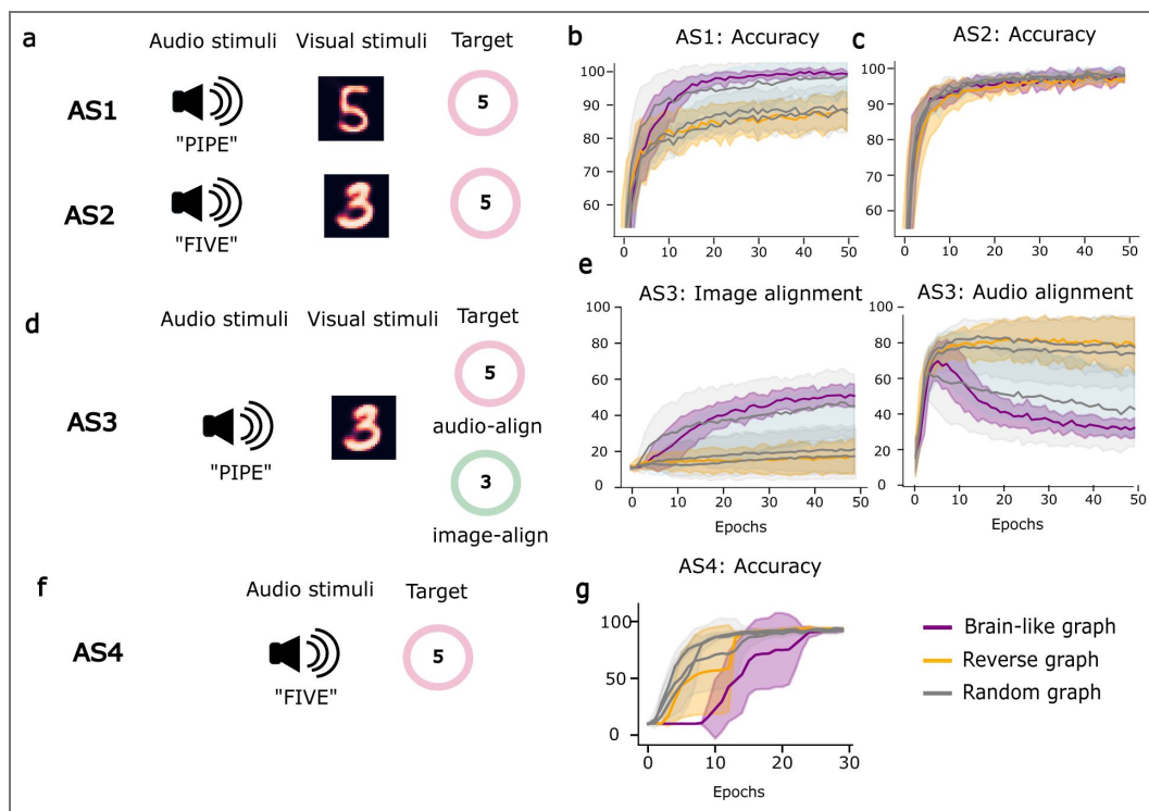
Figure 3. Multimodal auditory tasks.
