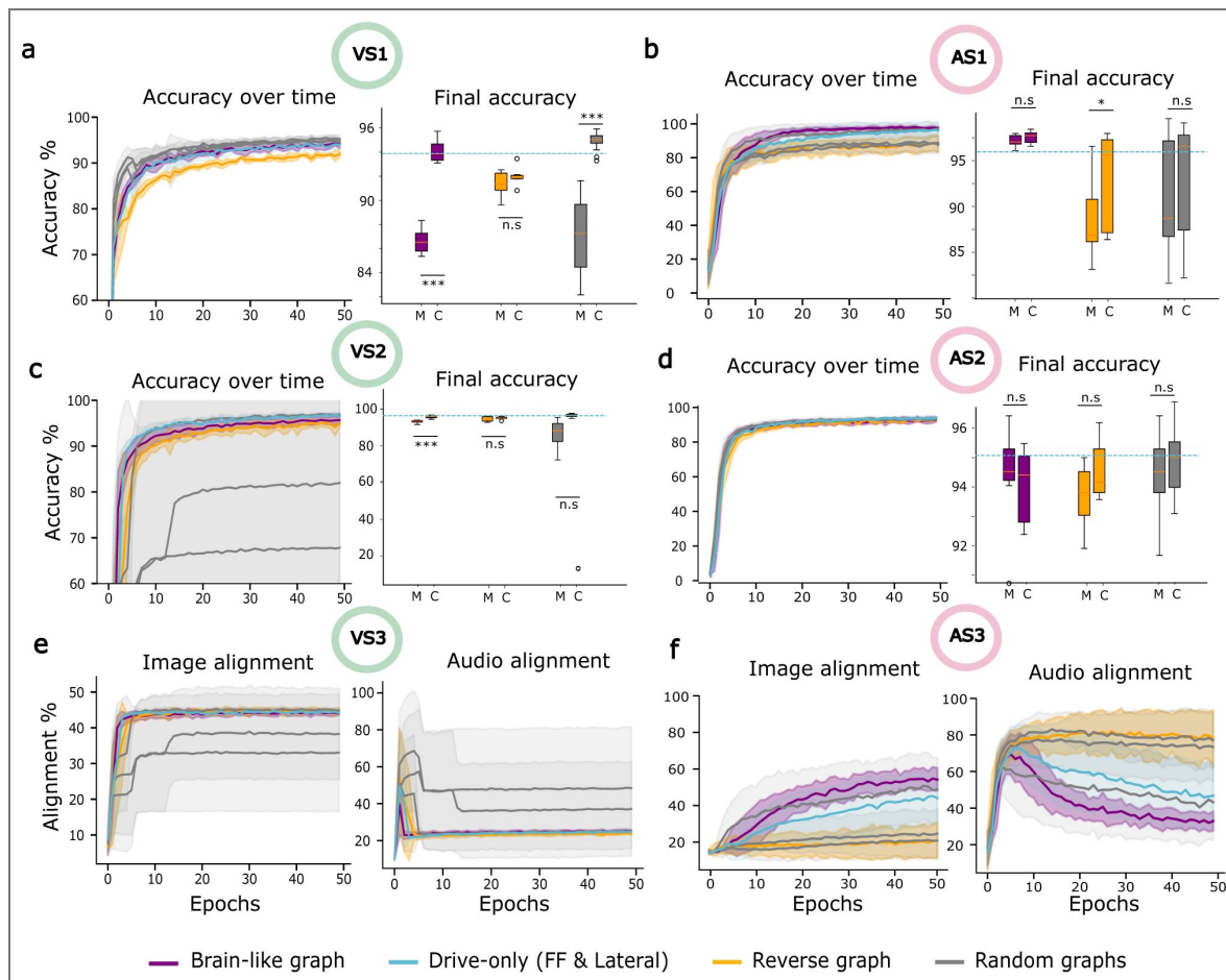
Figure 4. Composite versus multiplicative feedback in multimodal tasks.
