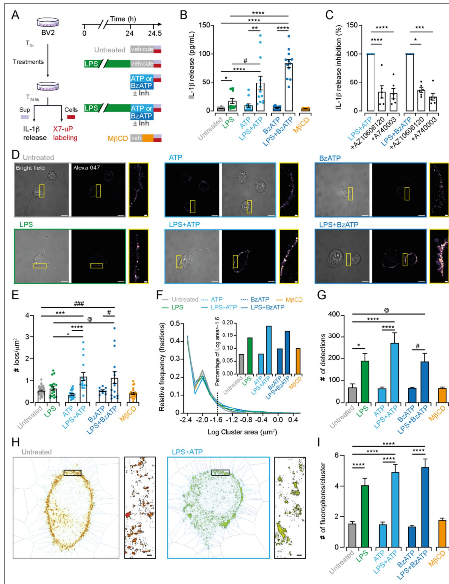
Figure 5. dSTORM data revealed nanoscale P2X7 plasma membrane localization in BV2 cells.
