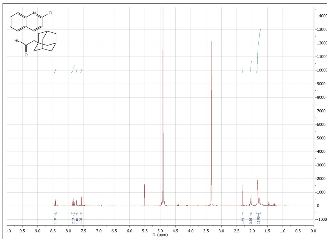
Figure 1 — figure supplement 5. ^1\text{H} NMR spectrum of compound 6.
