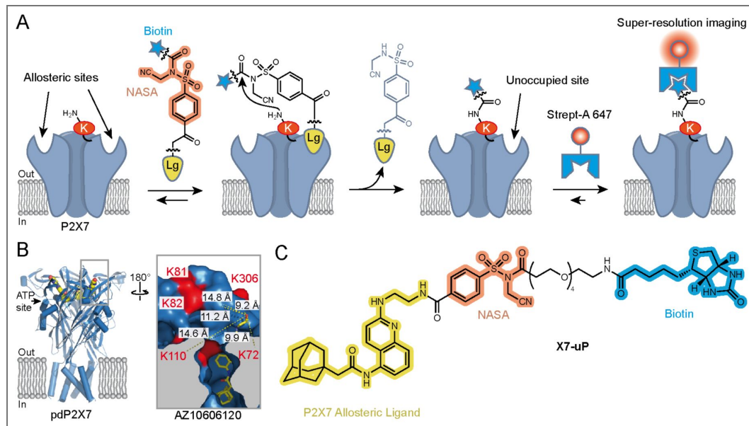
Figure 1. Affinity-guided labeling strategy for P2X7.
