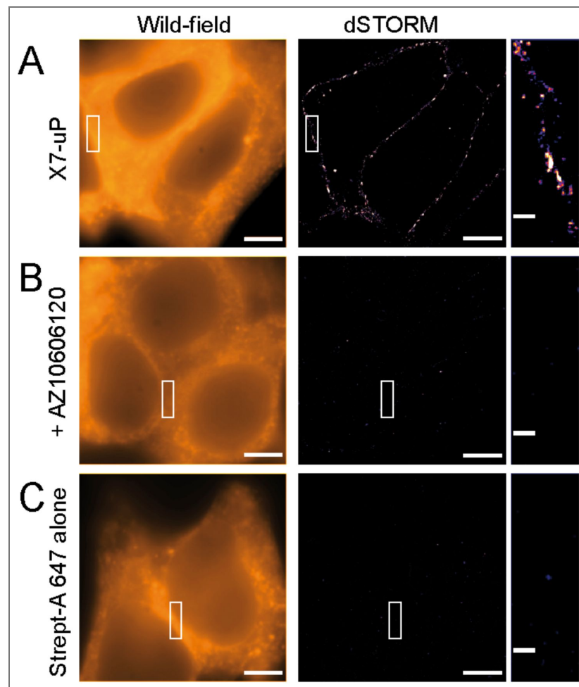
Figure 3 — figure supplement 2. dSTORM images of HEK293T cells transfected with P2X7-mScarlet.
