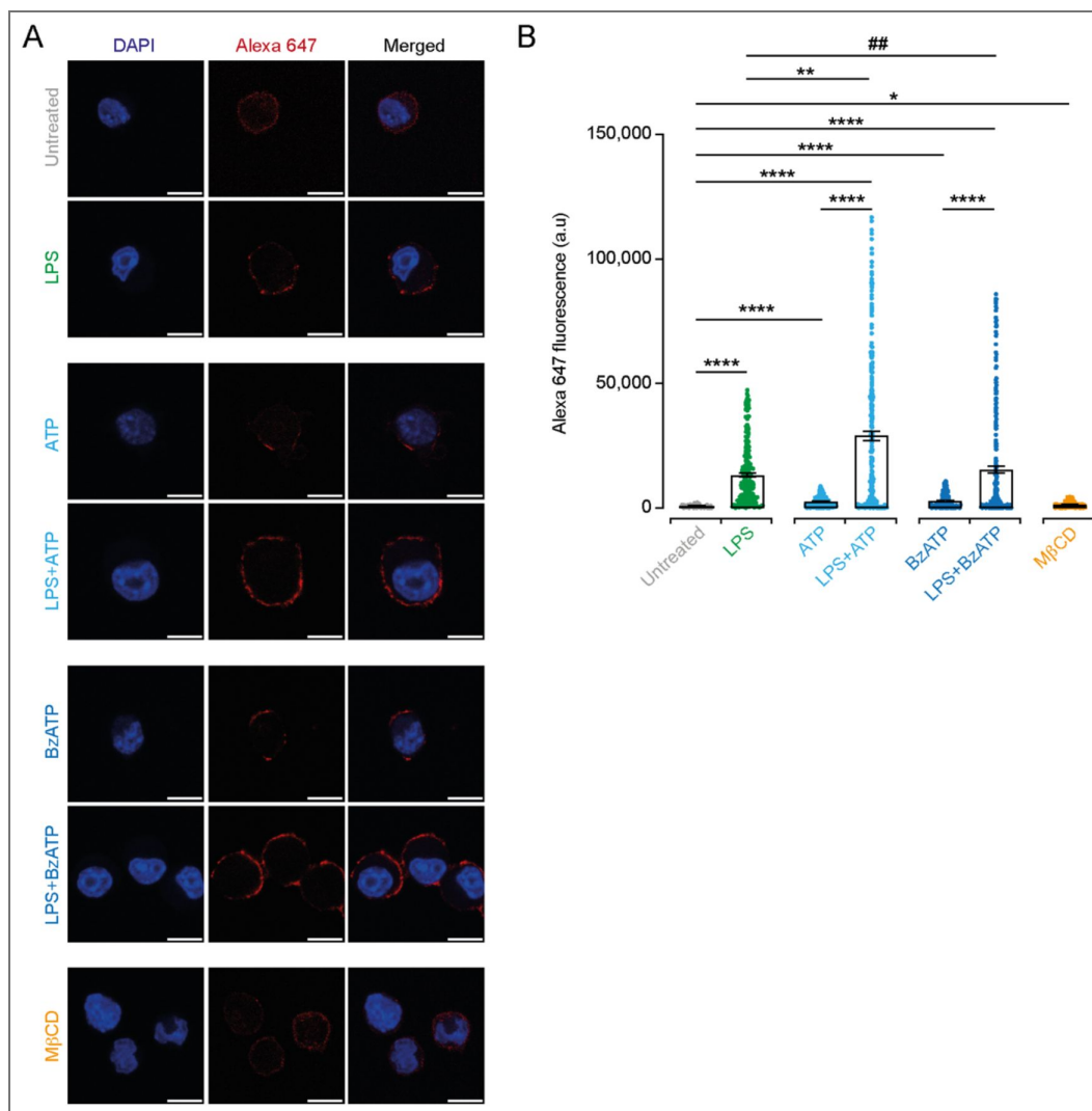
Figure 5 — figure supplement 4. Confocal data of X7-uP-induced P2X7 labeling in BV2 cells.
