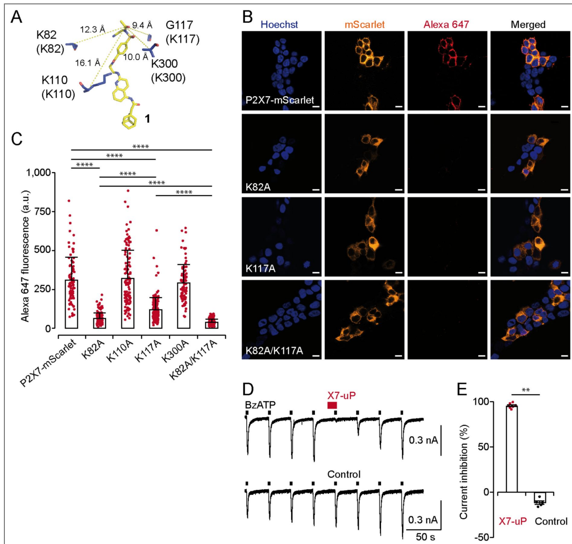
Figure 4. X7-uP labels K82 and K117 in rat P2X7.
