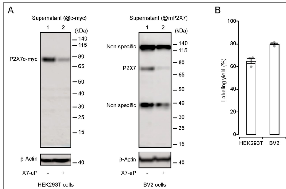
Figure 2 — figure supplement 2. Determination of X7-uP-induced P2X7 labeling yields in HEK293T and BV2 cells.
