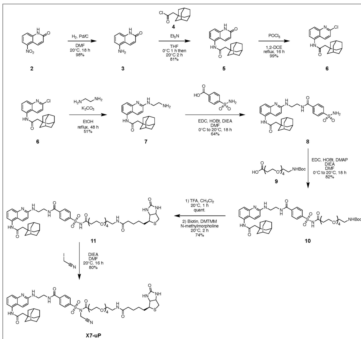
Figure 1 — figure supplement 2. Multi-step synthesis of X7-uP.
