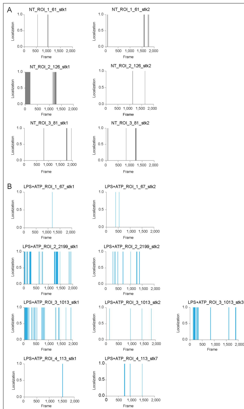
Figure 5 — figure supplement 3. Blink detection features.
