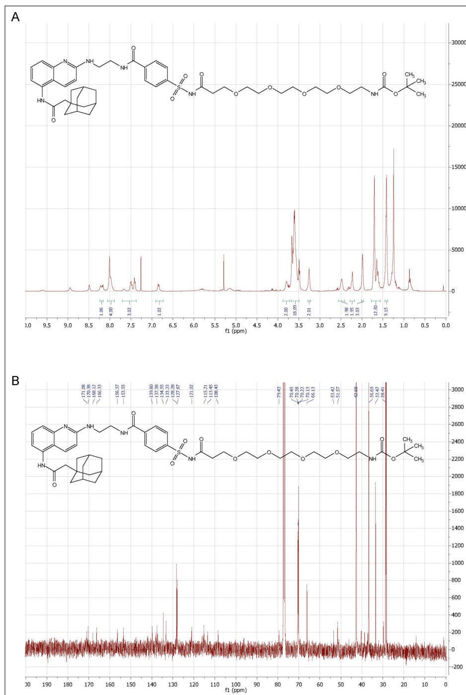
Figure 1 — figure supplement 8. ^1\text{H} NMR (A) and ^{13}\text{C} NMR (B) spectra of compound 10.
