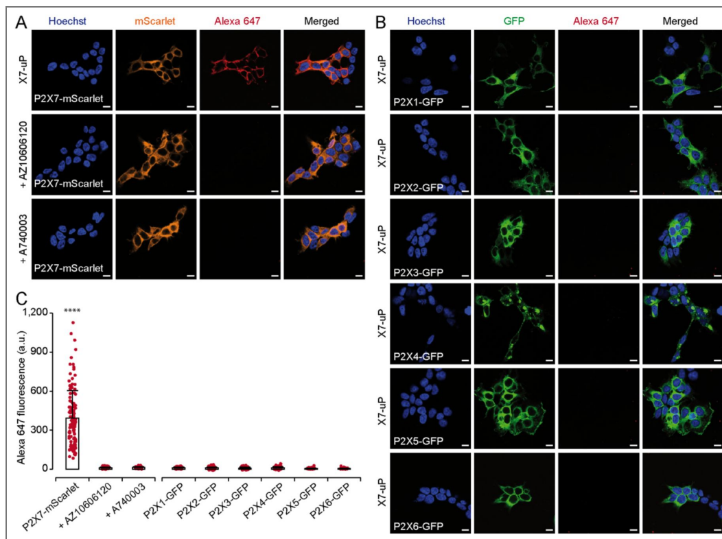
Figure 3. X7-uP labeling is highly selective for P2X7.
