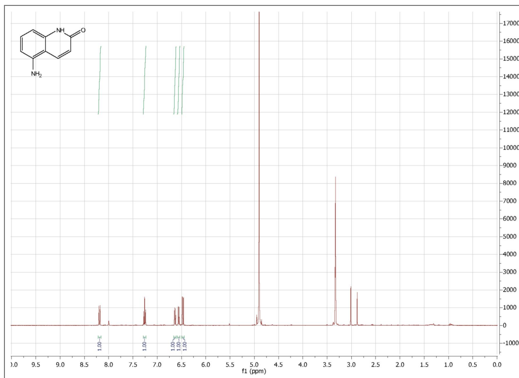
Figure 1 — figure supplement 3. ^1\text{H} NMR spectrum of compound 3.
