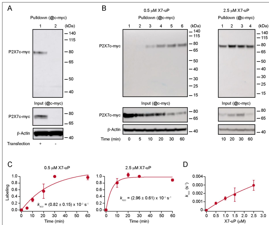
Figure 2 — figure supplement 1. Specificity and kinetic analysis of P2X7 labeling by X7-uP.
