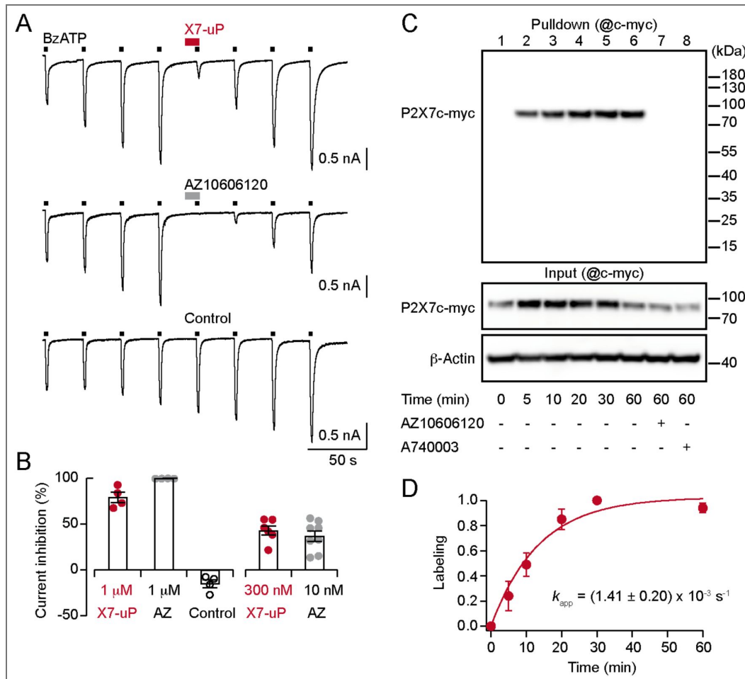
Figure 2. X7-uP is a potent P2X7 inhibitor that rapidly labels ectopically expressed P2X7 in HEK293T cells.
