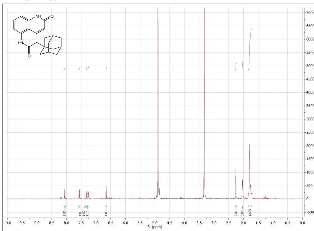
Figure 1 — figure supplement 4. ^1\text{H} NMR spectrum of compound 5.
