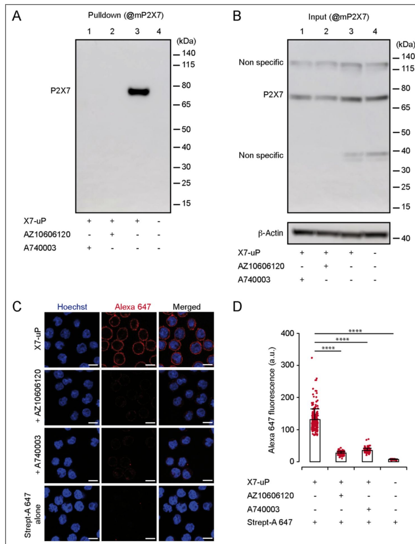
Figure 5 — figure supplement 1. X7-uP-induced P2X7 labeling in BV2 cells.
