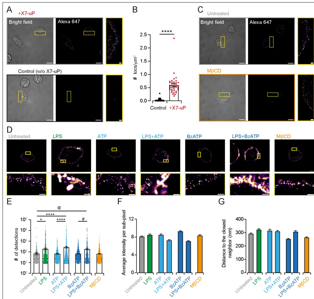
Figure 5 — figure supplement 2. dSTORM analysis of X7-uP-induced P2X7 labeling in BV2 cells.
