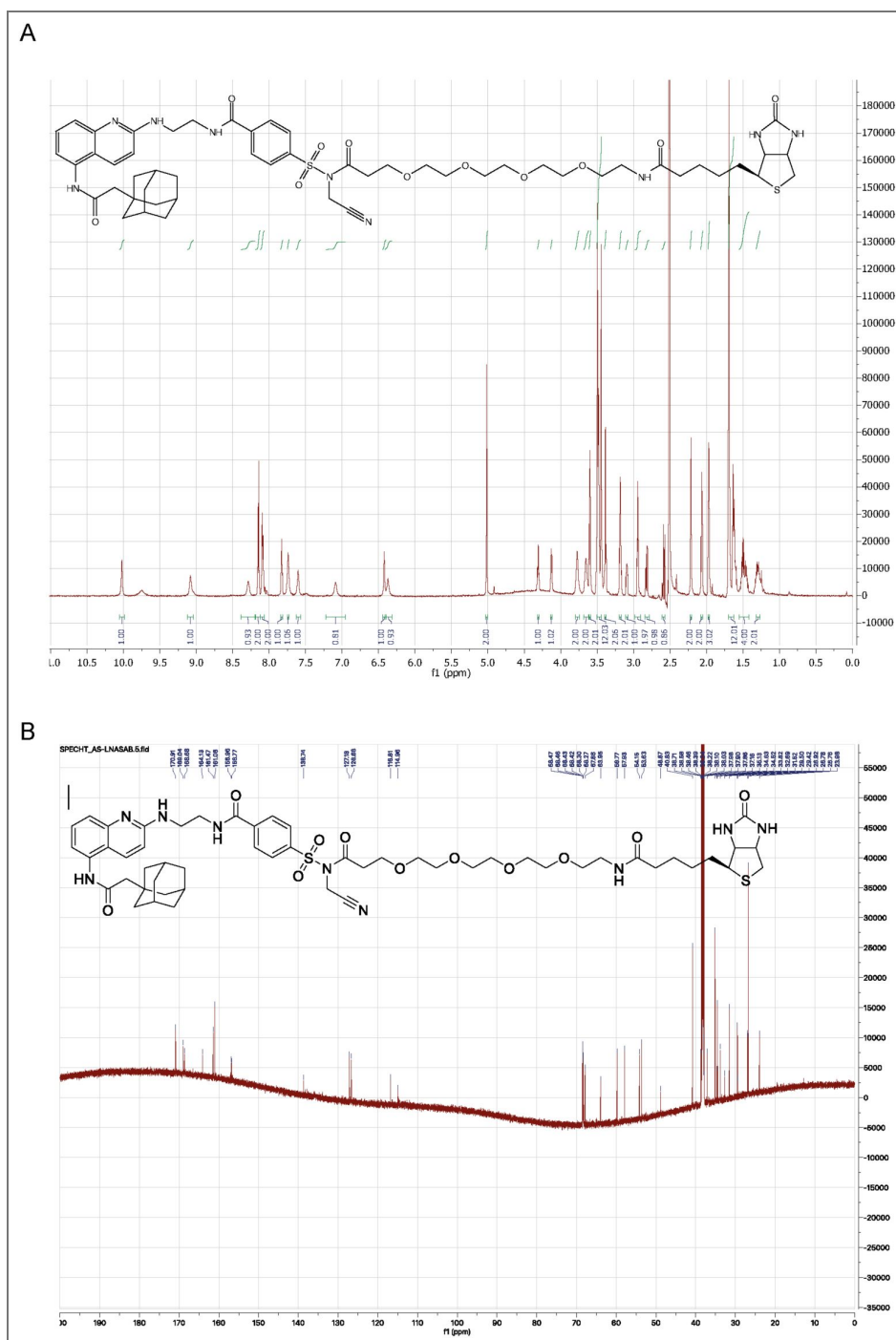
Figure 1 — figure supplement 10. ^1\text{H} NMR (A) and ^{13}\text{C} NMR (B) spectra of compound X7-uP.
