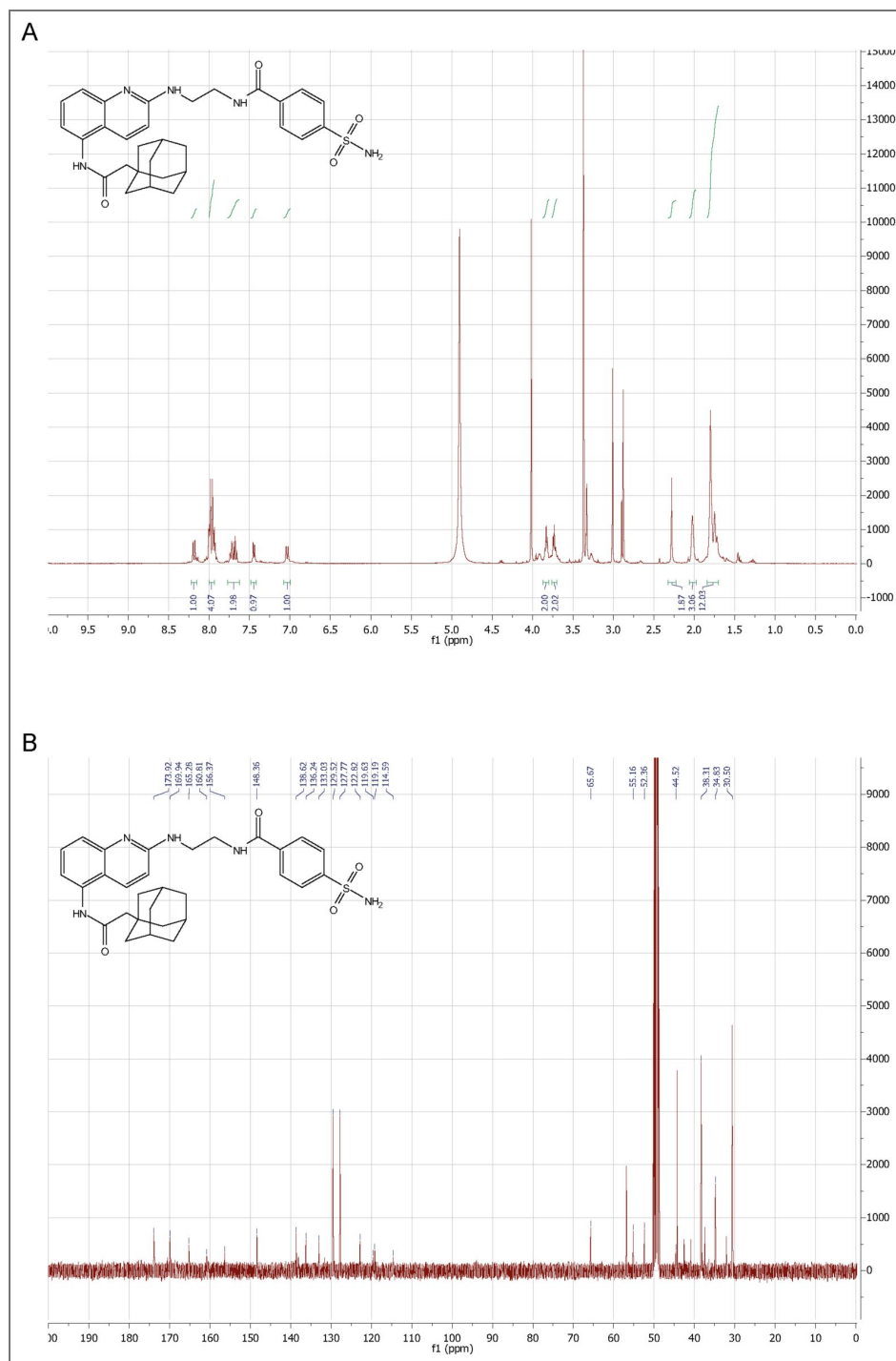
Figure 1 — figure supplement 7. ^1\text{H} NMR (A) and ^{13}\text{C} NMR (B) spectra of compound 8.
