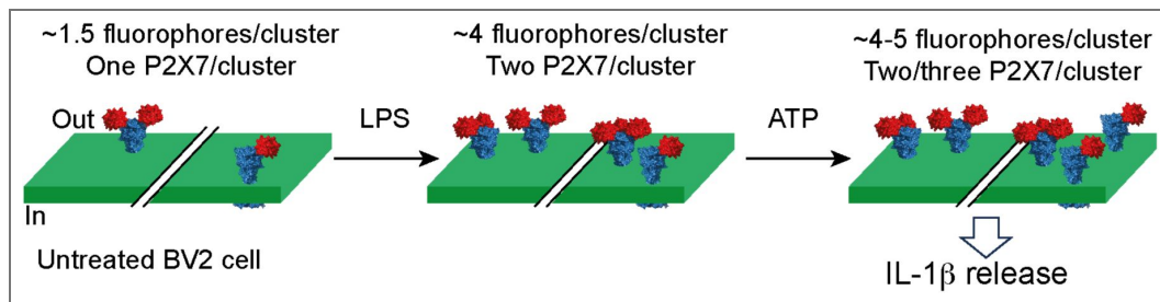
Figure 6. Nanoscale redistribution of individual P2X7 receptors in microglia under pro-inflammatory conditions at the plasma membrane.
