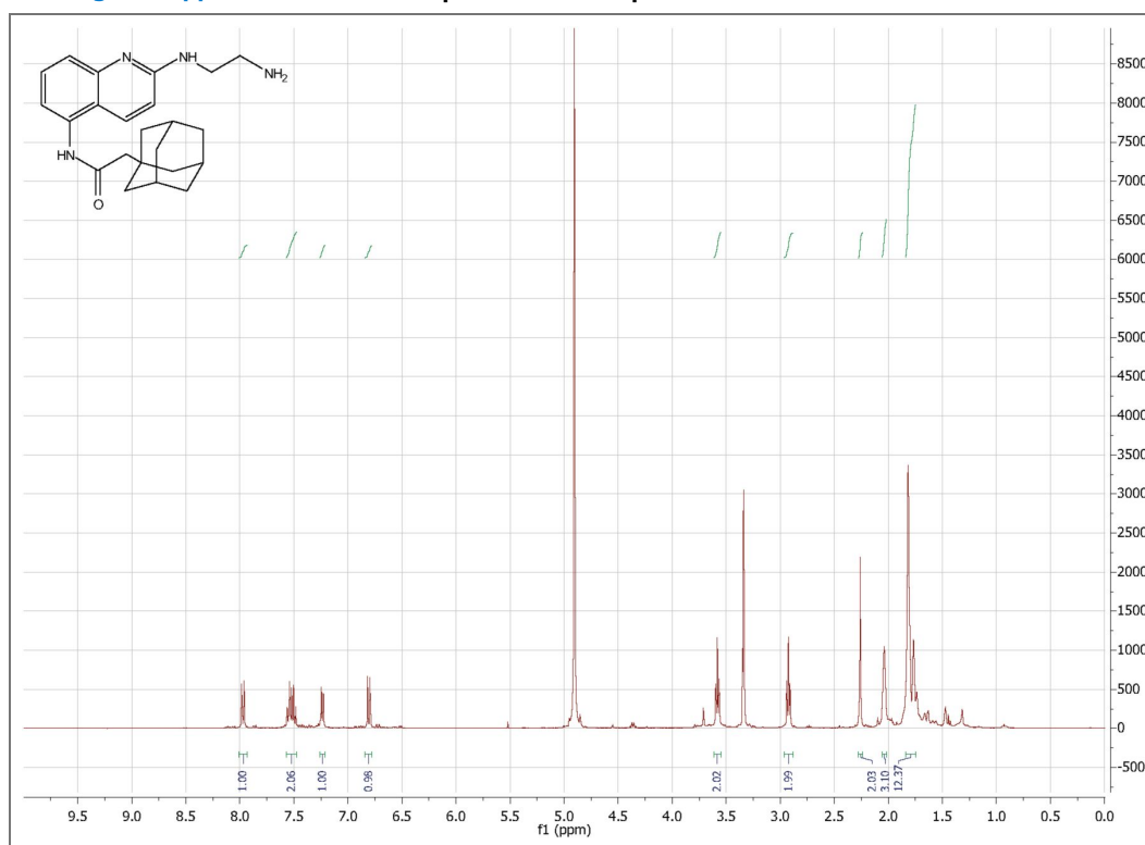
Figure 1 — figure supplement 6. ^1\text{H} NMR spectrum of compound 7.
