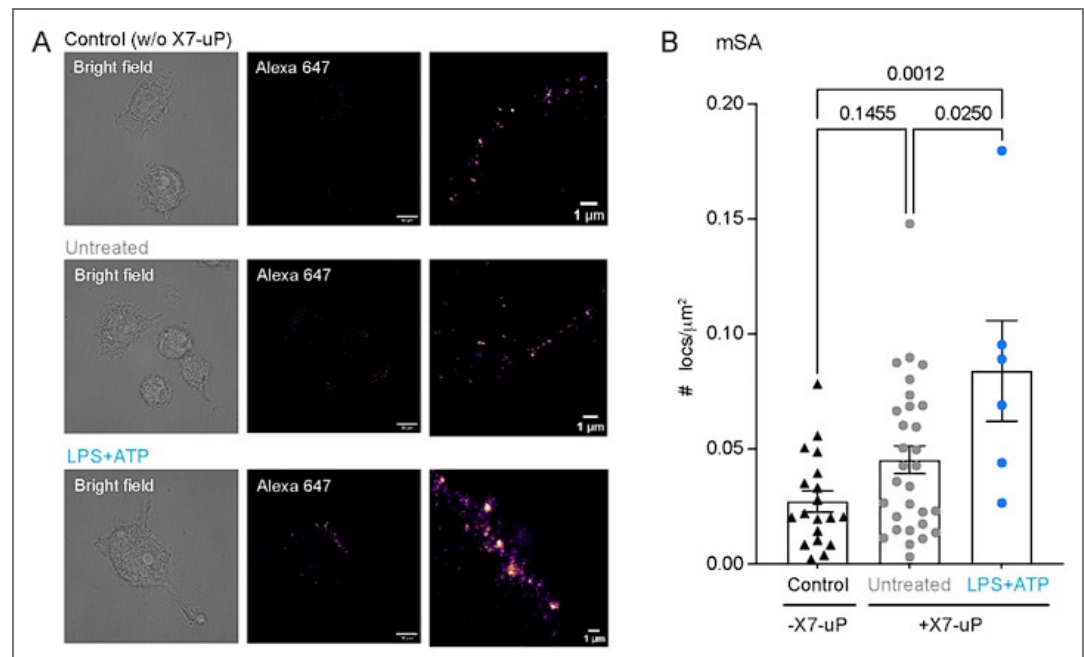
Author response image 1. BV2 labeling with monomeric streptavidin-Alexa 647 (mSA). (A) Bright-field and dSTORM images of BV2 cells labeled with mSA in the presence (untreated and LPS+ATP) or absence (control) of 1 \mu M X7-uP. Treatment: LPS (1 \mu g/mL for 24 hours) and ATP (1 mM for 30 minutes). Scale bars, 10 \mu m. Insets: Magnified dSTORM images. Scale bars, 1 \mu m. (B) Quantification of the number of localizations ( n = 2 independent experiments). Bars represent mean \pm s.e.m. One-way ANOVA with Tukey's multiple comparisons (P values are indicated above the graph).
