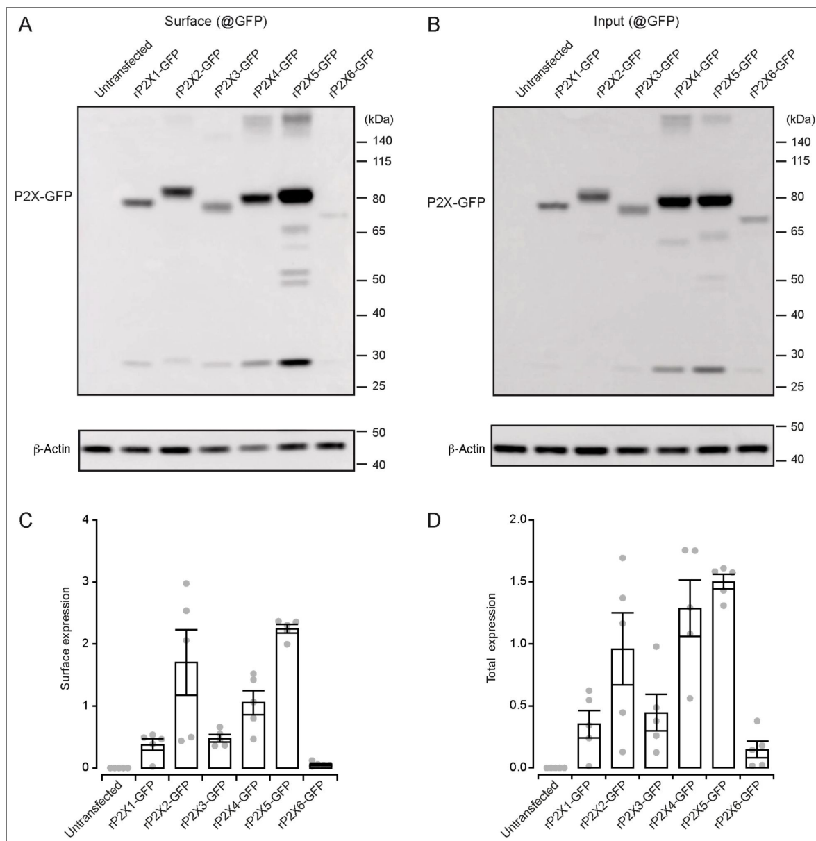
Figure 3 — figure supplement 1. Cell-surface labeling assay of HEK293T cells transfected with various GFP-tagged P2X subunits.
