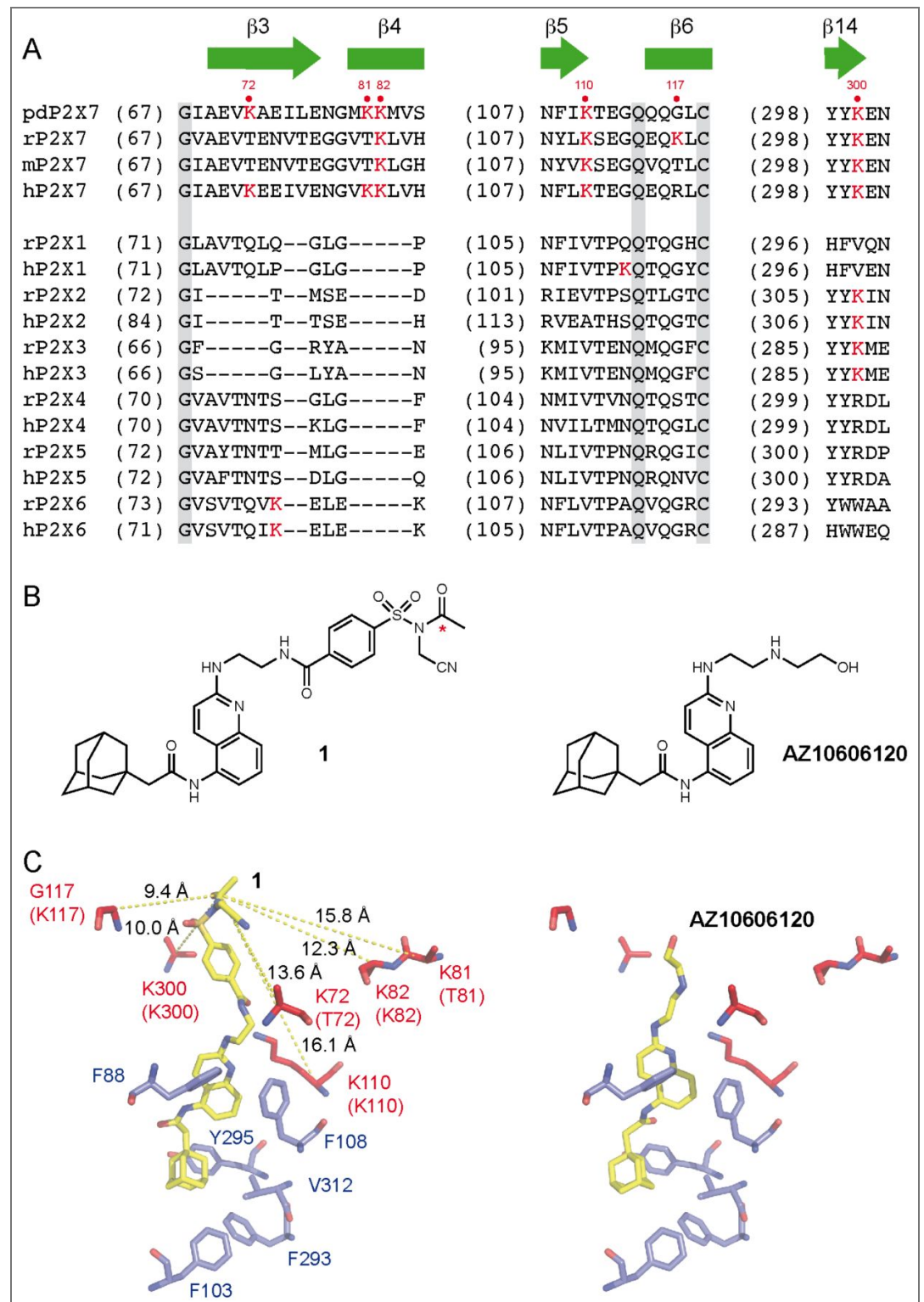
Figure 1 — figure supplement 1. Mapping the X7-uP labeling site. (A) Sequence alignment of selected regions from P2X receptors: panda P2X7 (pdP2X7), rat P2X7 (rP2X7), mouse P2X7 (mP2X7), human P2X7 (hP2X7), and rat and human P2X1-6 (rP2X1-6, hP2X1-6). Lysine residues are highlighted in red. Secondary structure elements are depicted in cartoon representation and are labeled as in the crystal structure of pdP2X7 (Karasawa & Kawate, 2016). (B) Chemical structures of compound 1 and AZ10606120. Red star indicates electrophilic carbon of the N-cyanomethyl group. (C) Right, crystal structure of AZ10606120 (stick representation) bound to pdP2X7 (PDB:5U1W) (Karasawa & Kawate, 2016). Left, same view with 1 docked to pdP2X7 (left). Distances (in Å)
