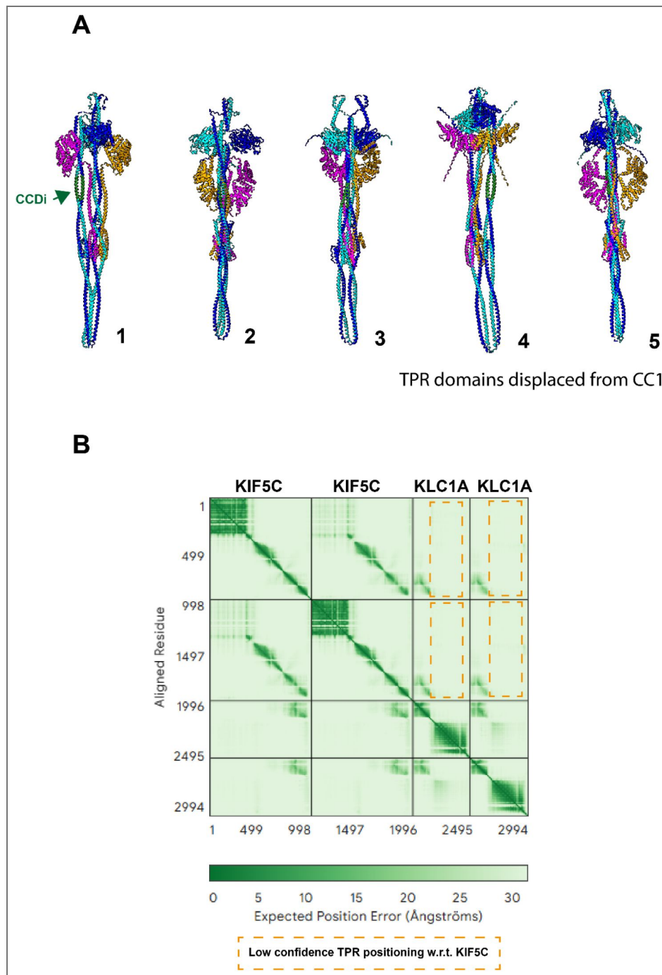
Figure S5. AlphaFold3 models of \Delta TDS kinesin-1 complexes.
