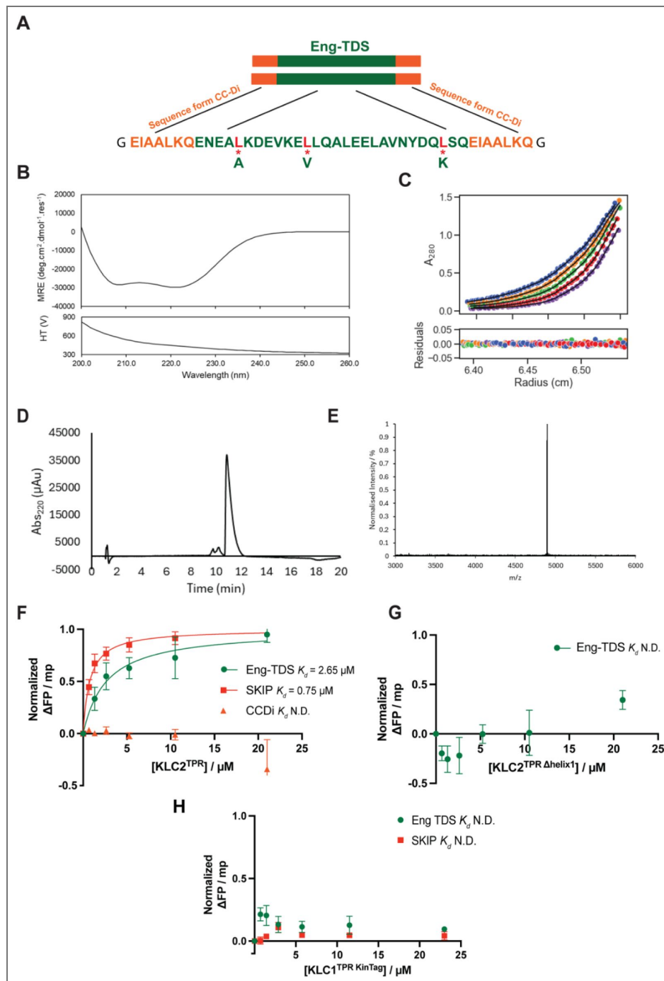
Figure S6. Eng-TDS design, characterisation and interaction with KLC.
