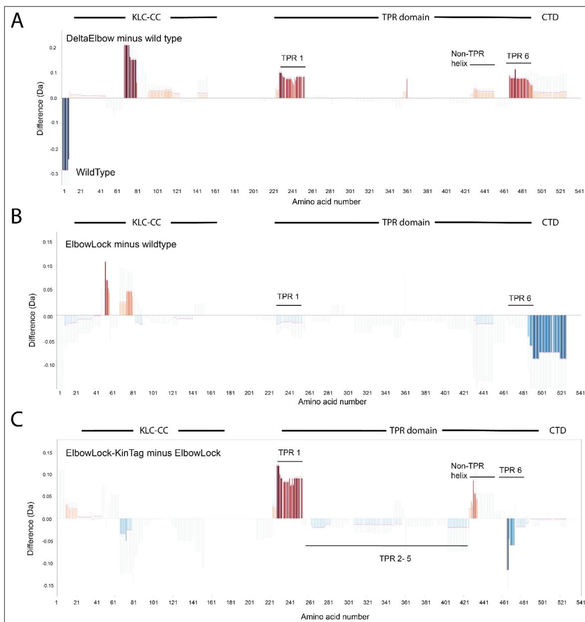
Figure S12. Difference plots showing total HDX across all timepoints comparing light chain of DeltaElbow and Elbowlock to wild type and ElbowLock-KinTag to ElbowLock.
