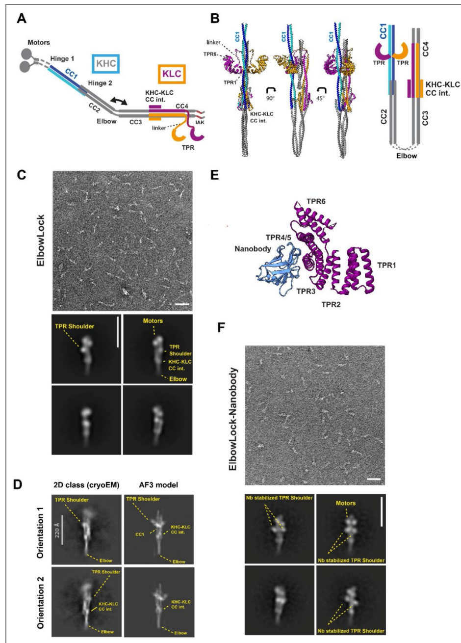
Figure 1. Computational modelling and single particle EM analysis identify a TPR docking site (TDS) on CC1
