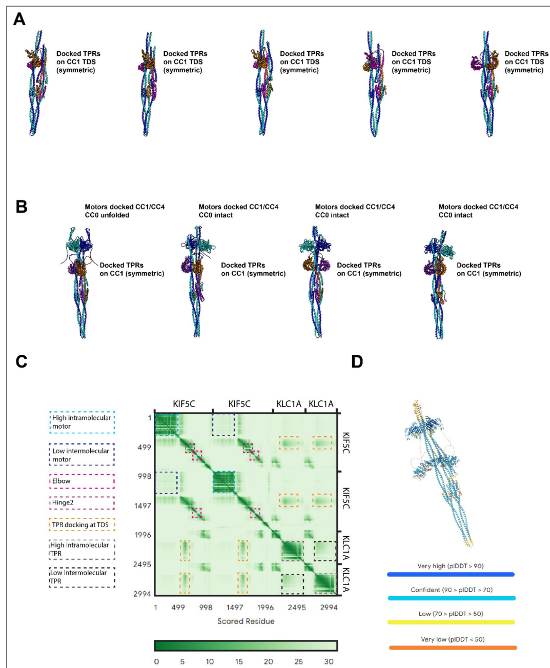
Figure S1. AlphaFold3 models of KHC-KLC complexes. (A) Models of kinesin-1 heterotetramer coiled-coil domains (KIF5C CC1-CC4; aa 410-917) with two KLCs (KLC1A CC-TPR; aa 1-480). (B) Models of complete full-length (KIF5C/KLC1A) kinesin-1 heterotetramers, including motor domains and C-terminal KLC sequences. (C) Representative predicted aligned error plot highlighting confidence in intra and inter domain interactions in a full length heterotetrameric model. (D) Representative model showing pLDDT. Plots are typical of other models.
