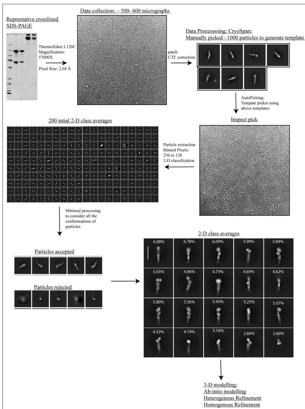
Figure S3. Representative NS-EM processing workflow.
