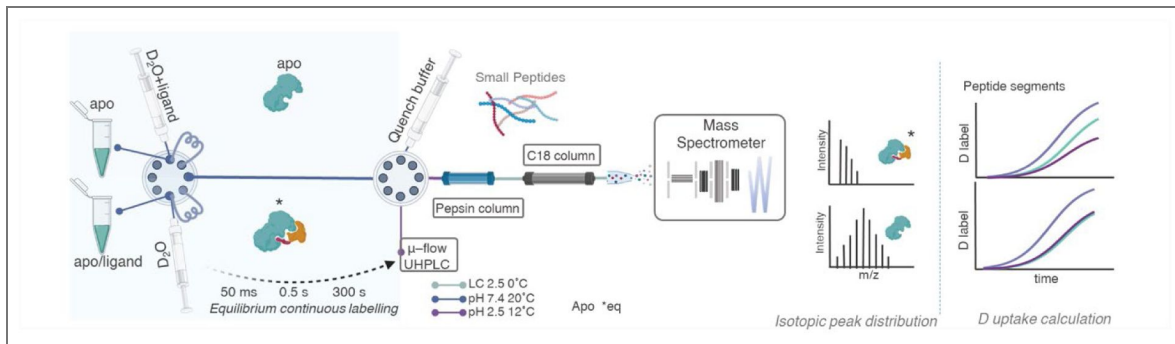
Figure S9. Schematic representation of the HDX experiment.
