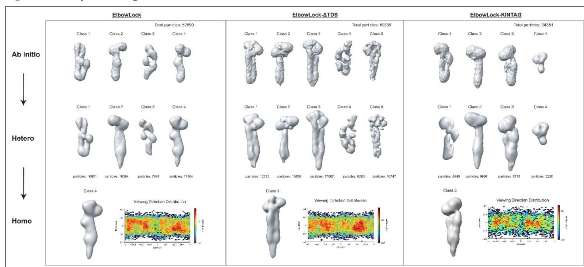
Figure S8. EM processing workflow for 3D reconstructions.
