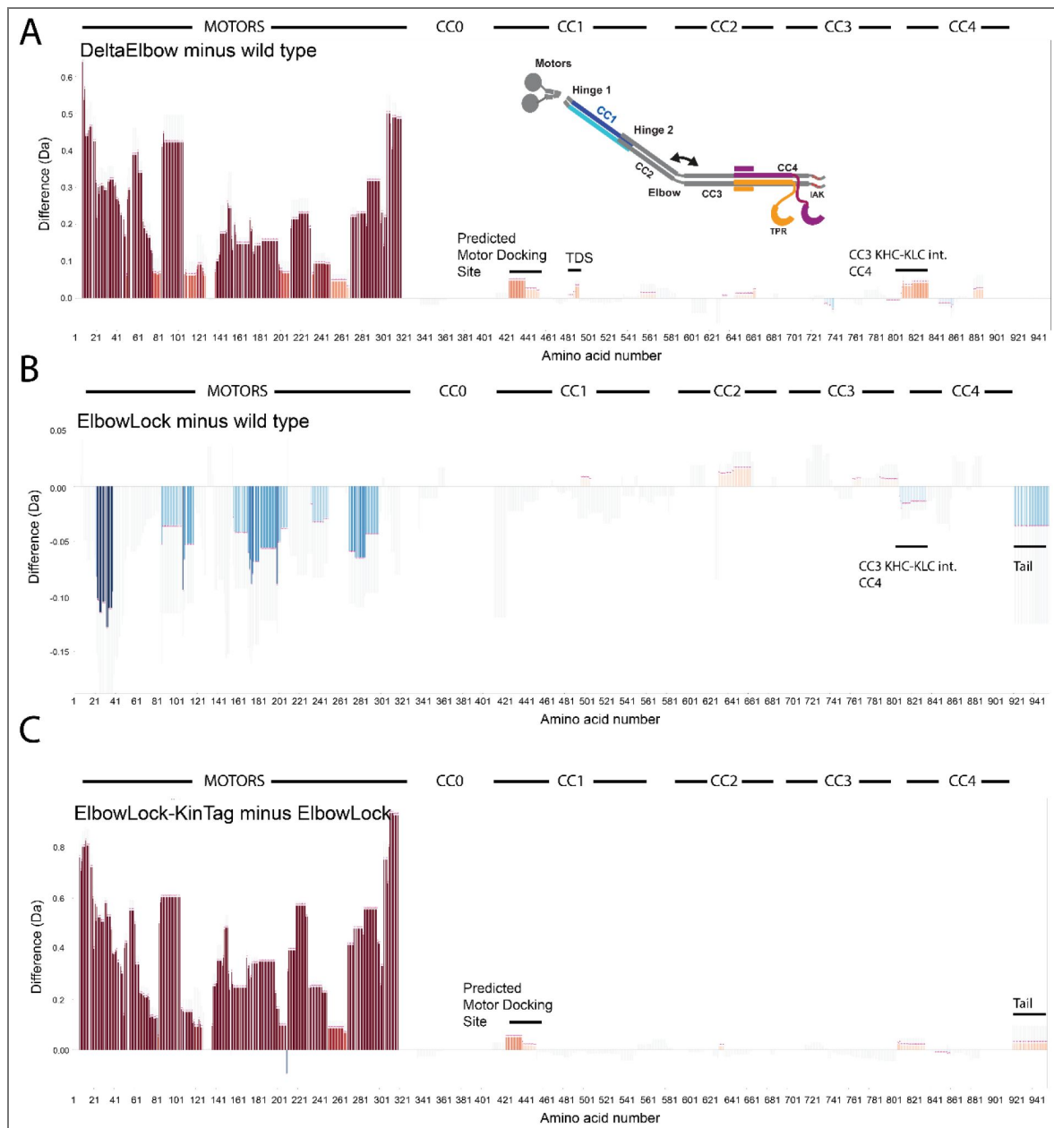
Figure S11. Difference plots showing total HDX across timepoints comparing heavy chain of DeltaElbow and Elbowlock to wild type and ElbowLock-KinTag to ElbowLock.
