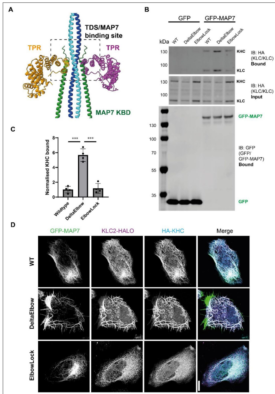
Figure 5. Opening the kinesin-1 complex promotes its association with MAP7.
