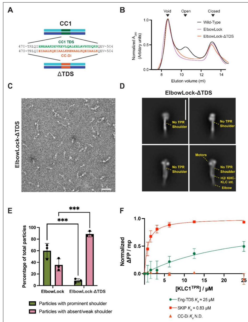
Figure 2. The CC1 TDS is required for the formation of the kinesin-1 shoulder.
