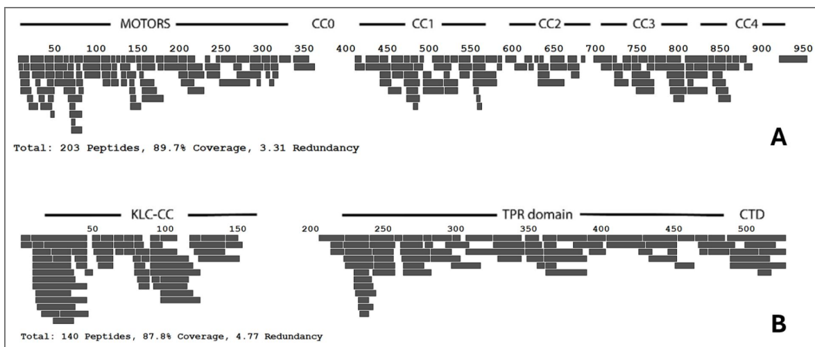
Figure S10. Coverage map of mass spectral assignment of peptides in 'bottom-up' HDX-MS experiments for kinesin-1 HC (A) and LC (B).
