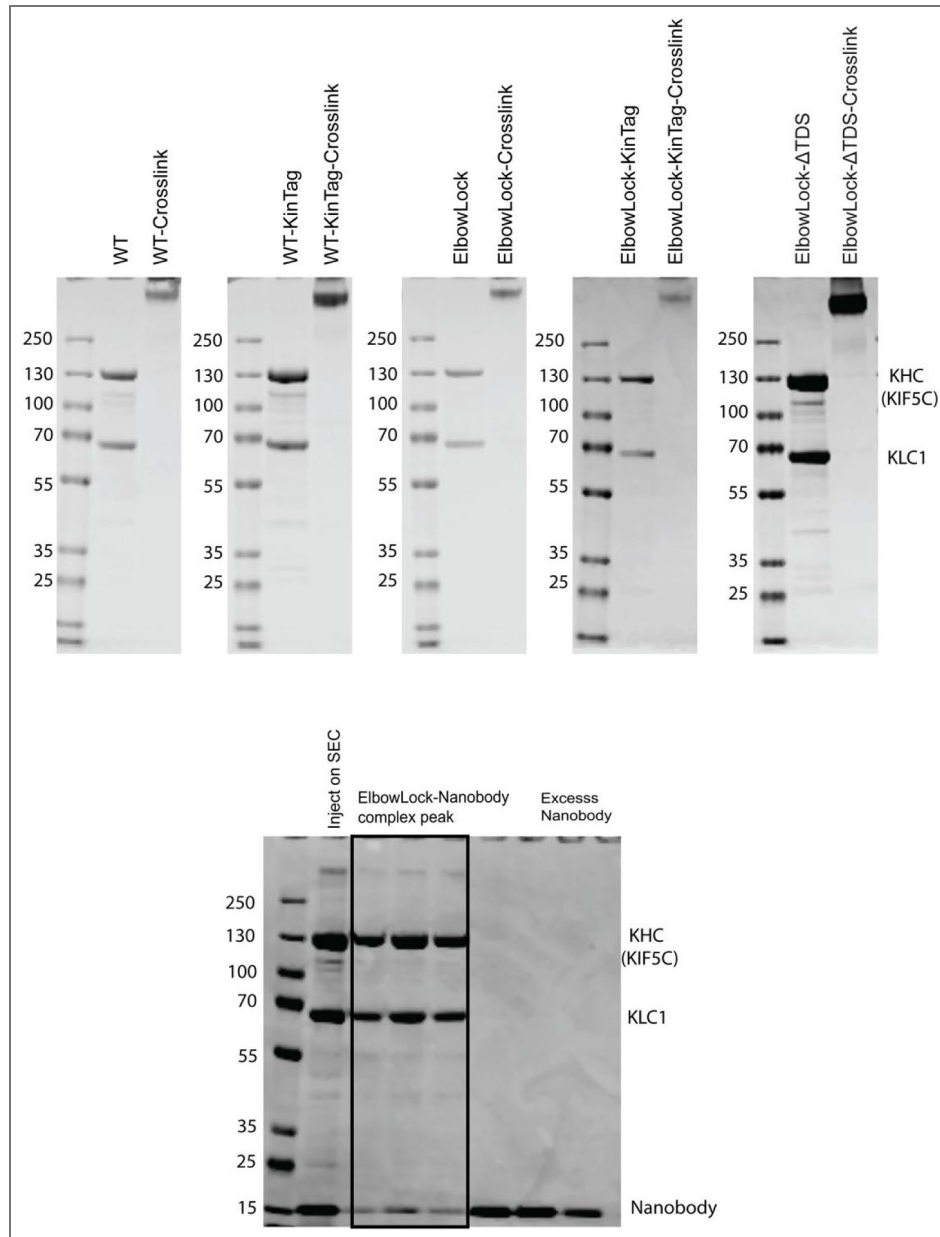
Figure S2. Representative samples of protein complexes used in this study.
