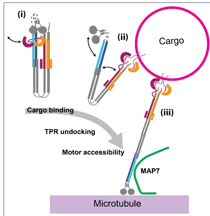
Figure 6. Model for cargo-mediated initiation of kinesin-1 activation.
