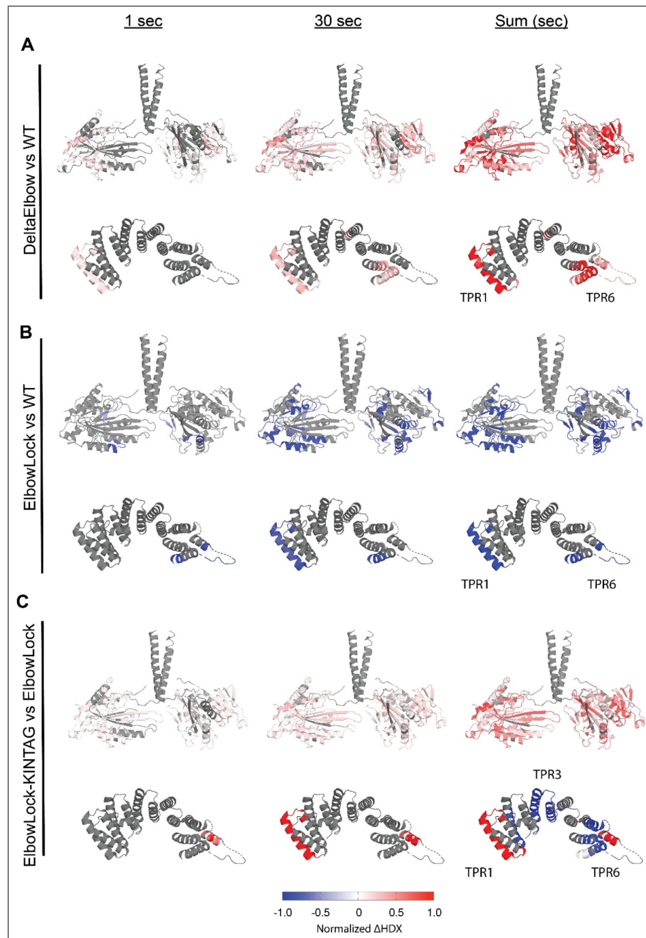
Figure 4. Adaptor-binding to the KLC TPR domain promotes motor accessibility.
