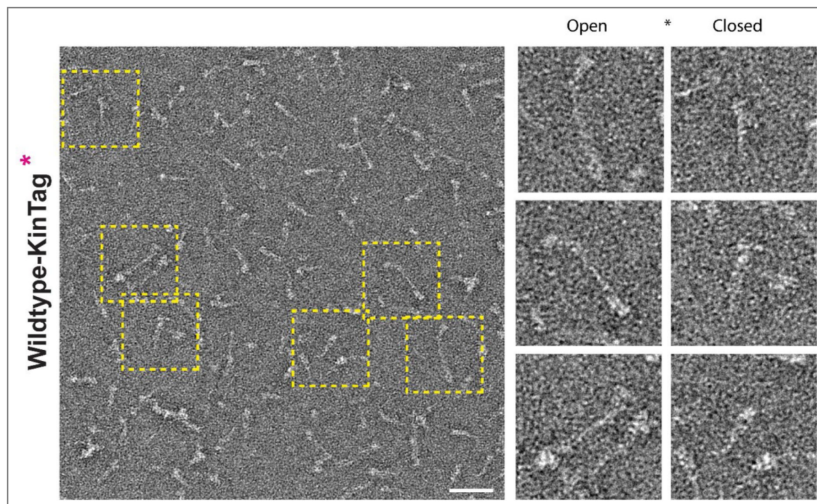
Figure S7. Representative NS-EM electron micrograph showing wild type-KinTag particles with selected open and close particles expanded on right.
