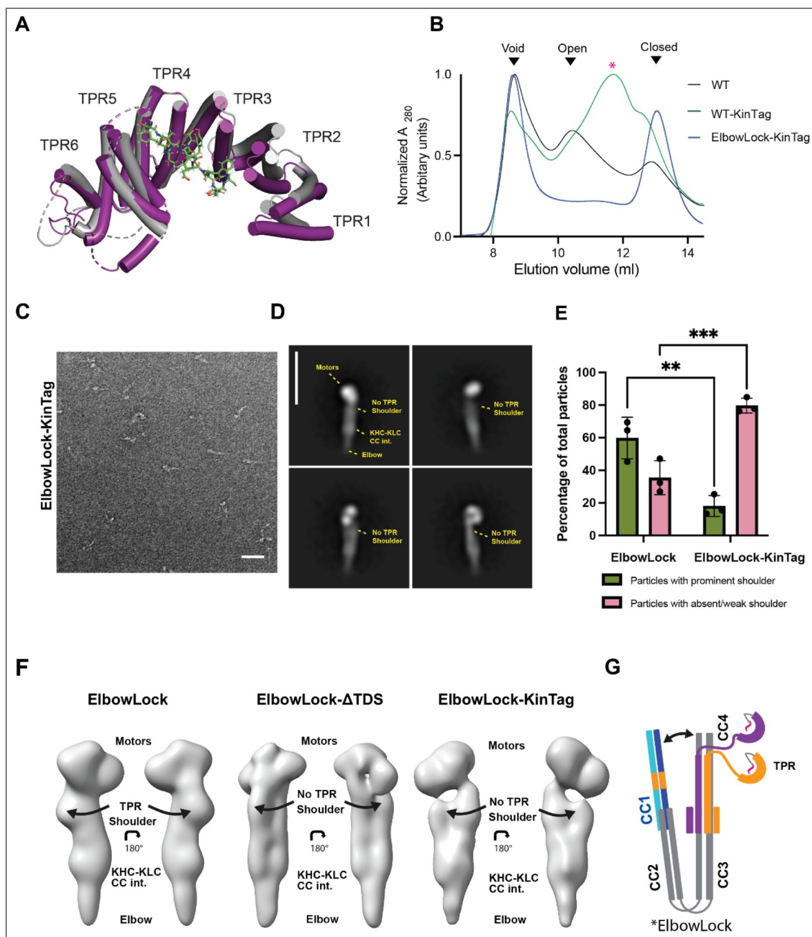
Figure 3. Adaptor-binding to KLC-TPR dislocates the kinesin-1 shoulder.
