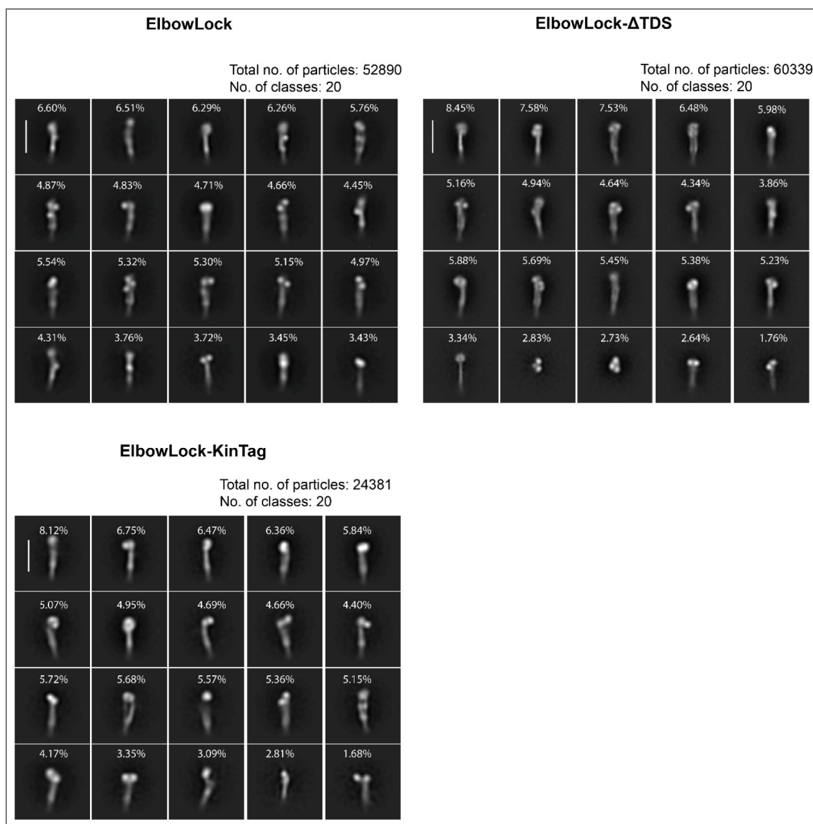
Figure S4. Representative sets of 2D classes for all complexes.
