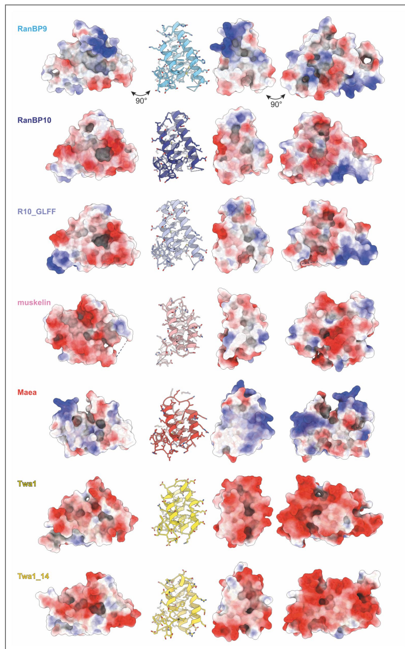
Suppl. Fig. 12. Electrostatic surface representation of CTLH-CRA domains used in this study.
