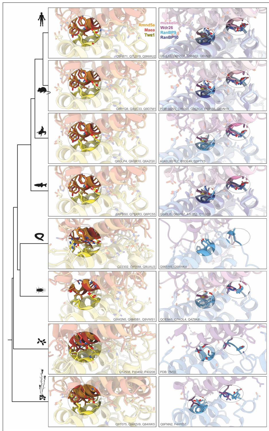
Suppl. Fig. 9. Overlay of AlphaFold3-predicted CTLH-CRA interfaces across species.
