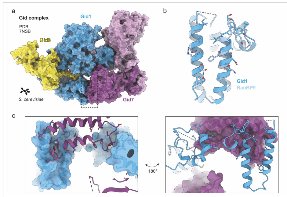
Suppl. Fig. 10. CTLH-CRA interface of the yeast Gid1-Gid7.
