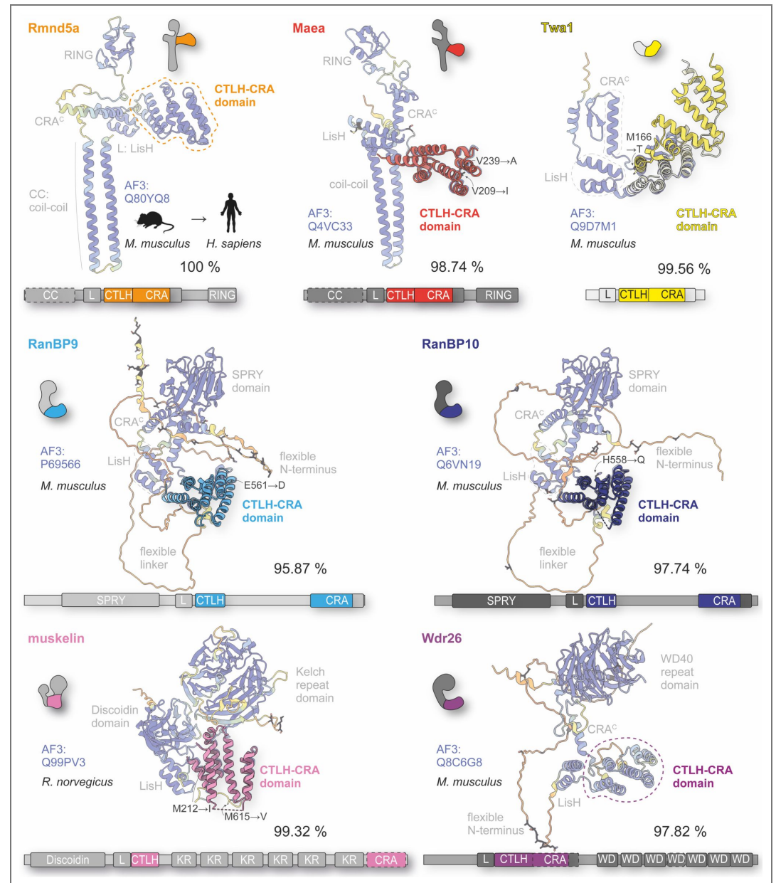
Suppl. Fig. 1. Conservation of mammalian core CTLH complex subunits. Overlay of the experimentally determined CTLH-CRA domain structures (PDB: 9SNH, 9SNI, 9SNE, 9SNF, and 9SNV) with full-length AlphaFold predictions (Varadi et al., 2024) of the proteins used in this study (mouse; rat muskelin). Sequence differences between the murine or rat proteins and their human counterparts are shown in black, and variations located within the CTLH-CRA domains are explicitly indicated at the respective positions in the structures. Percent sequence identity to the human proteins is provided. The overlay demonstrates that the truncated and fused CTLH-CRA constructs accurately reflect the structural context of the full-length proteins and highlights the high conservation of these mammalian subunits.
