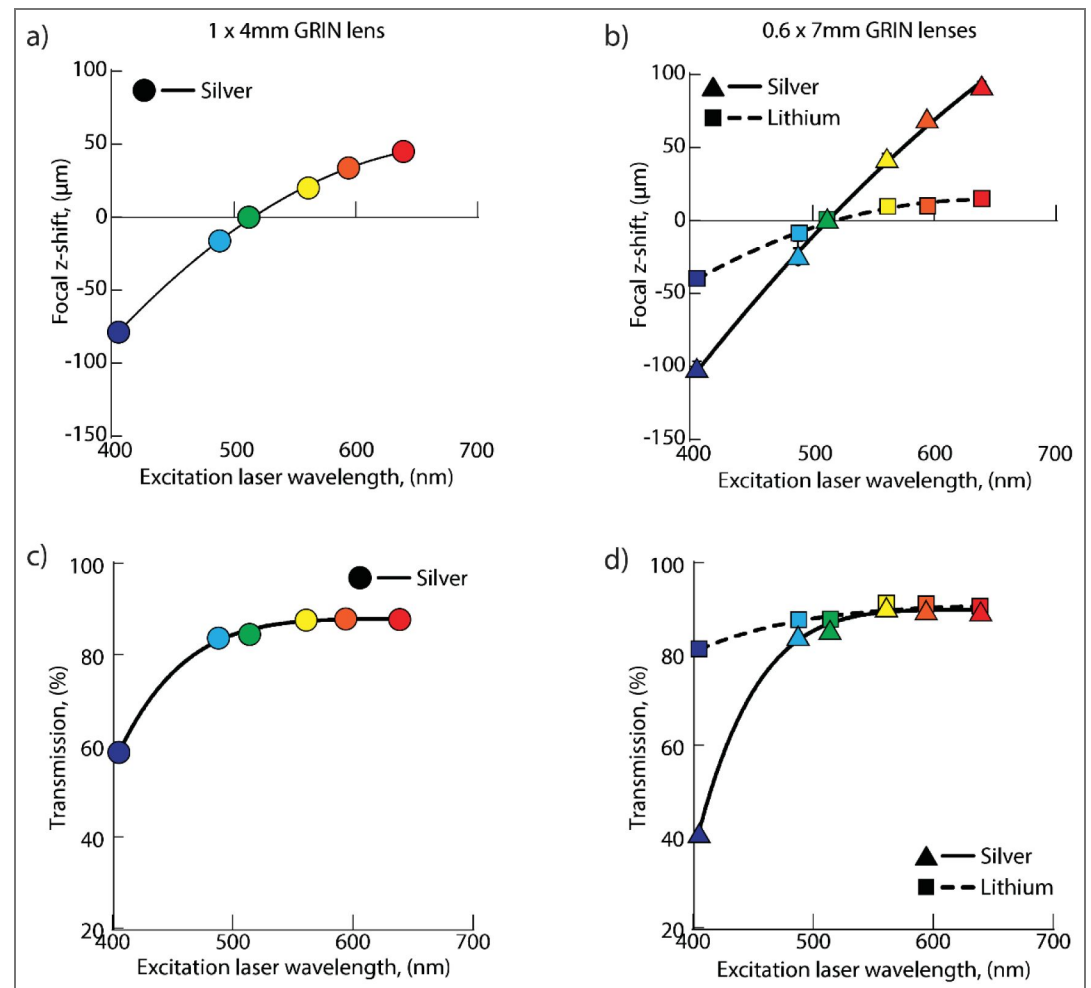
Figure 2 - Figure Supplement 1. Comparison of aberrations across GRIN lens types: Comparison of aberrations across GRIN lens types a, Shift in z-focal plane as a function of excitation laser wavelength in a 1×4 mm silver-doped GRIN lens. Second-order polynomial R^2 = 0.9970 . b, Shift in z-focal plane as a function of excitation laser wavelength in 0.6×7 mm GRIN lenses doped with either silver or lithium. Second-order polynomials: Silver R^2 = 0.9983 , Lithium R^2 = 0.9928 . c, Percent transmission through a 1×4 mm silver-doped GRIN
