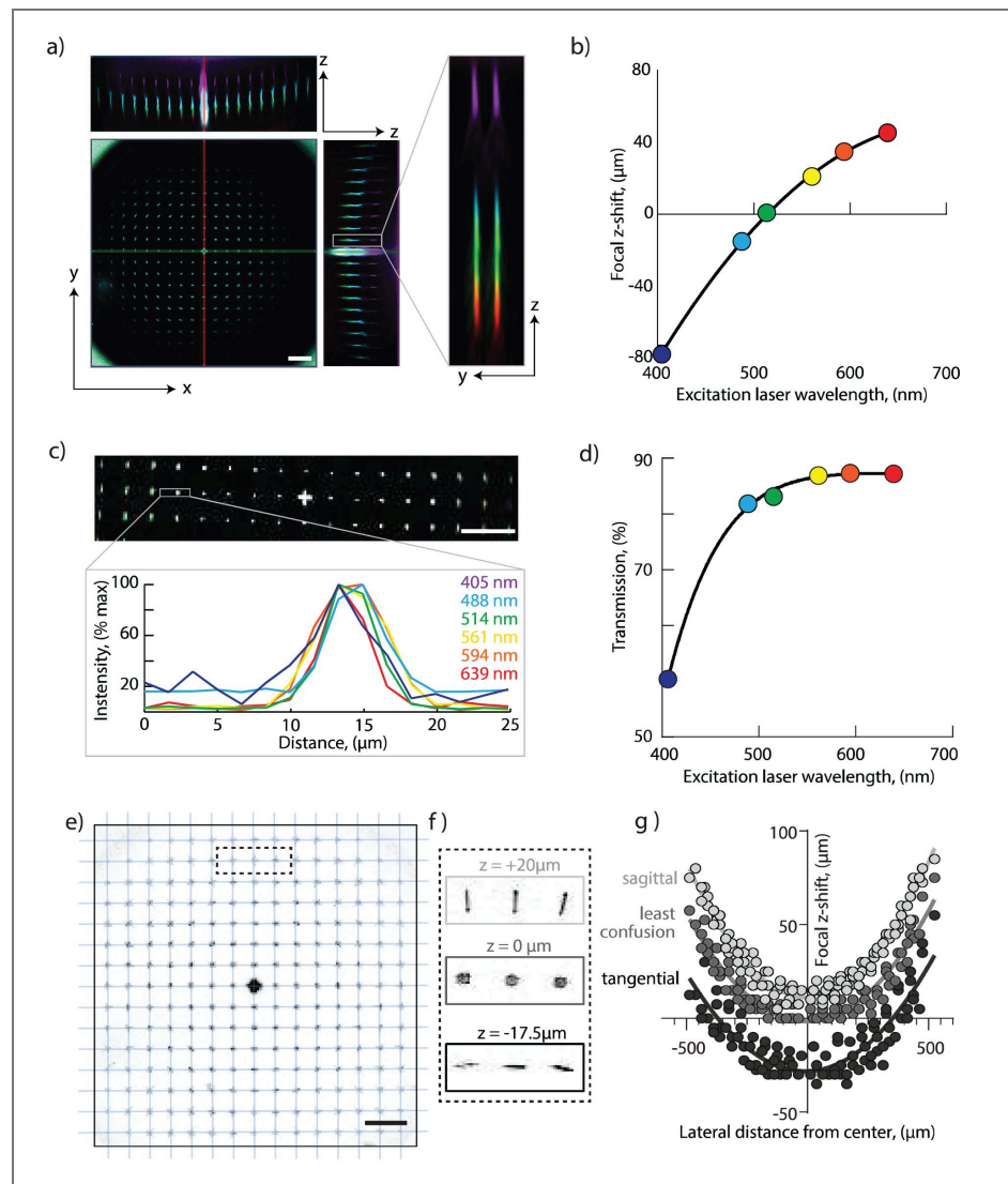
Figure 2. GRIN lens induced chromatic aberrations
