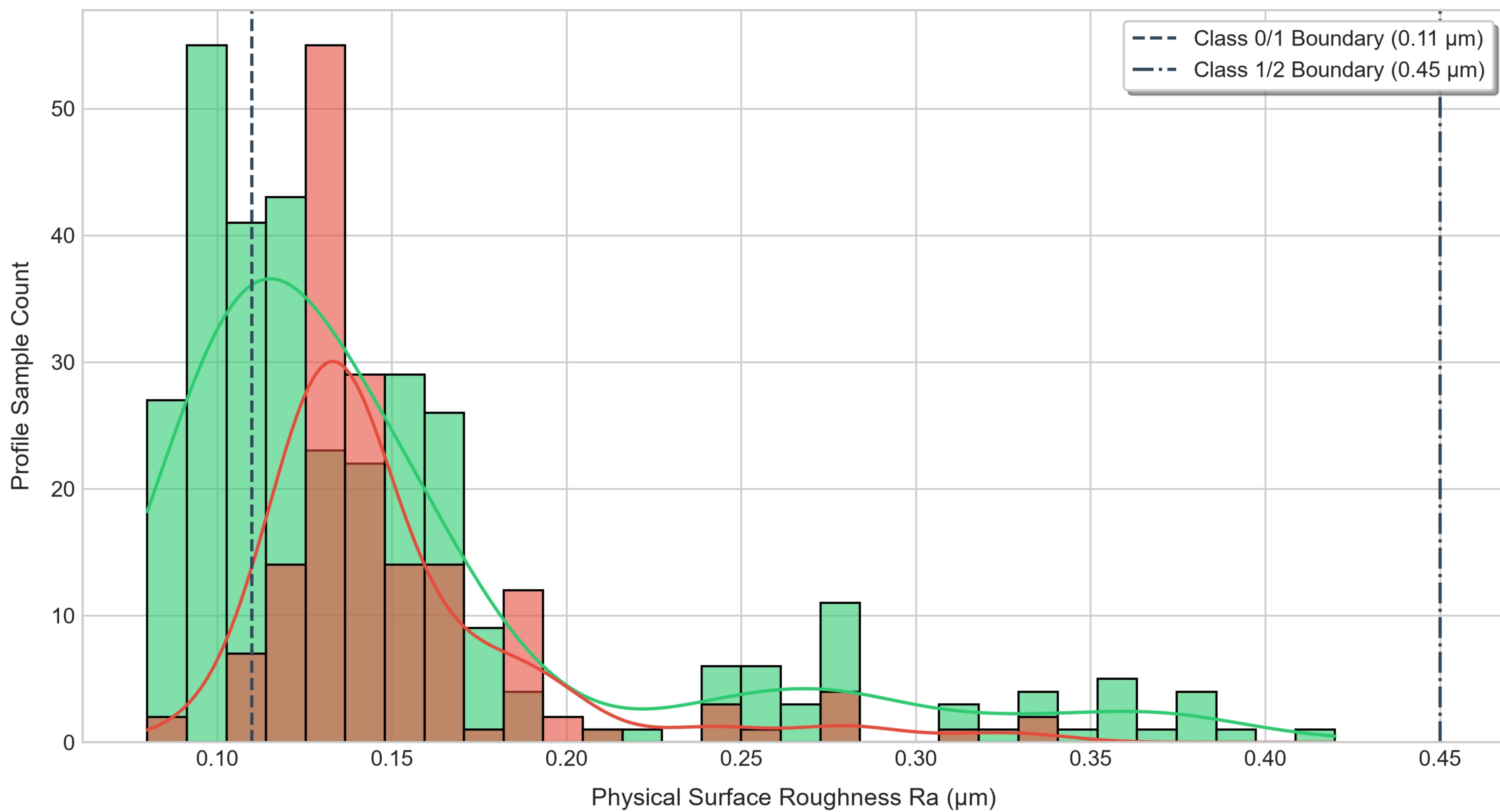
Specimen Distance to Decision Boundaries (0.11 \mu\text{m} & 0.45 \mu\text{m} Limit Zones)
