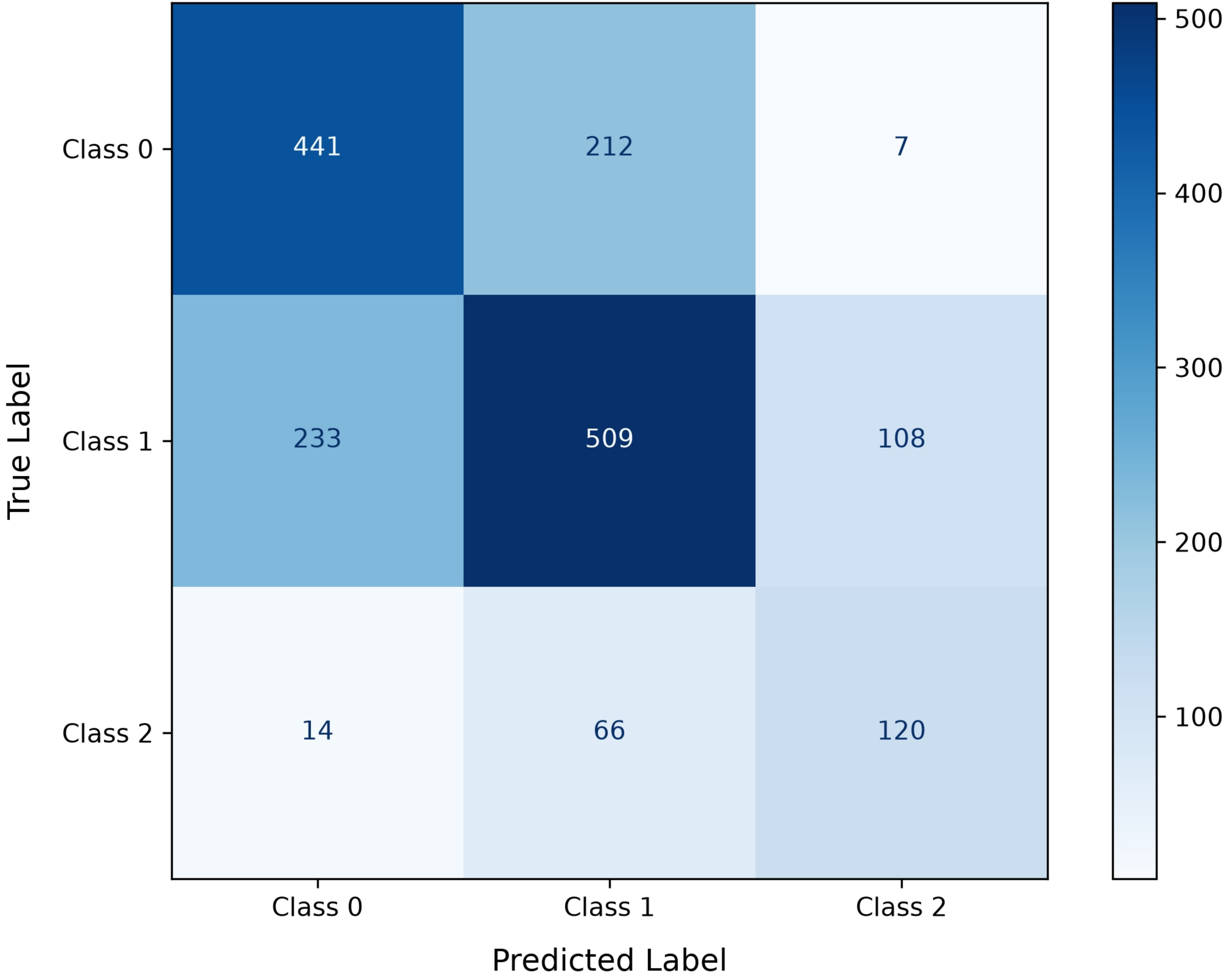
C4.5 Unpruned Model - Confusion Matrix
