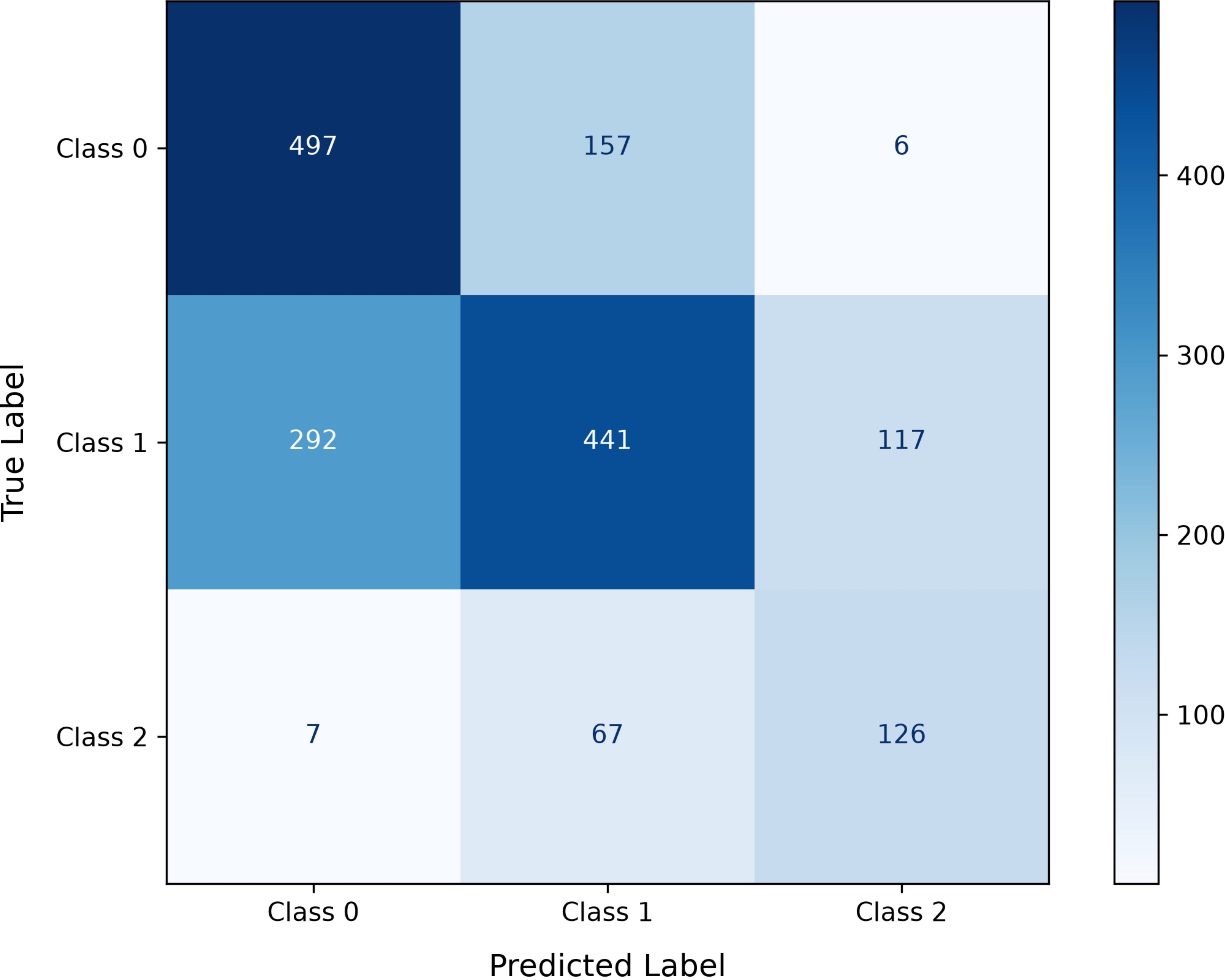
C4.5 Pruned (J48) Model - Confusion Matrix
