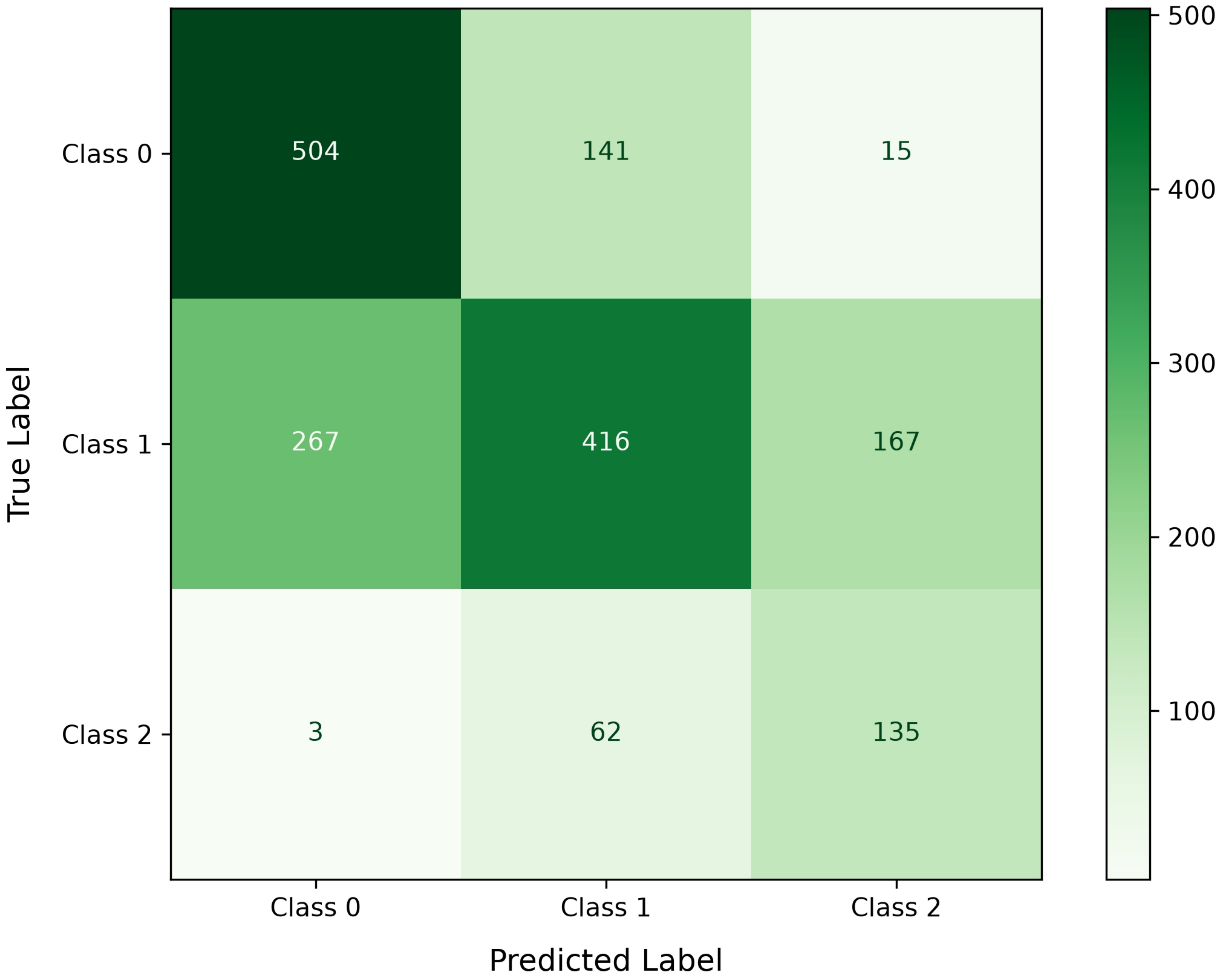
Gini CART Pruned Model - Confusion Matrix
