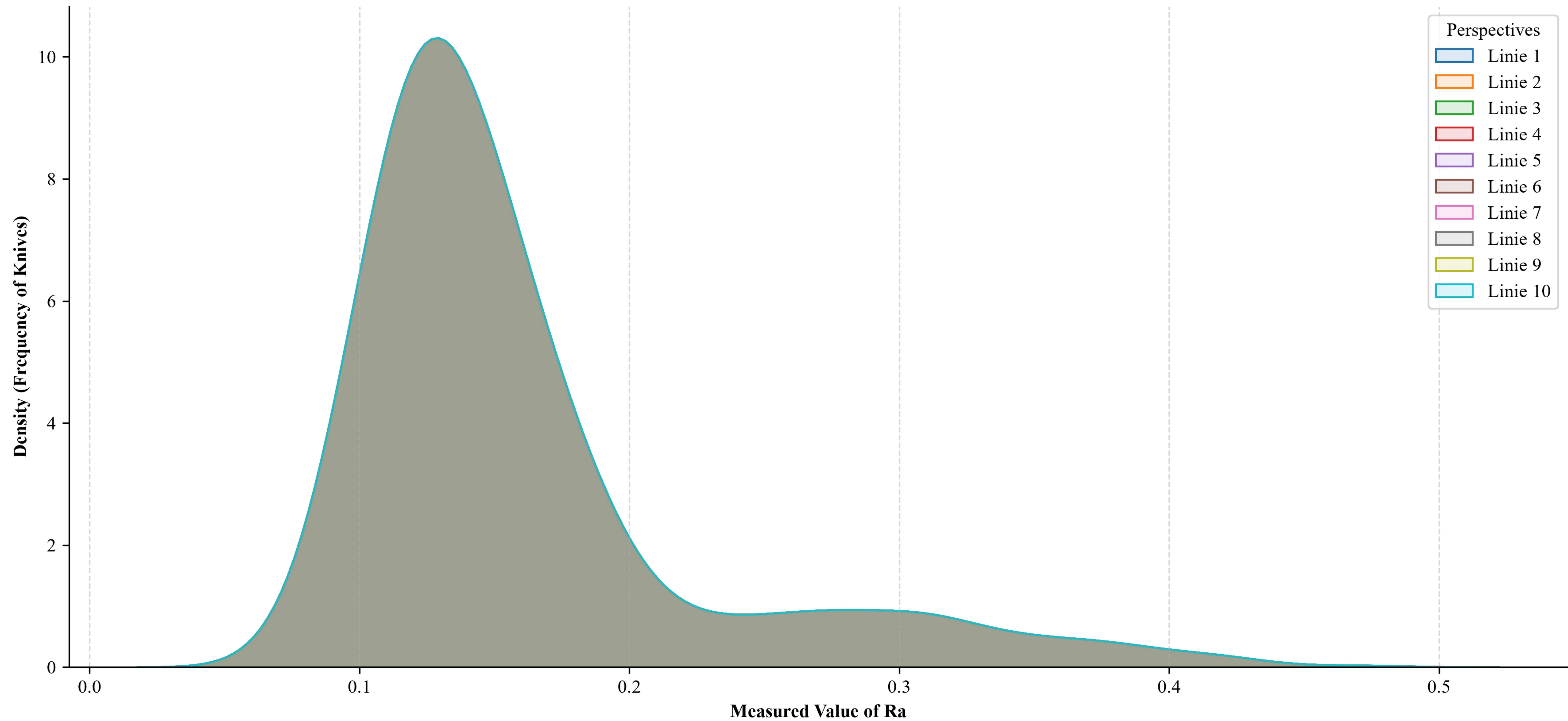
Surface Parameter 'Ra' Distribution Across Measurement Perspectives
