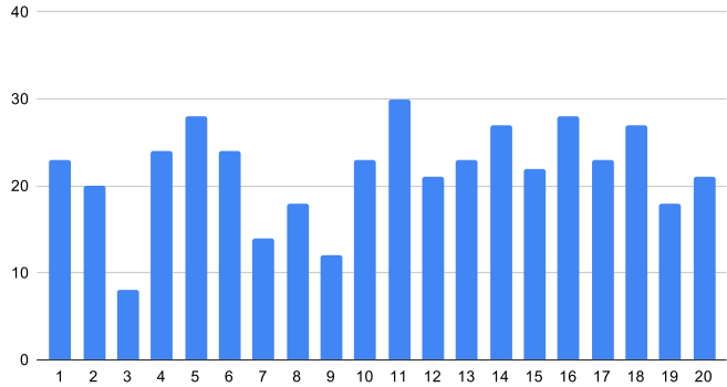
Position ve Phred Score
