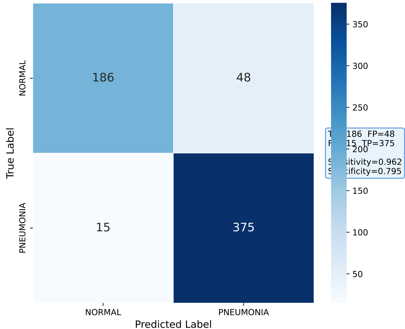
EfficientNetB0 — Confusion Matrix (Test)
