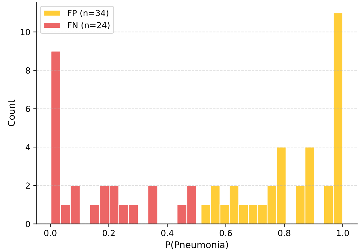
ResNet50
