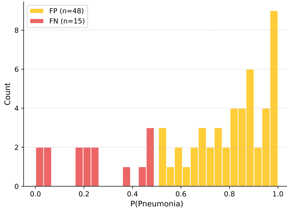
EfficientNetB0
