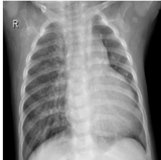
FN | conf=0.141
