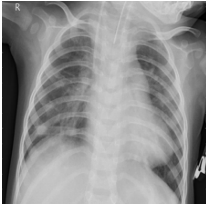
FN | conf=0.073
