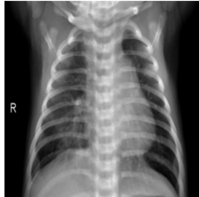
FN | conf=0.173
