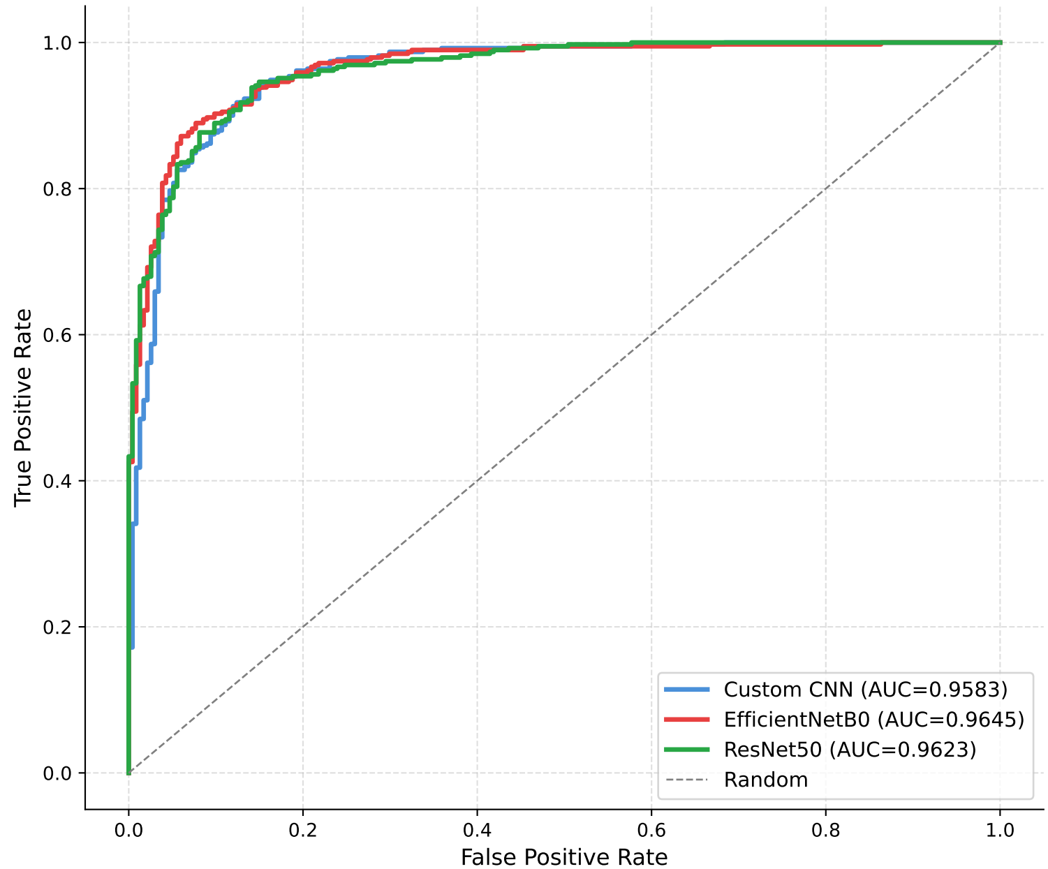
ROC Curves — All Models (Test Set)
