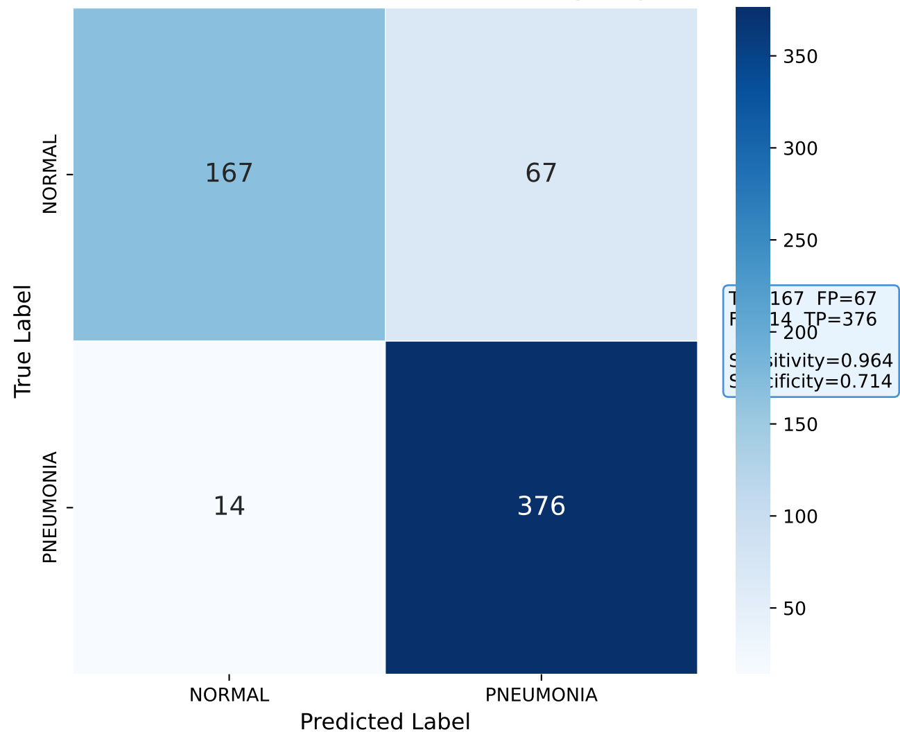
Custom CNN — Confusion Matrix (Test)
