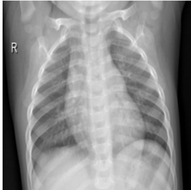
FN | conf=0.157
