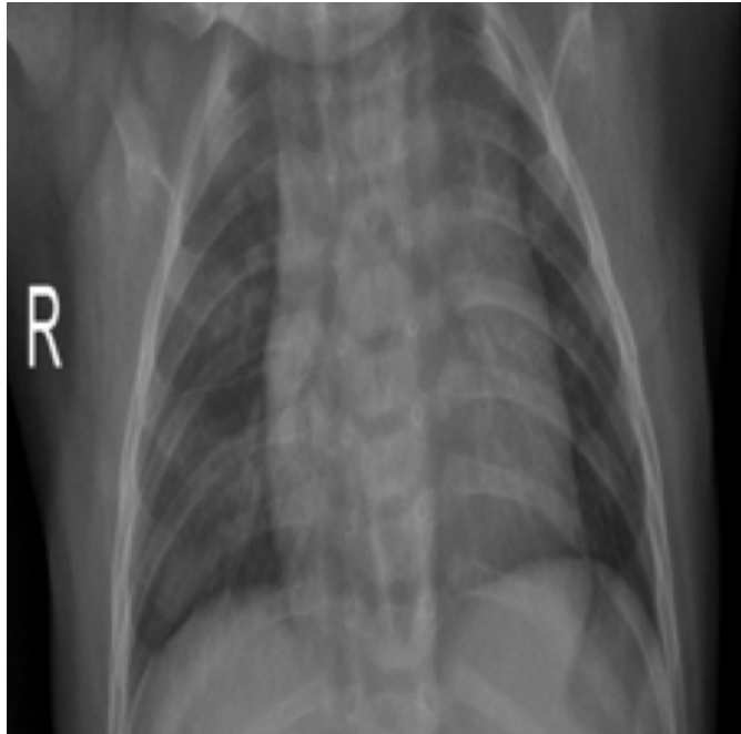
FN | conf=0.078
