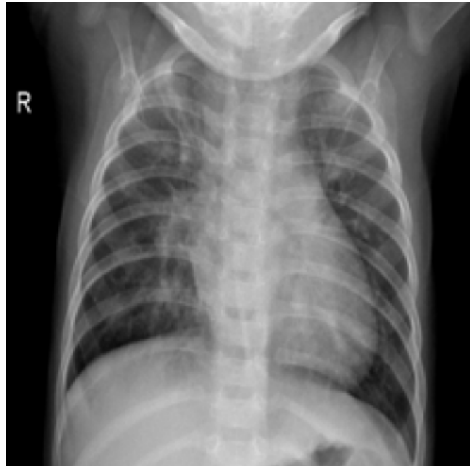
FN | conf=0.148
