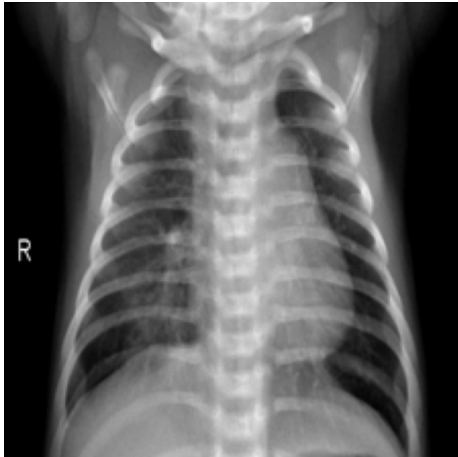
FN | conf=0.266
