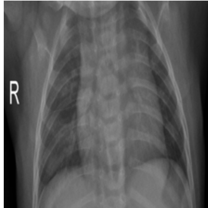
FN | conf=0.412
