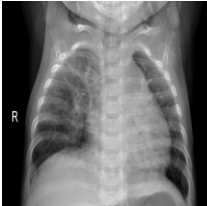
FN | conf=0.414
