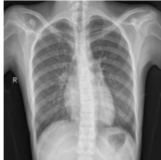
FN | conf=0.047
