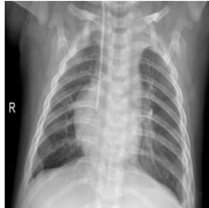
FN | conf=0.032
