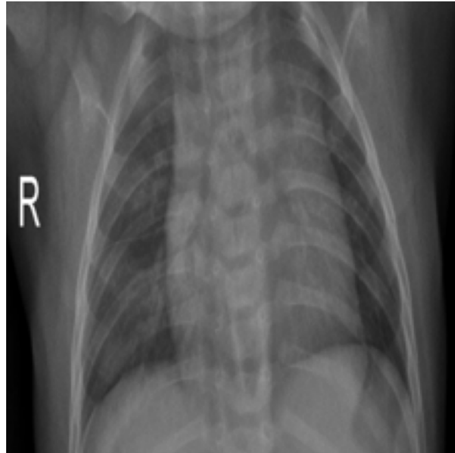
FN | conf=0.174
