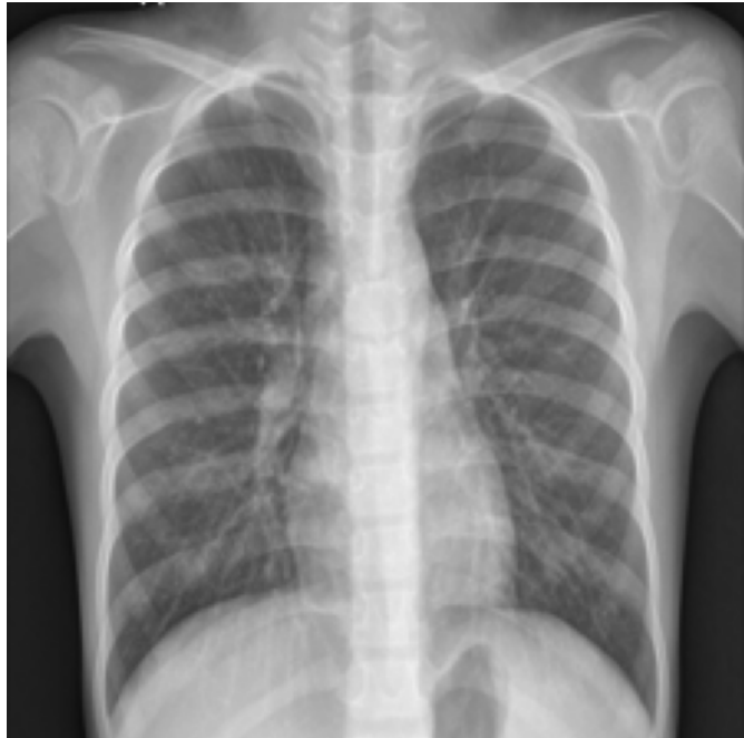
FN | conf=0.070
