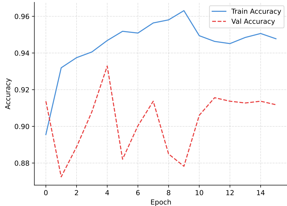
Accuracy
