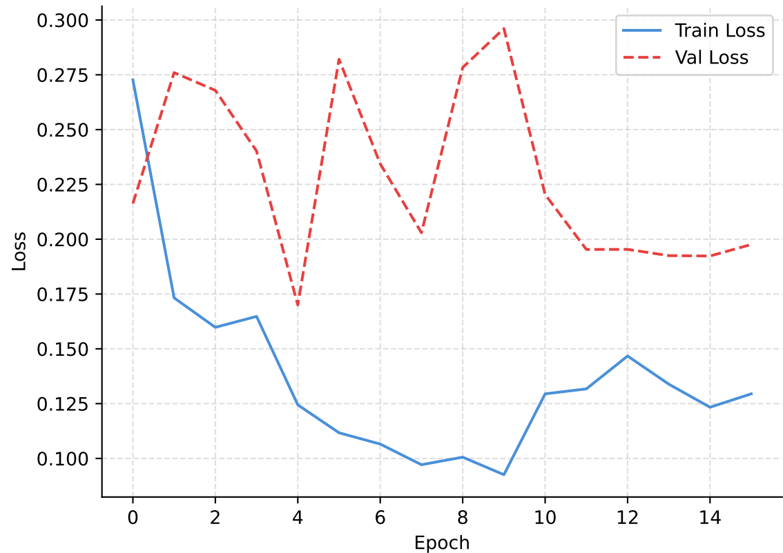
Loss
