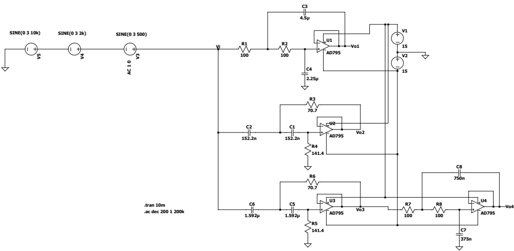
2nd order low pass Butterworth filter for 500Hz
