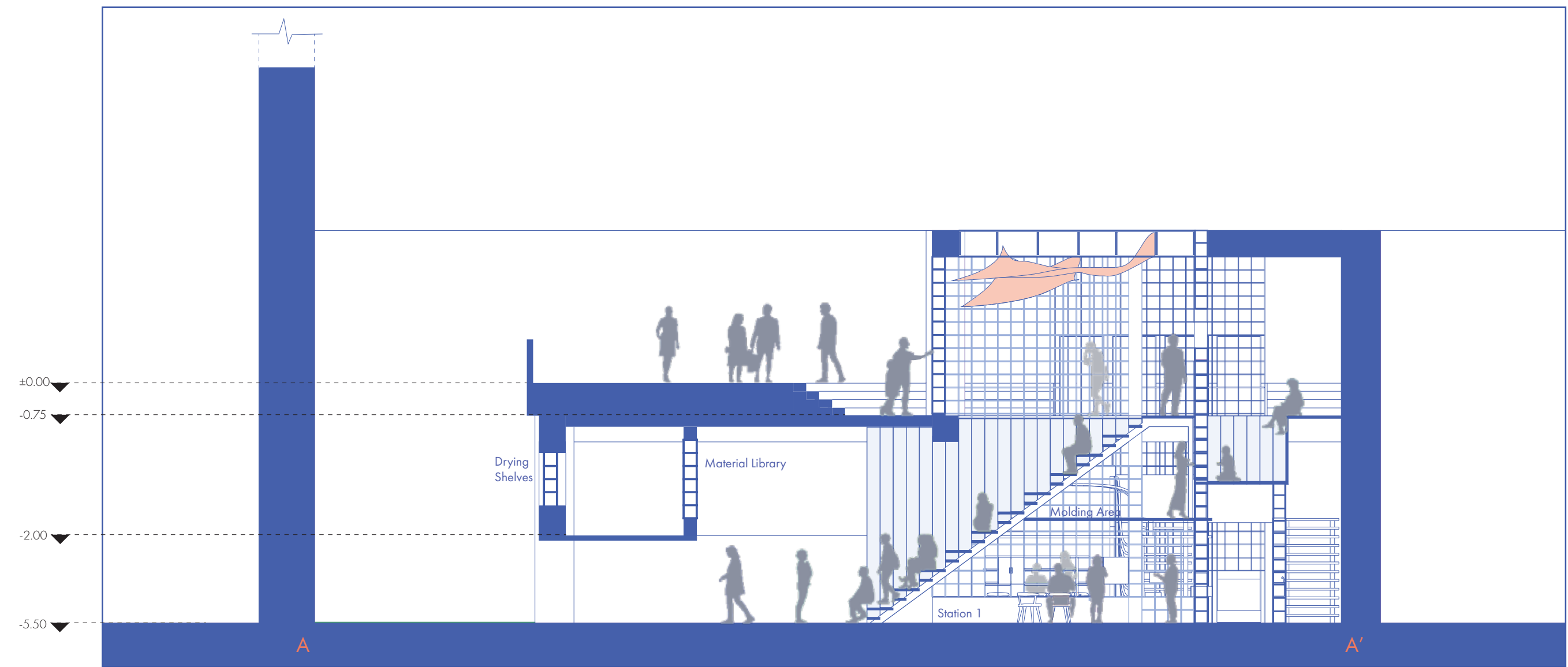
AA' Section 1/100
