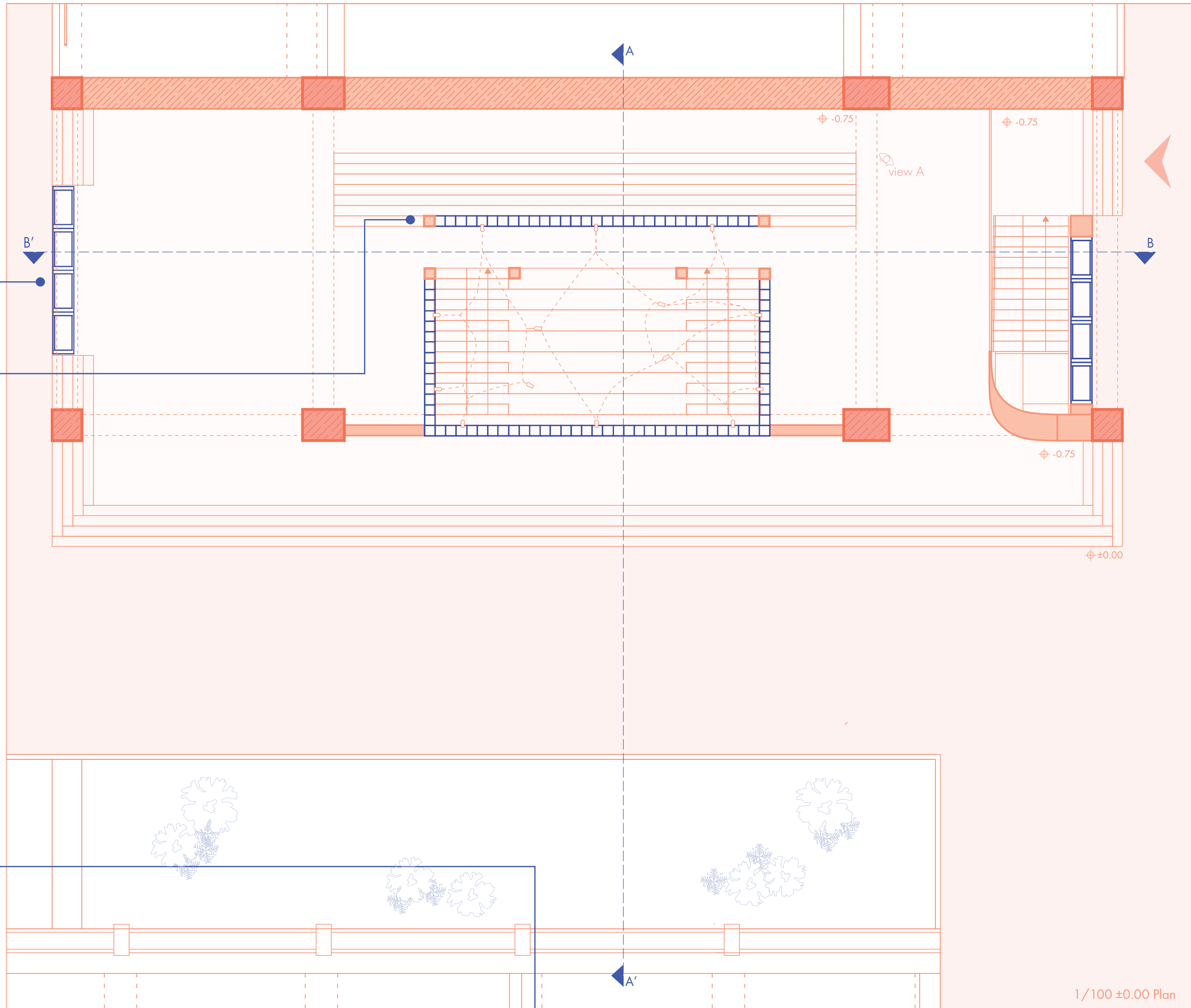
1/100 ±0.00 Plan
