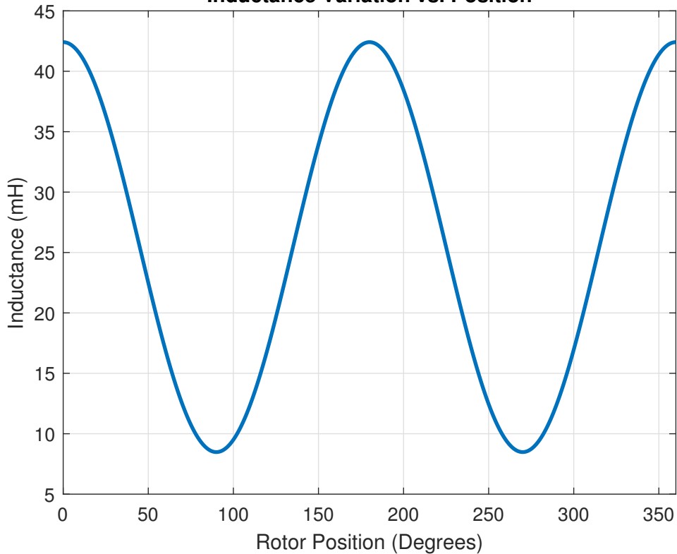
Inductance Variation vs. Position
