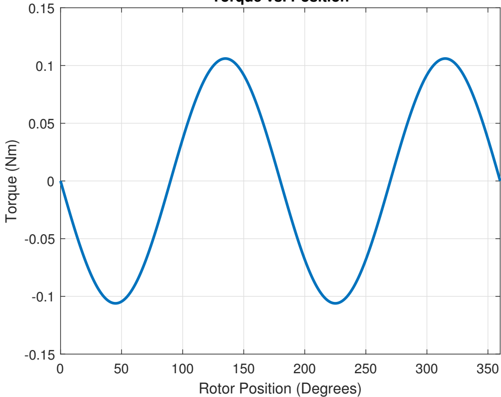
Torque vs. Position
