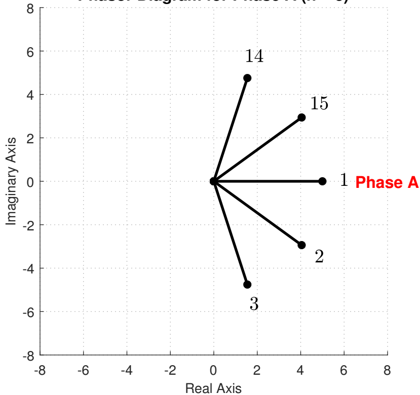
Phasor Diagram for Phase A ( n = 3 )
