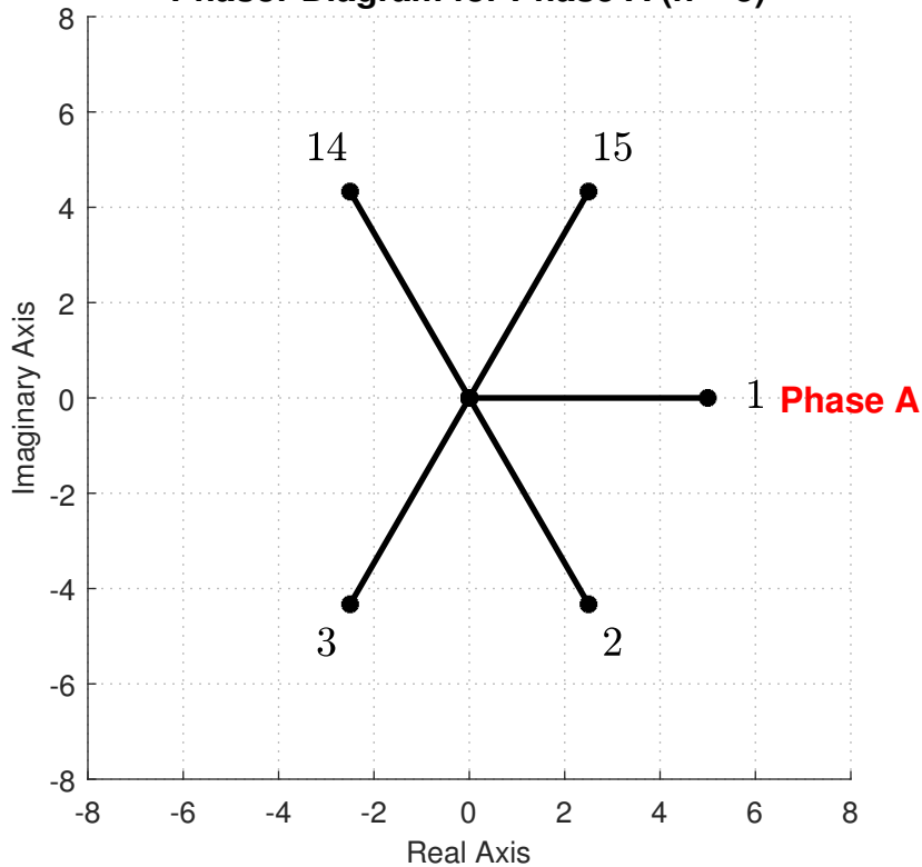
Phasor Diagram for Phase A ( n = 5 )
