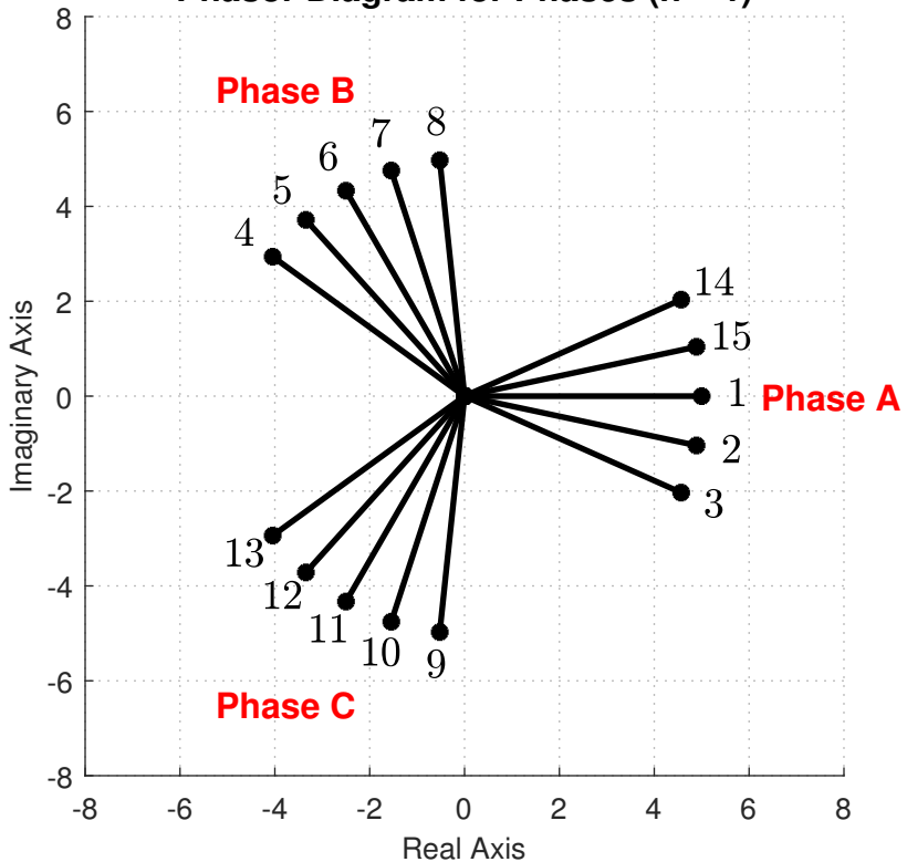
Phasor Diagram for Phases (n = 1)
