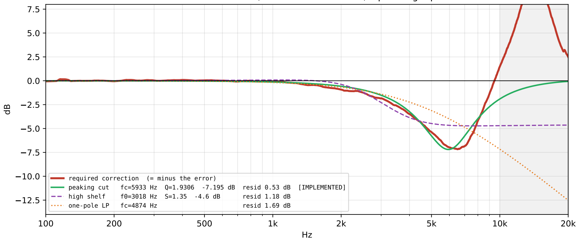
Candidate corrective filters, fitted 300 Hz - 10 kHz, equal weight per octave
