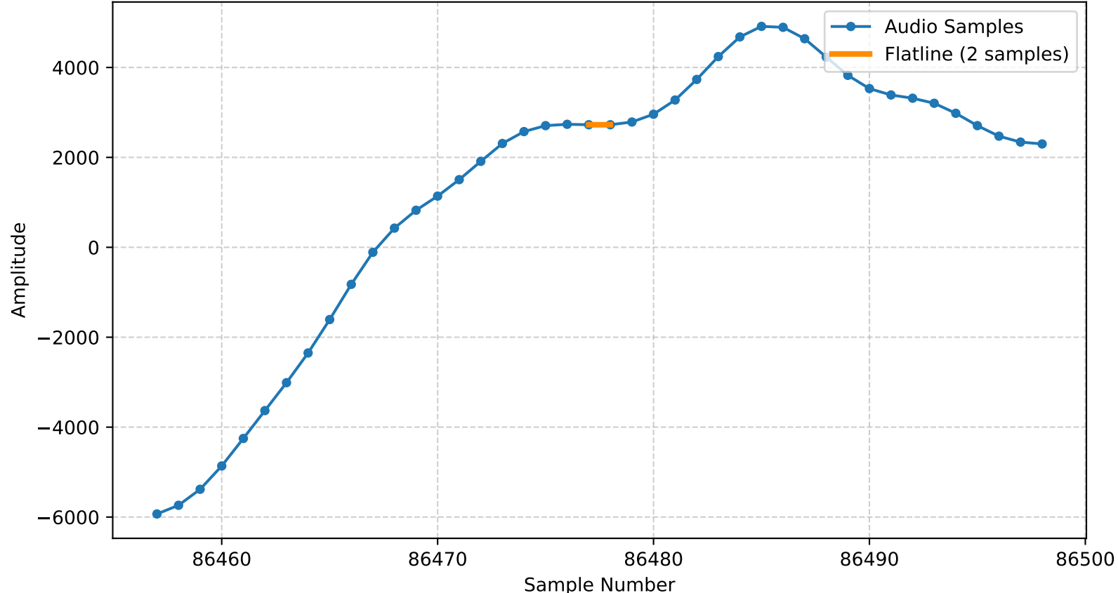
Flatline (2 samples) at Sample 86477 | Channel 1 | Sample Value: 2726.00
