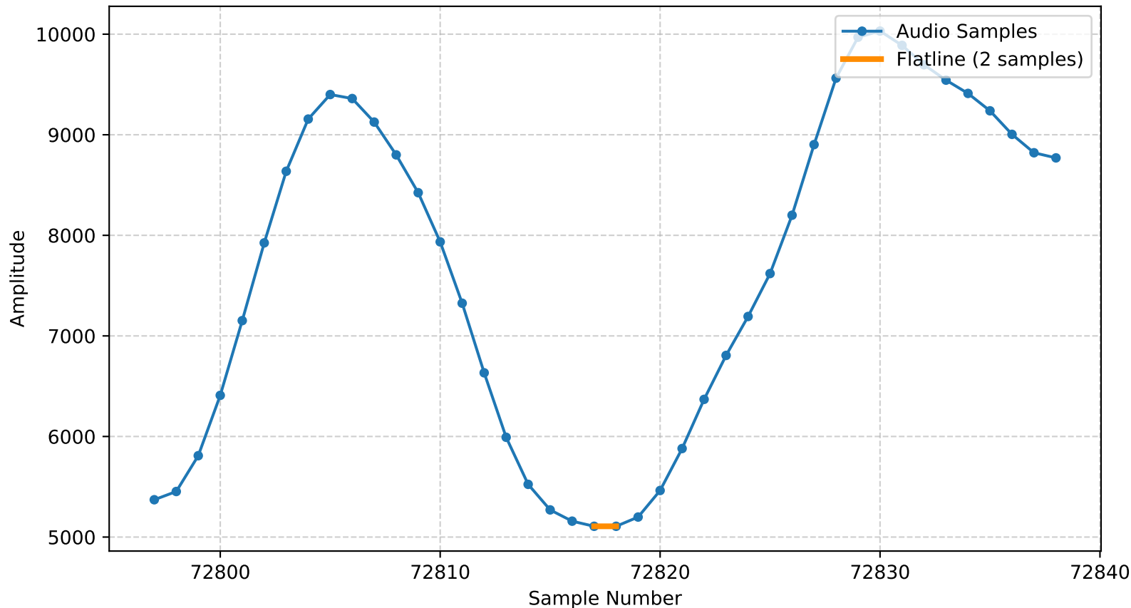
Flatline (2 samples) at Sample 72817 | Channel 1 | Sample Value: 5107.00
