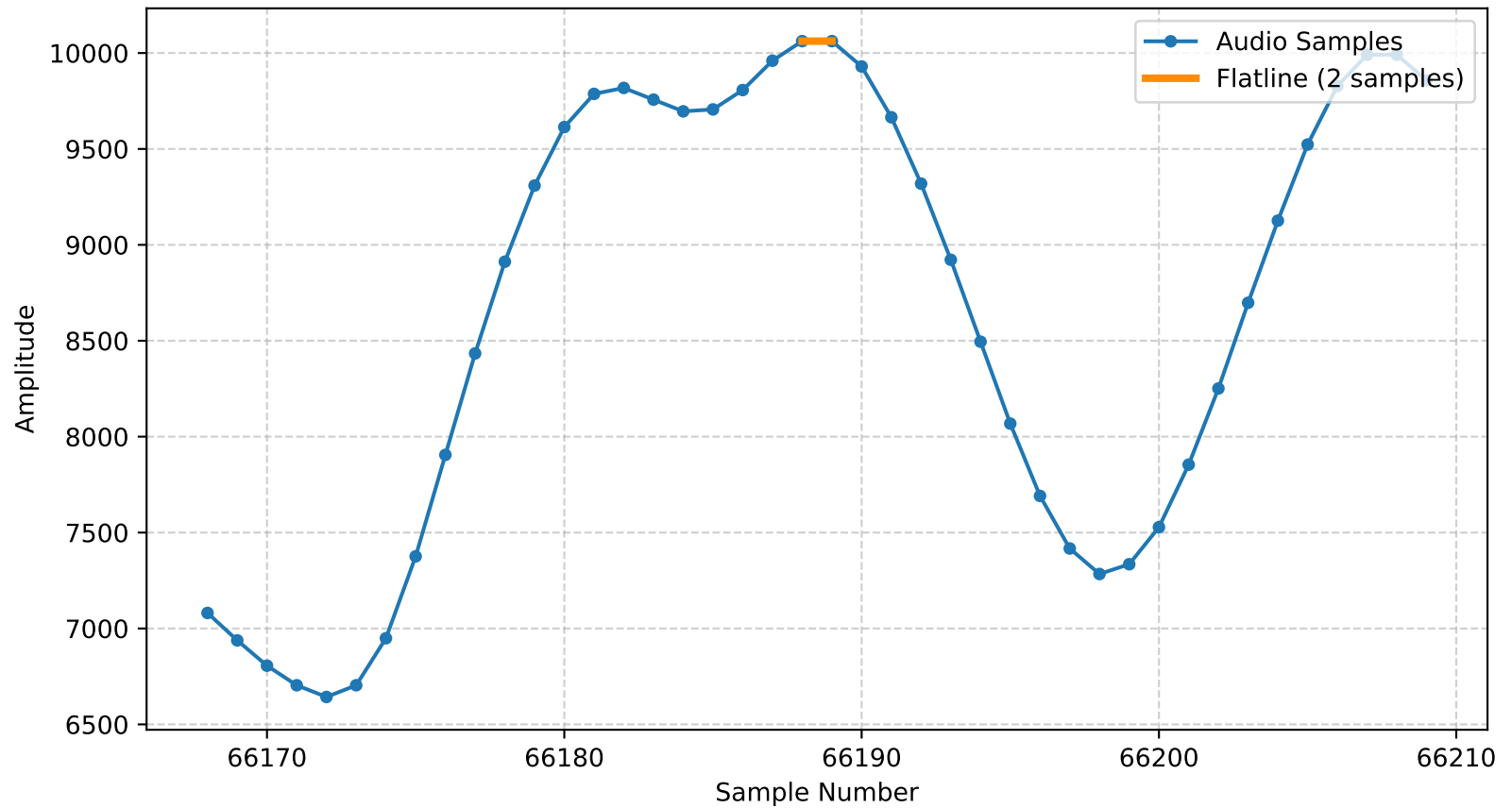
Flatline (2 samples) at Sample 66188 | Channel 1 | Sample Value: 10062.00
