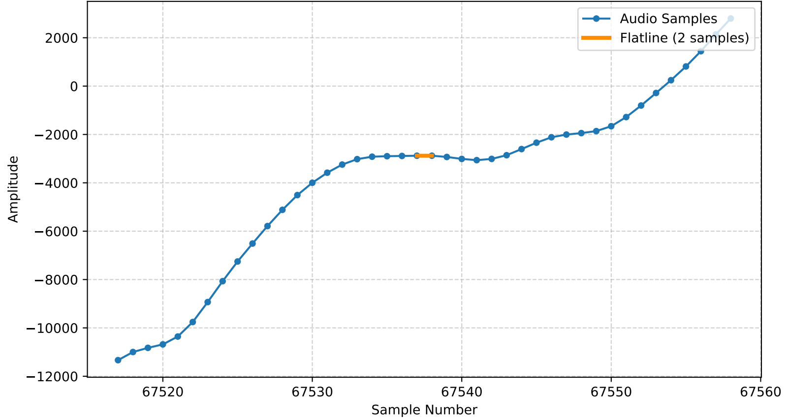
Flatline (2 samples) at Sample 67537 | Channel 1 | Sample Value: -2879.00
