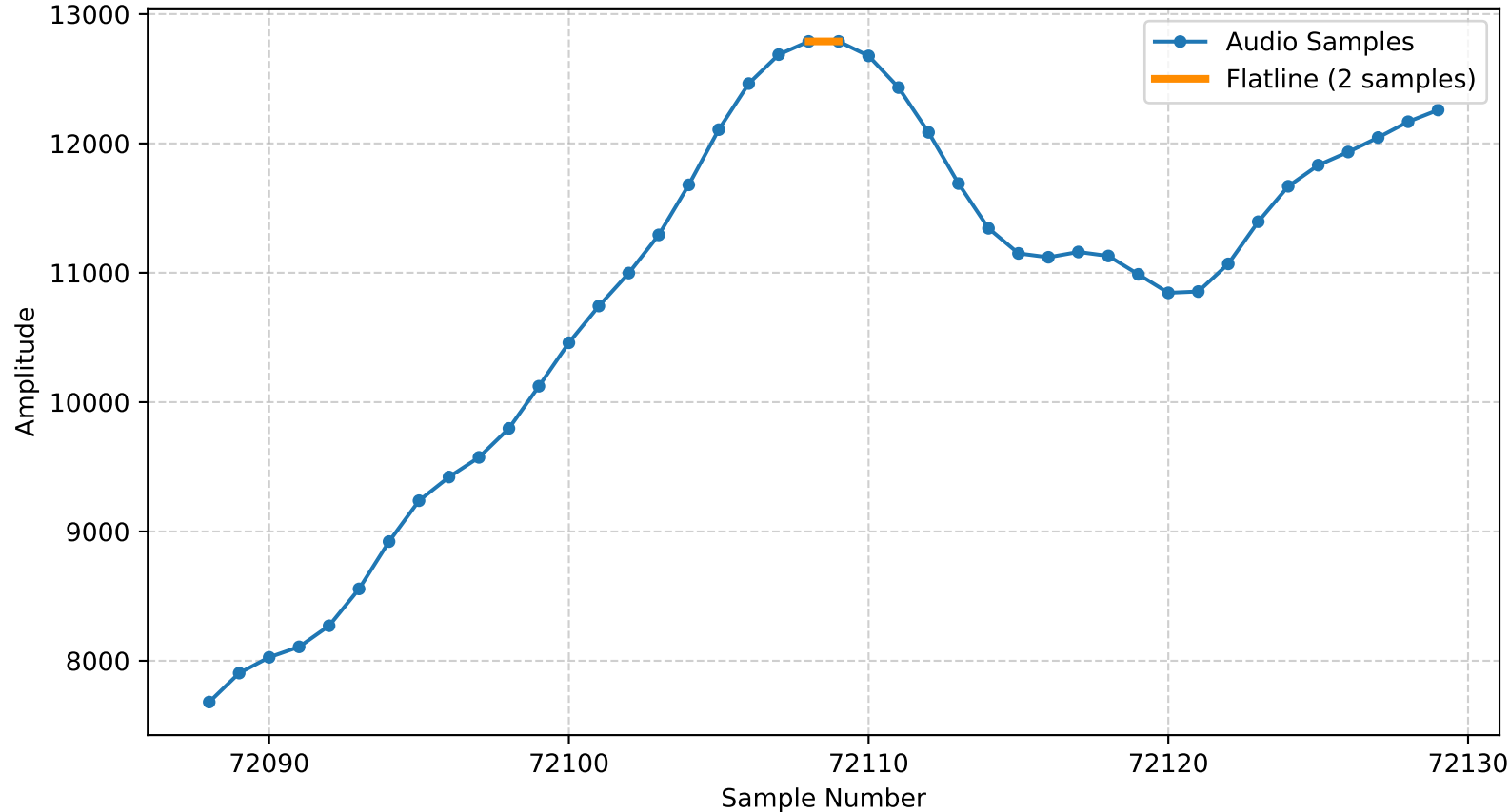
Flatline (2 samples) at Sample 72108 | Channel 0 | Sample Value: 12789.00
