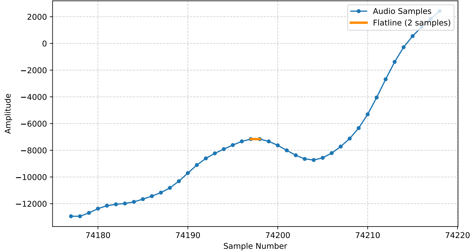
Flatline (2 samples) at Sample 74197 | Channel 1 | Sample Value: -7162.00
