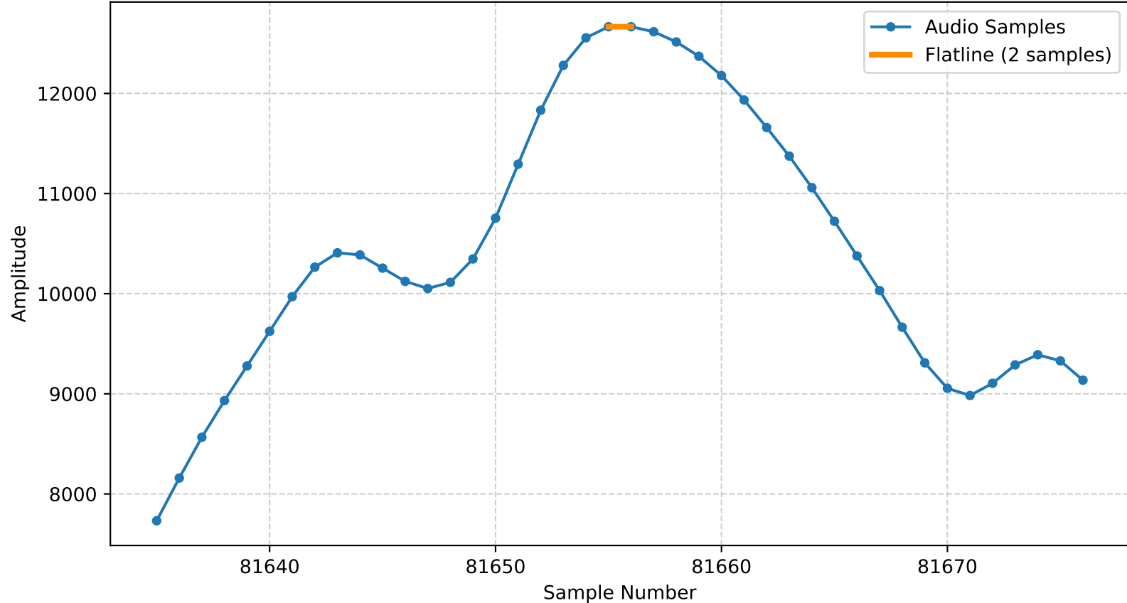
Flatline (2 samples) at Sample 81655 | Channel 1 | Sample Value: 12666.00
