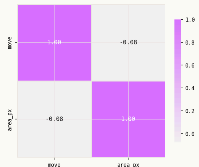
Correlation Matrix
