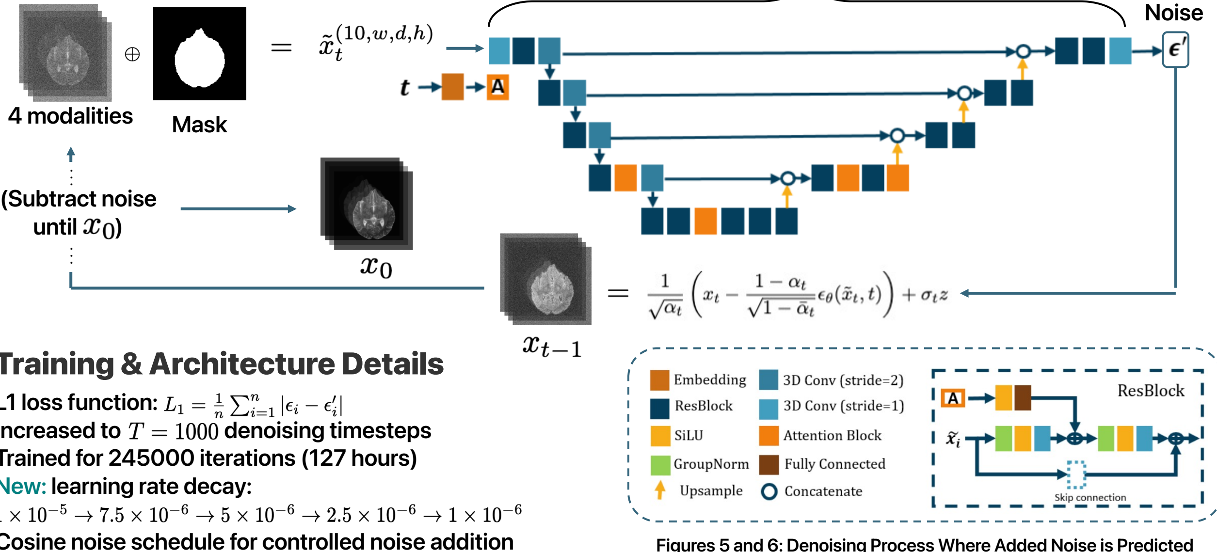
Figures 5 and 6: Denoising Process Where Added Noise is Predicted by a 3D U-Net. U-Net Architecture Originally Displayed in [4].
