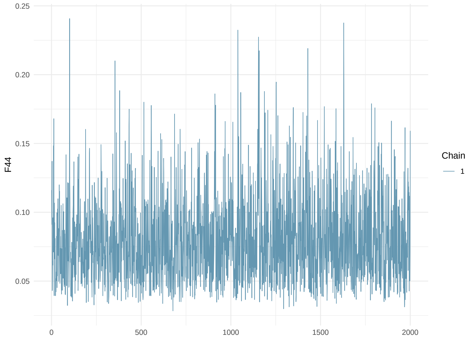
Trace Plot: F44
