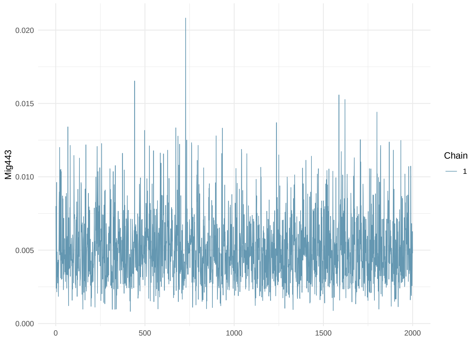
Trace Plot: Mig443
