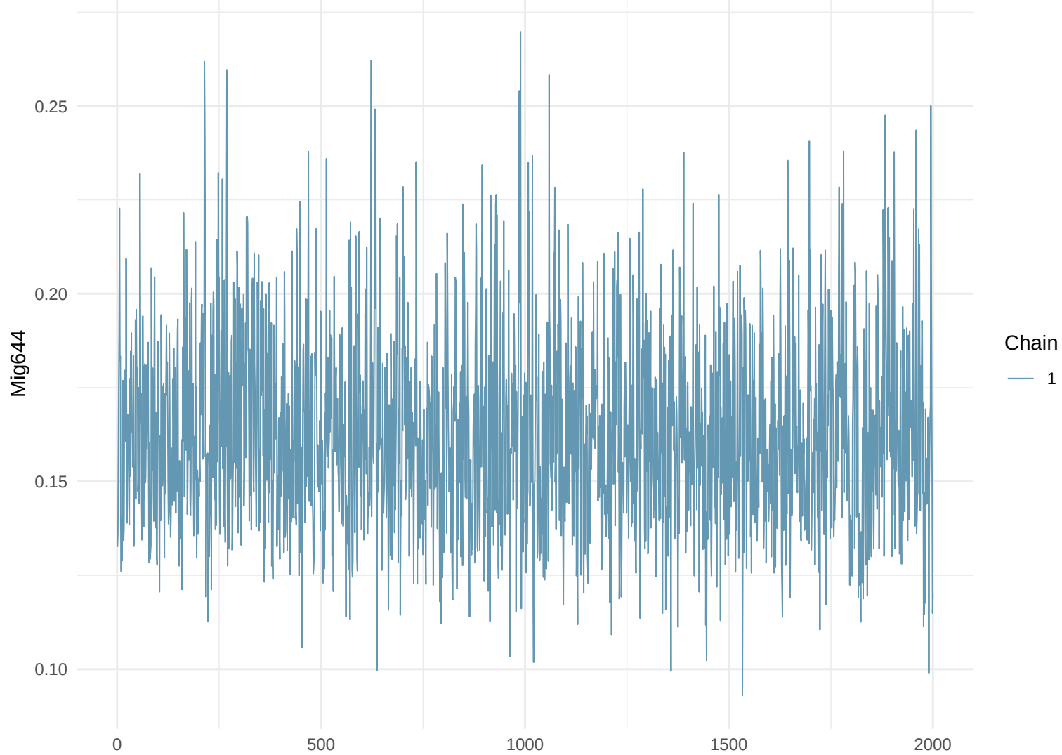
Trace Plot: Mig644
