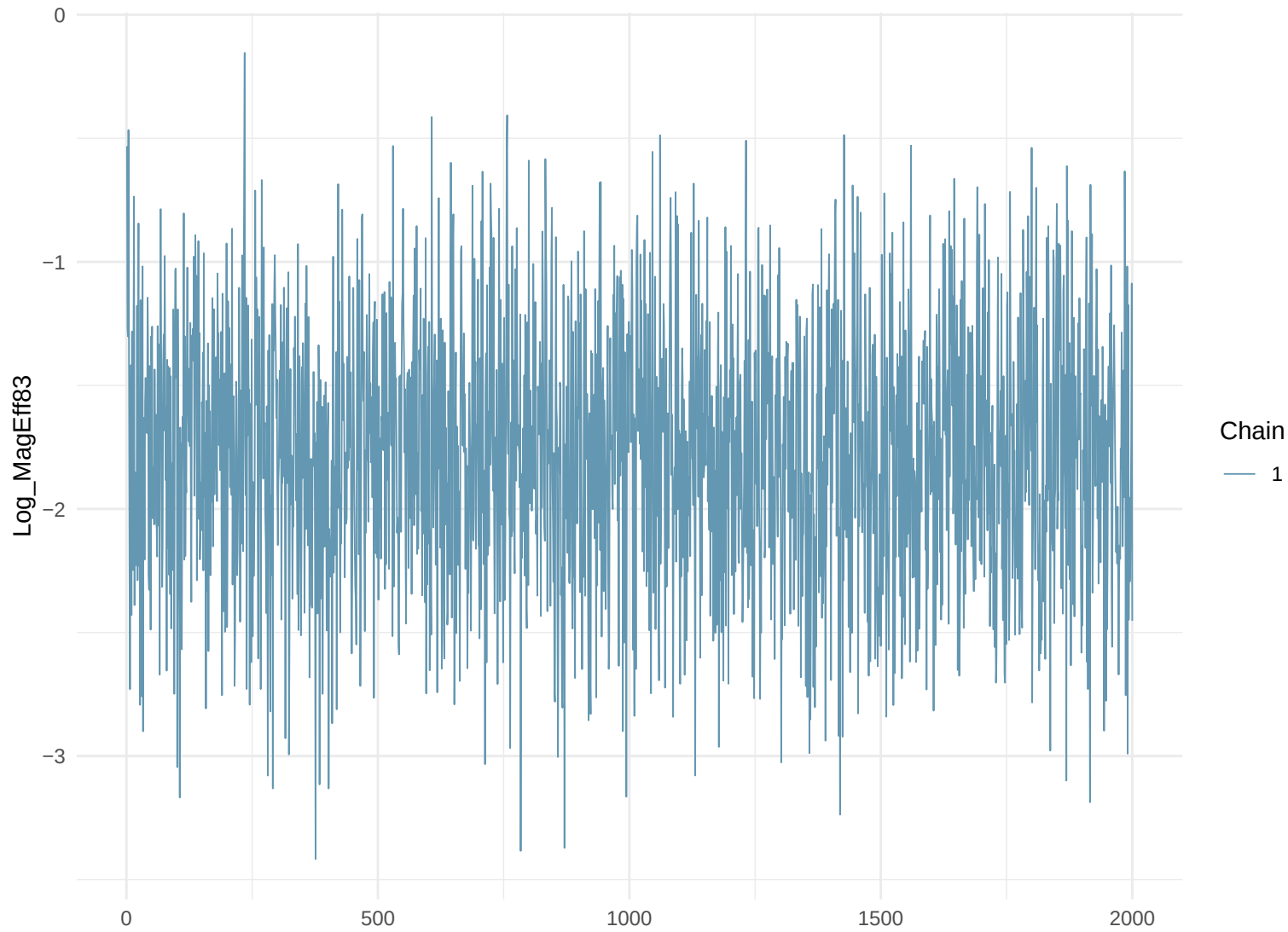
Trace Plot: Log_MagEff83
