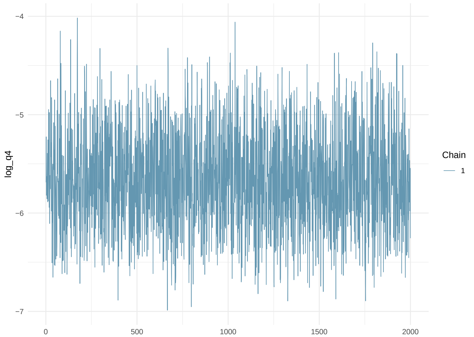
Trace Plot: log q 4
