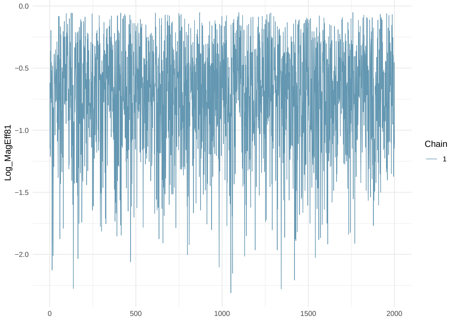
Trace Plot: Log_MagEff81
